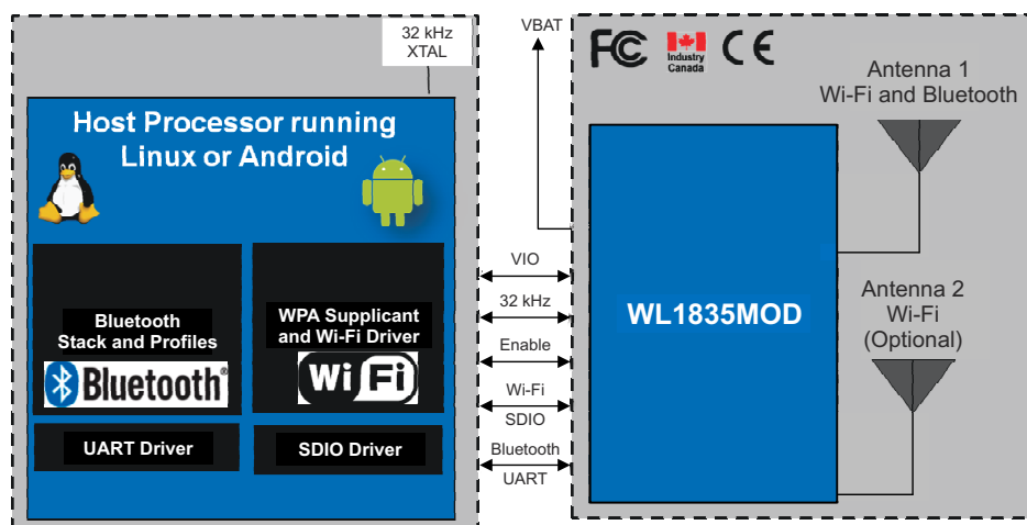
Figure 8-1. WL1835MOD High-Level System Diagram
