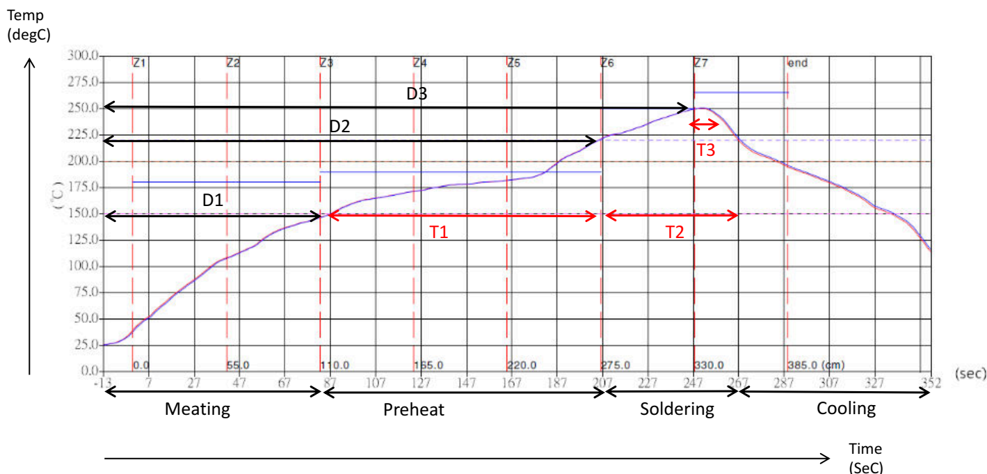
Figure 9-6. Reflow Profile for the WiLink 8 Module
