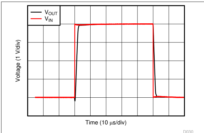
Figure 5-25. Large-Signal Step Response
