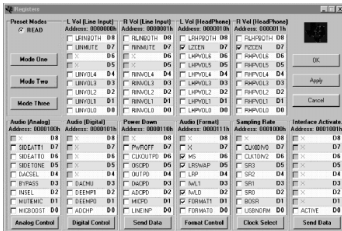
Figure 4–4. Register GUI
