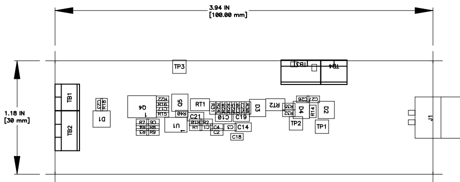
Figure 2. Top Assembly
