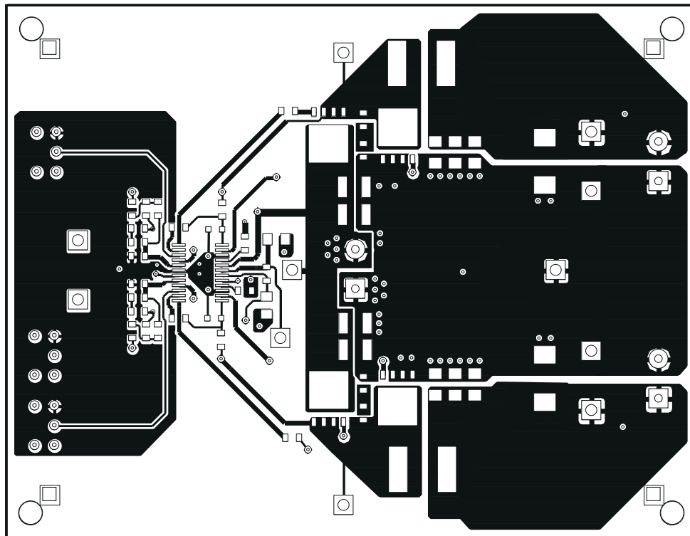
Figure 8-3. Top Layer
