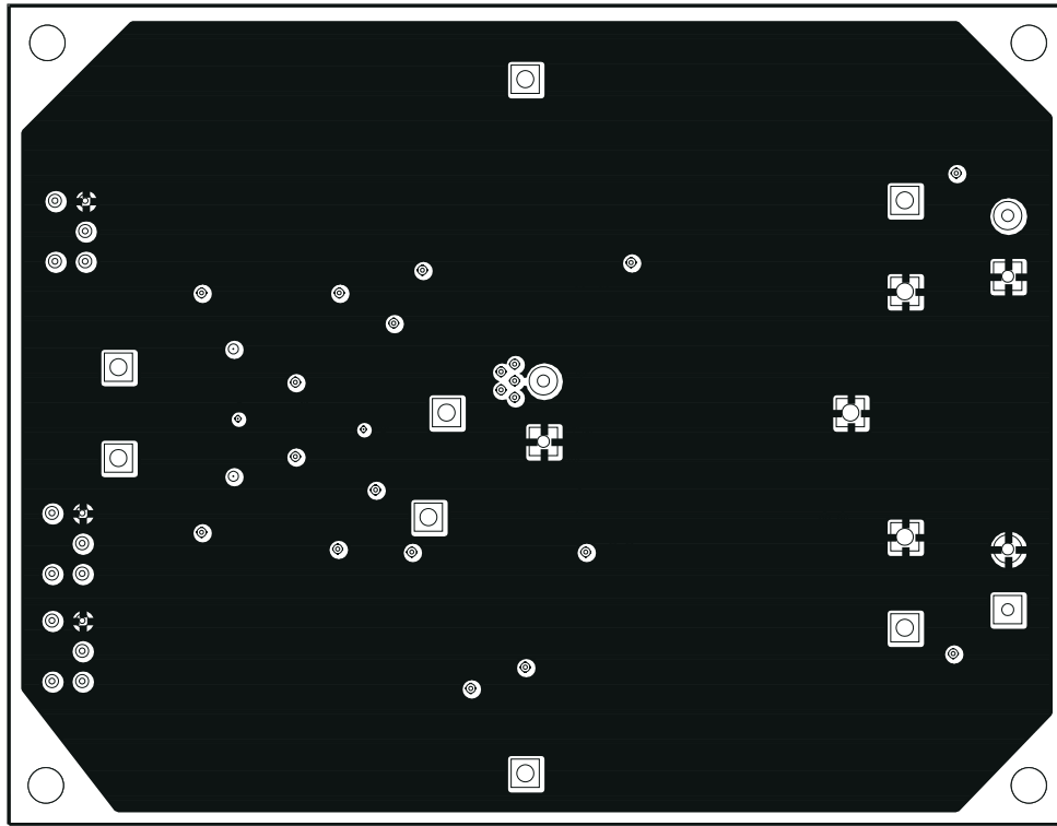
Figure 8-6. Internal Layer 2
