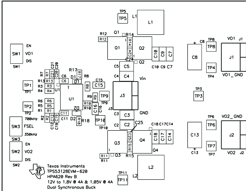
Figure 8-1. Top Assembly
