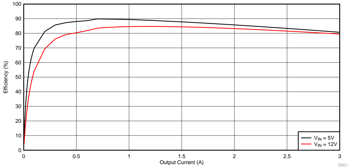
Figure 1. TPS563219EVM-663 Efficiency
