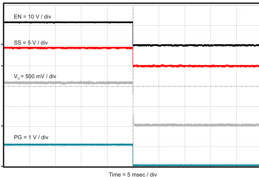
Figure 12. TPS563219EVM-663 Shut-Down Relative to EN
