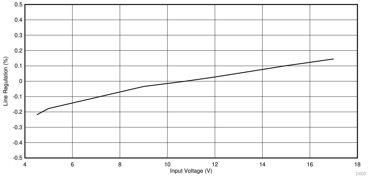
Figure 4-5. TPS563210EVM-663 Line Regulation
