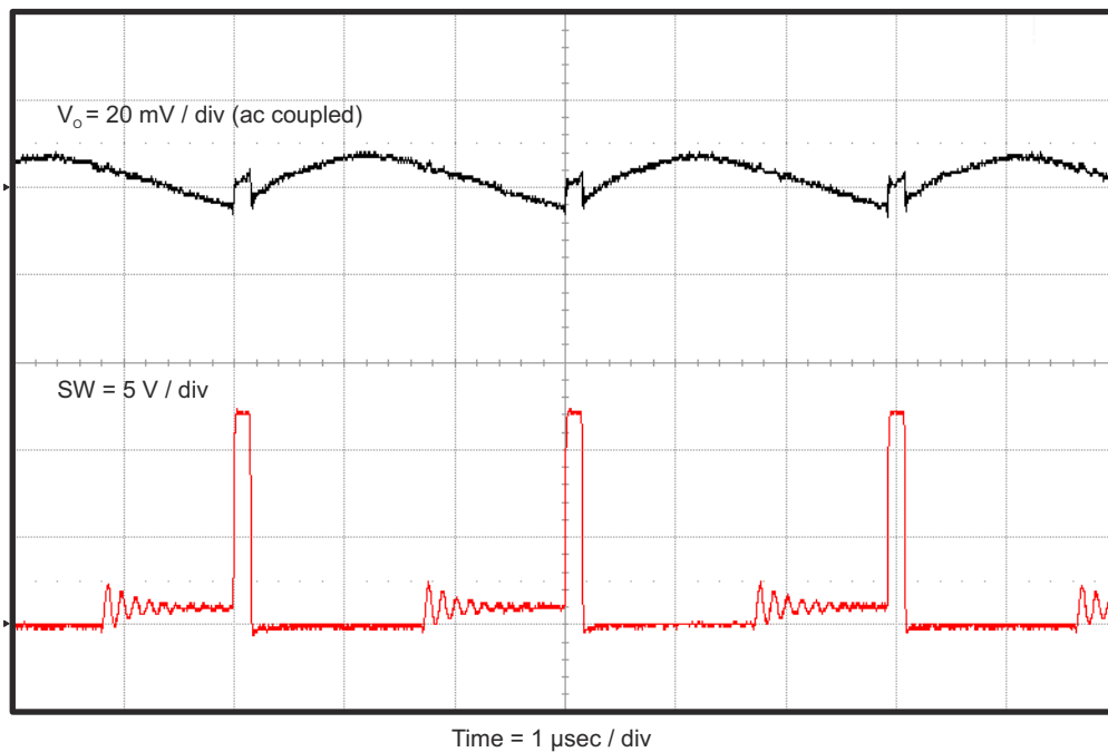
Figure 4-8. TPS563210EVM-663 Output Voltage Ripple, I_{OUT} = 300 \text{ mA}
