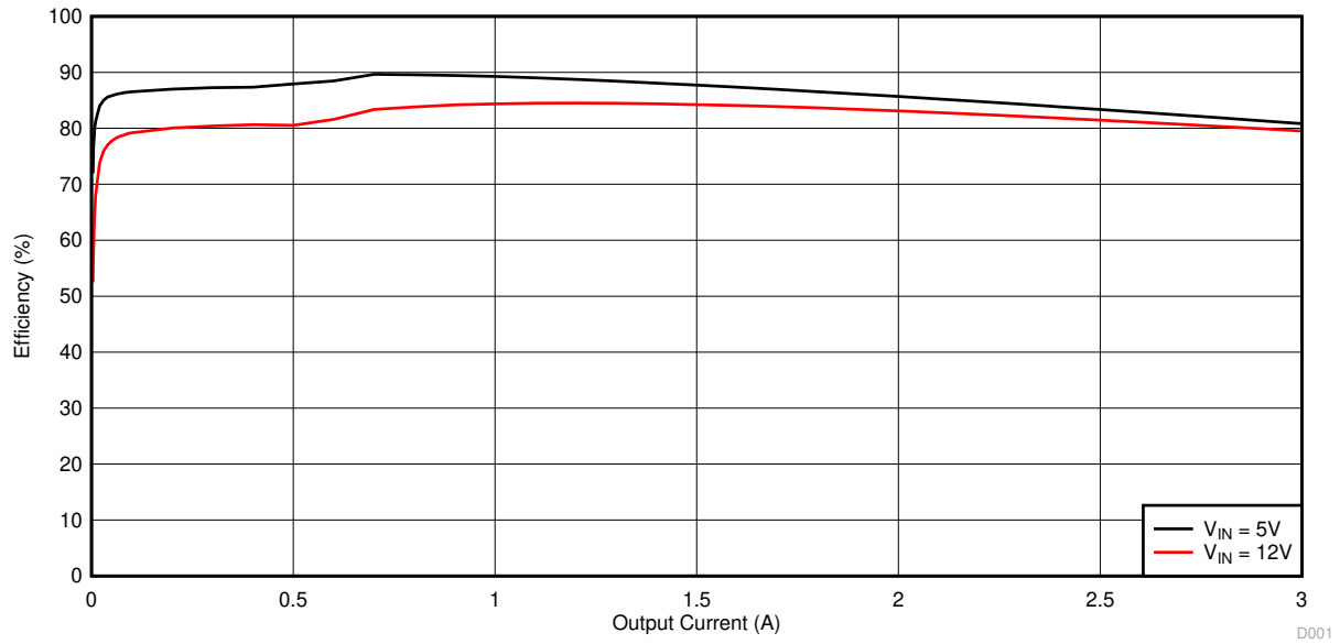
Figure 4-1. TPS563210EVM-663 Efficiency
