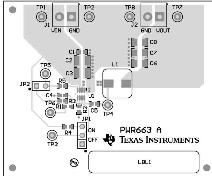
Figure 5-1. Top Assembly
