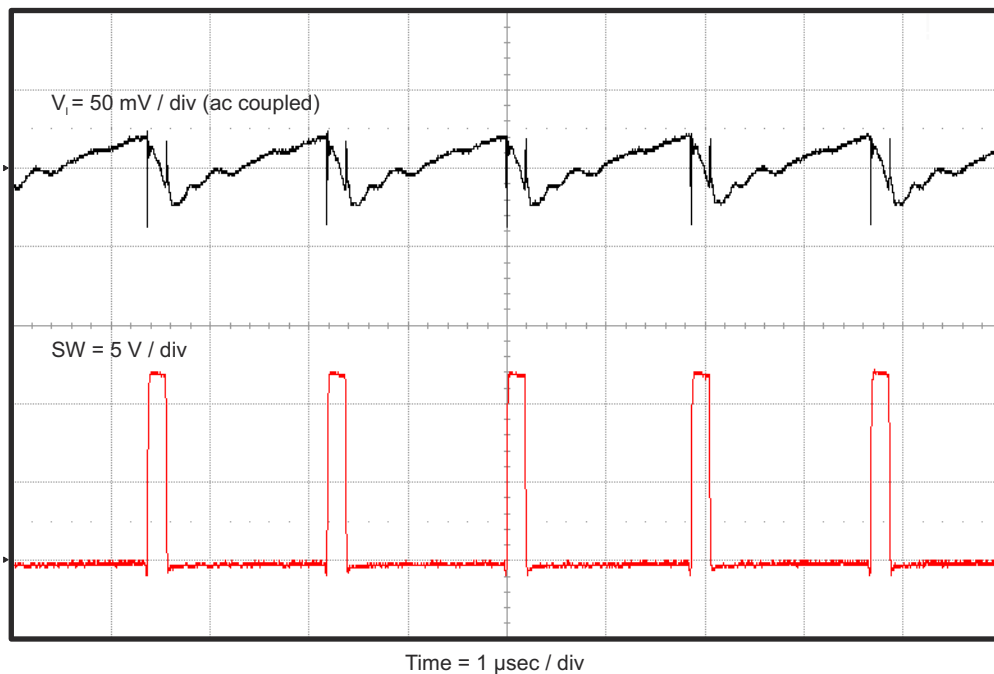
Figure 4-10. TPS563210EVM-663 Input Voltage Ripple, I_{OUT} = 3 \text{ A}
