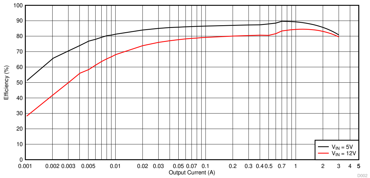
Figure 4-2. TPS563210EVM-663 Light Load Efficiency
