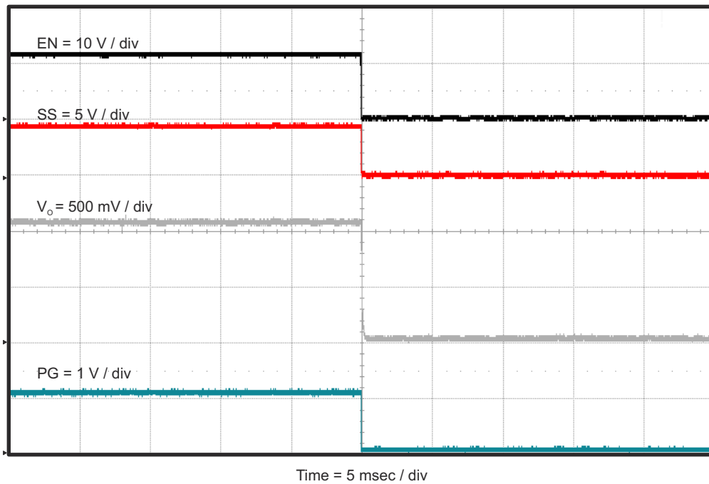
Figure 4-14. TPS563210EVM-663 Shut-Down Relative to EN
