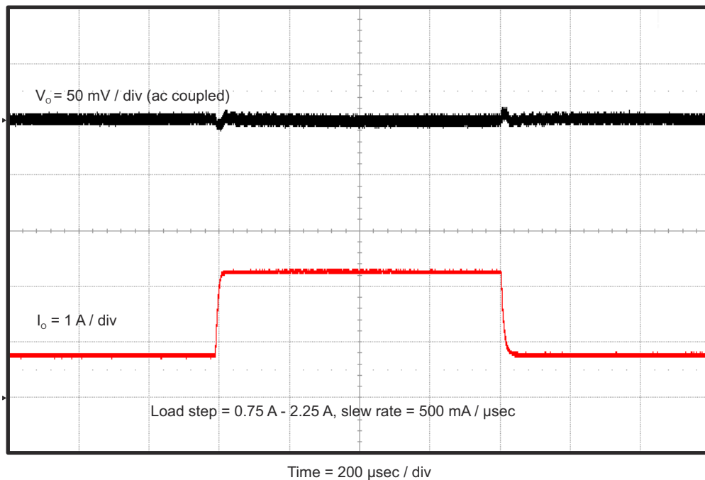
Figure 4-6. TPS563210EVM-663 Load Transient Response, 25% to 75% Load Step
