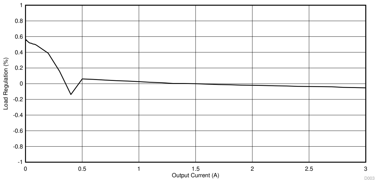
Figure 4-3. TPS563210EVM-663 Load Regulation, 5 V Input
