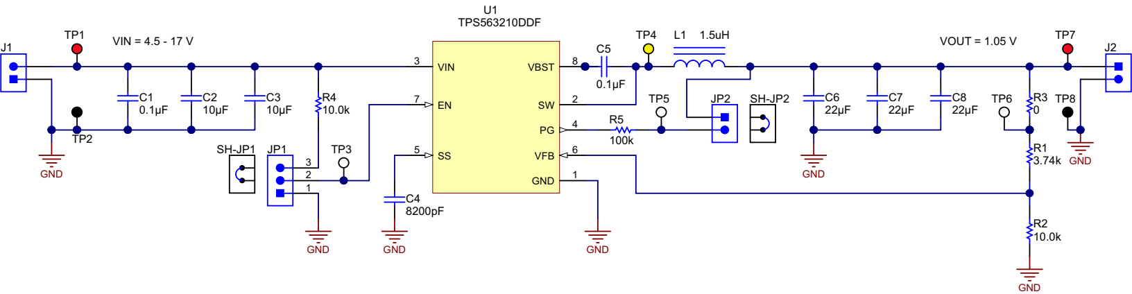
Figure 6-1. TPS563210EVM-663 Schematic Diagram
