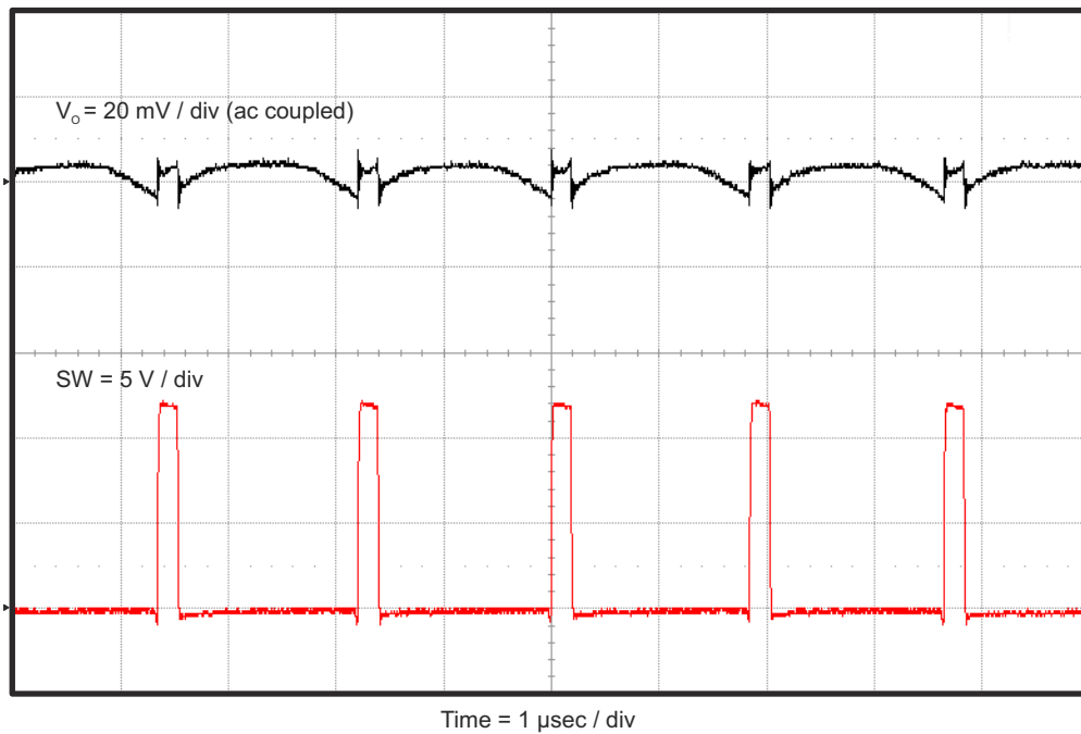
Figure 4-7. TPS563210EVM-663 Output Voltage Ripple, I_{OUT} = 3 \text{ A}
