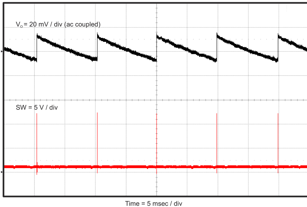
Figure 4-9. TPS563210EVM-663 Output Voltage Ripple, I_{OUT} = 0 \text{ mA}
