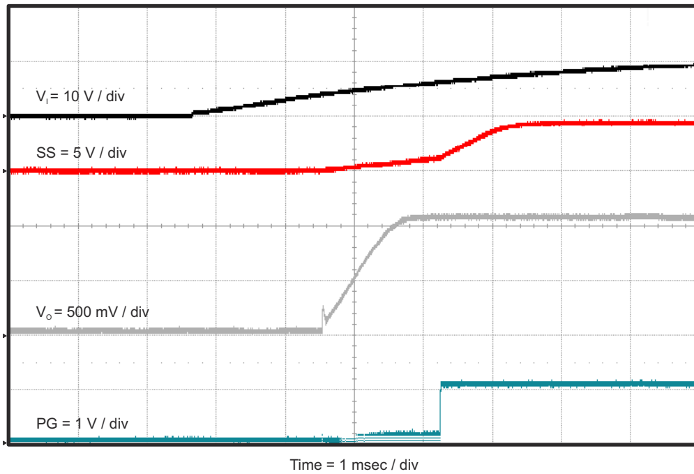
Figure 4-11. TPS563210EVM-663 Start-Up Relative to V_{IN}
