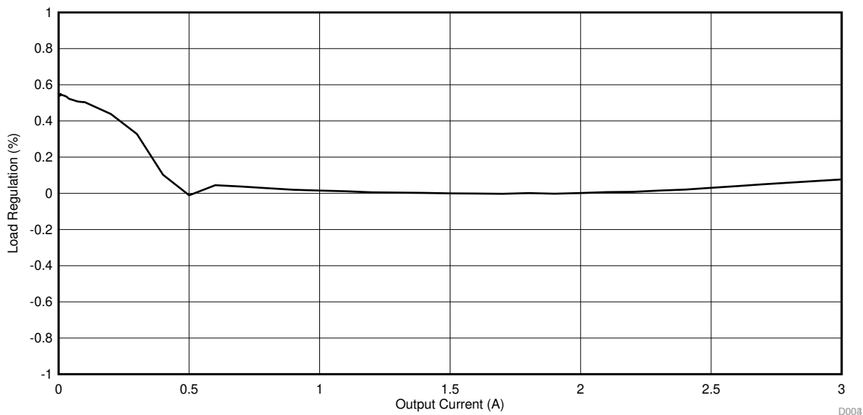
Figure 4-4. TPS563210EVM-663 Load Regulation, 12 V Input
