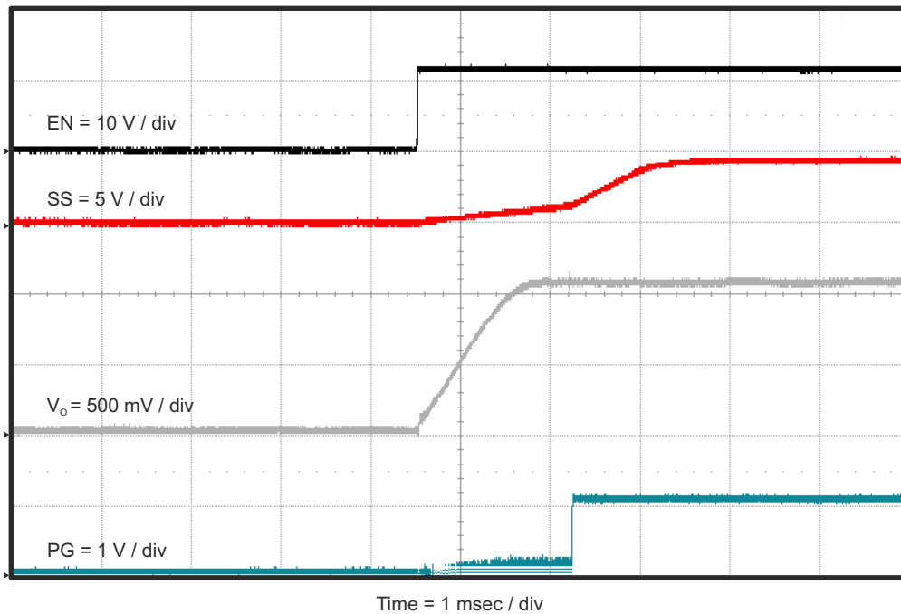
Figure 4-12. TPS563210EVM-663 Start-Up Relative to EN
