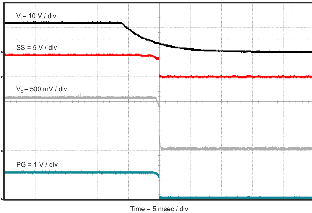
Figure 4-13. TPS563210EVM-663 Shut-Down Relative to V_{IN}
