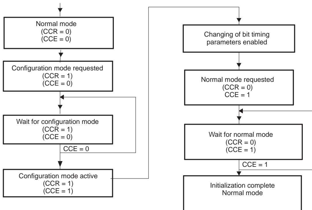
Figure 3-1. Initialization Sequence
