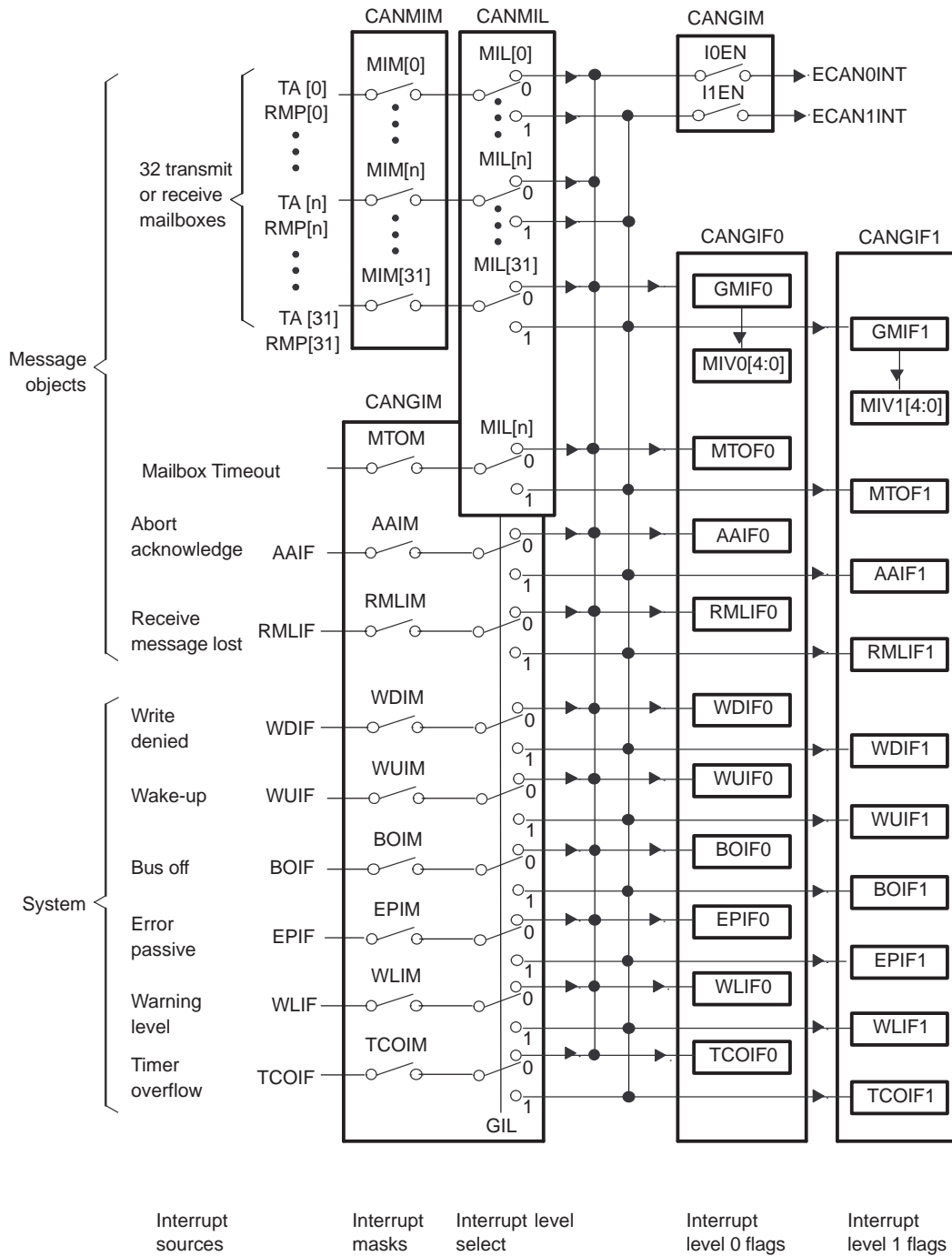
Figure 3-3. Interrupts Scheme
