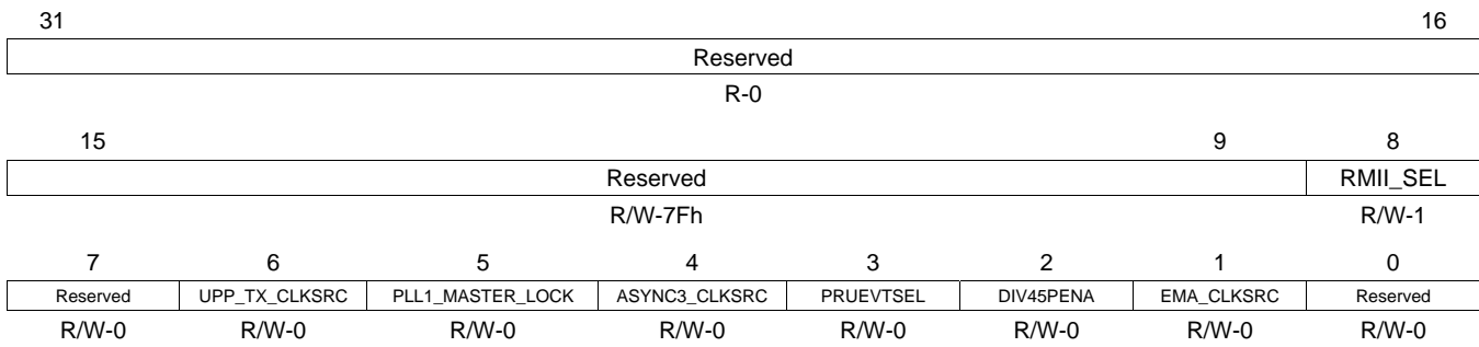
Figure 10-43. Chip Configuration 3 Register (CFGCHIP3)
