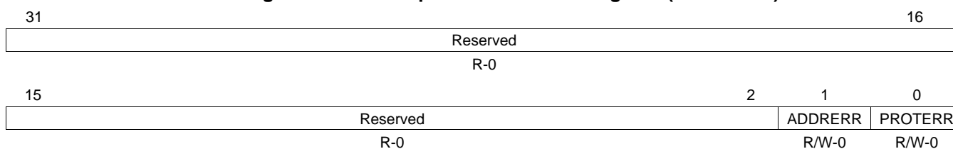
Figure 10-7. Interrupt Raw Status/Set Register (IRAWSTAT)
