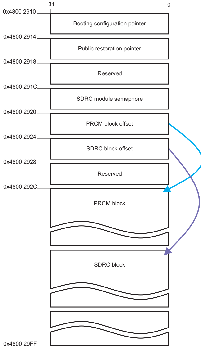
Figure 26-34. CONTROL_SAVE_RESTORE_MEM Format
