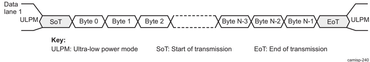
Figure 6-21. Camera ISP CSI2 One Data-Lane Configuration
