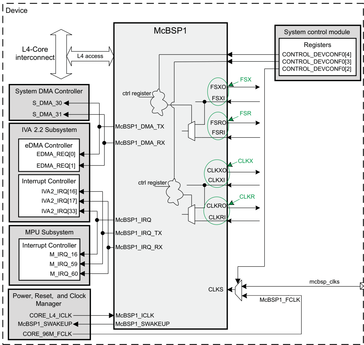
Figure 21-16. McBSP1 Integration
