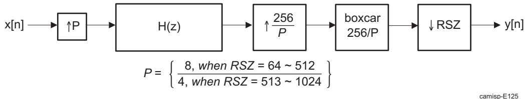
Figure 6-90. Camera ISP VPBE Resizer Approximation Scheme
