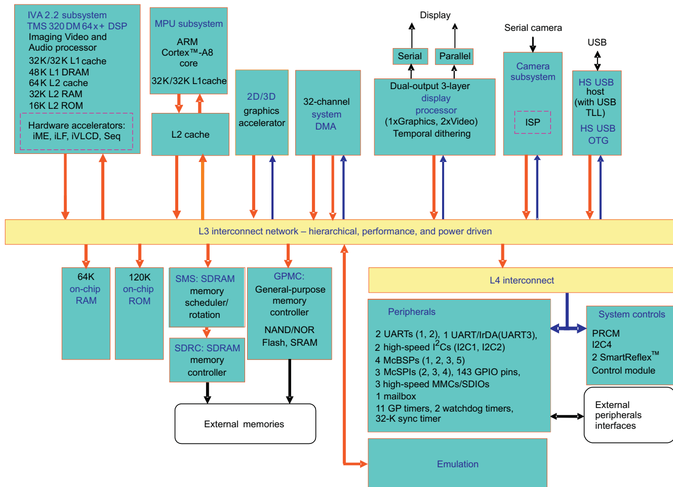
Figure A-1. OMAP36xx in CYN Package Block Diagram
