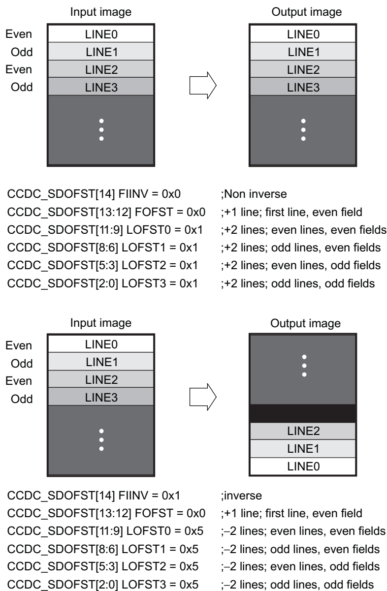
Figure 6-83. Camera ISP CCDC/Line-Output Control: Sample Formats of Input and Output Images
