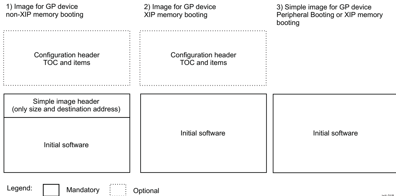
Figure 26-32. Image Format
