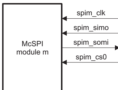
Figure 20-8. McSPI Interface Signals in Slave Mode
