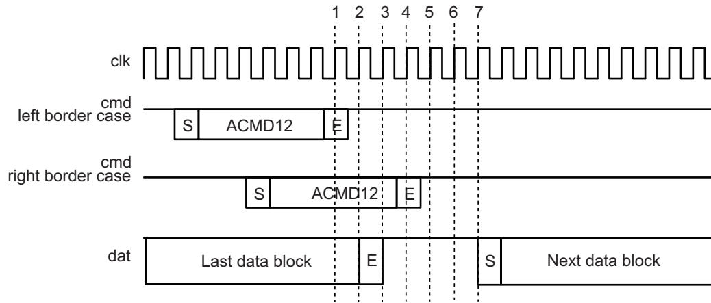
Figure 24-30. Autocommand 12 Timings During Read Transfer
