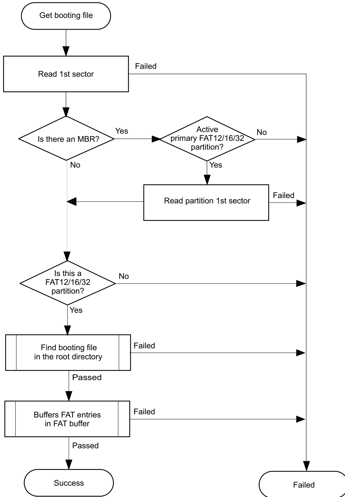
Figure 26-29. SD/MMC Booting
