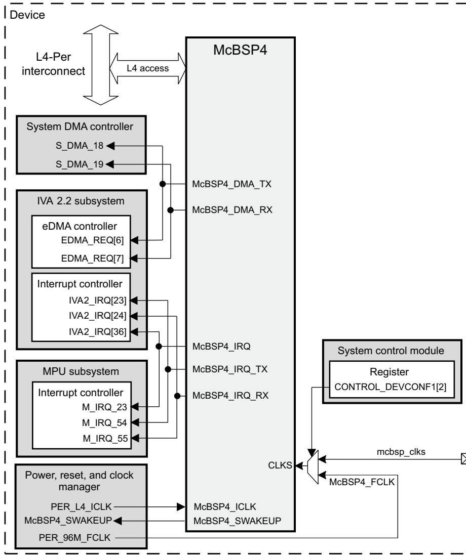
Figure 21-19. McBSP4 Integration
