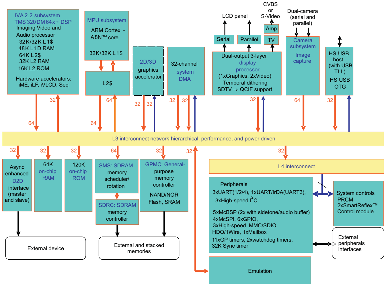
Figure 1-2. OMAP36xx High-Tier Block Diagram
