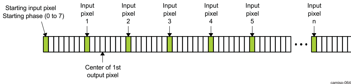
Figure 6-93. Camera ISP VPBE Resizer Pseudo-Code Description of the Resizer Algorithm in the 4-Tap/8-Phase Mode
