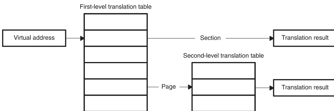
Figure 15-8. Translation Hierarchy
