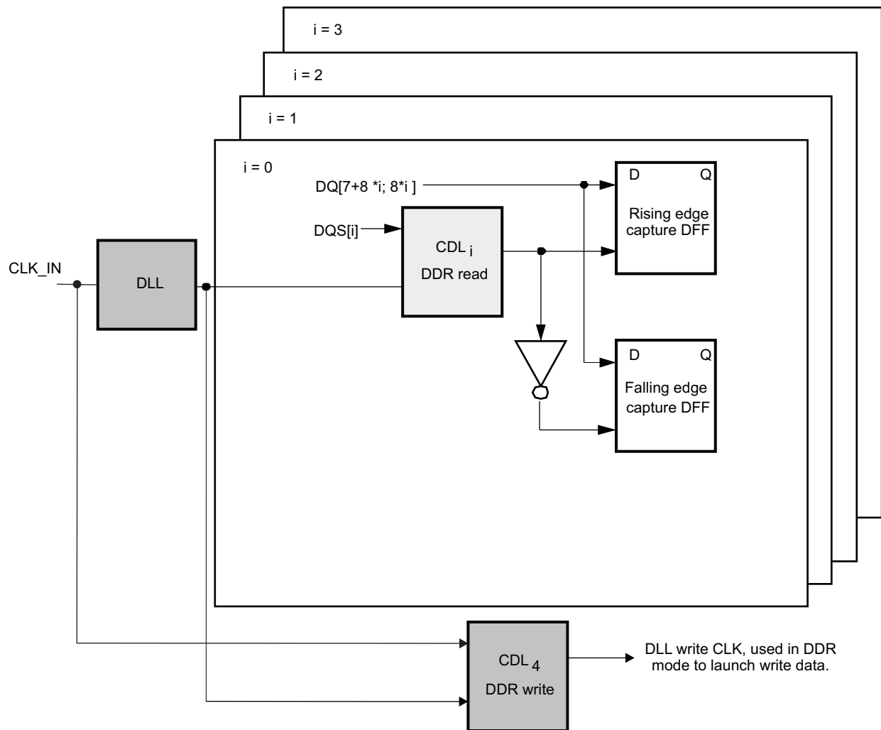
Figure 10-59. DLL/CDL Architecture
