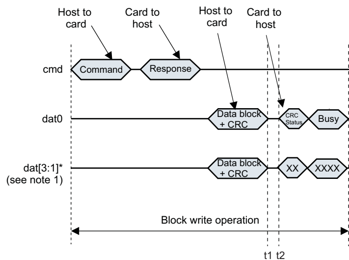
Figure 24-25. Write CRC Status Timeout
