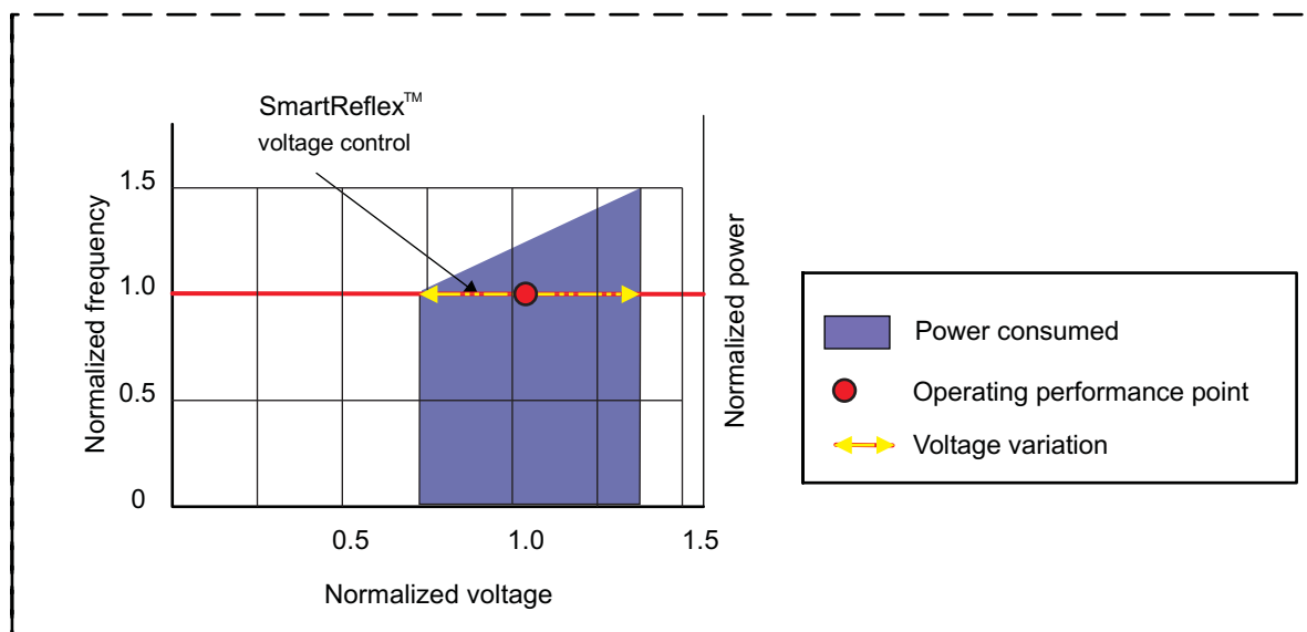
Figure 3-2. SmartReflex Example
