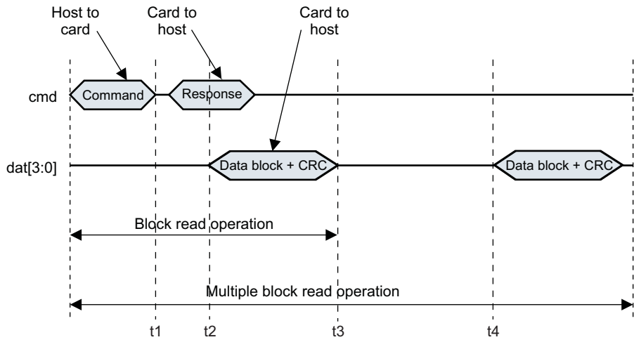
Figure 24-26. Read Data Timeout
