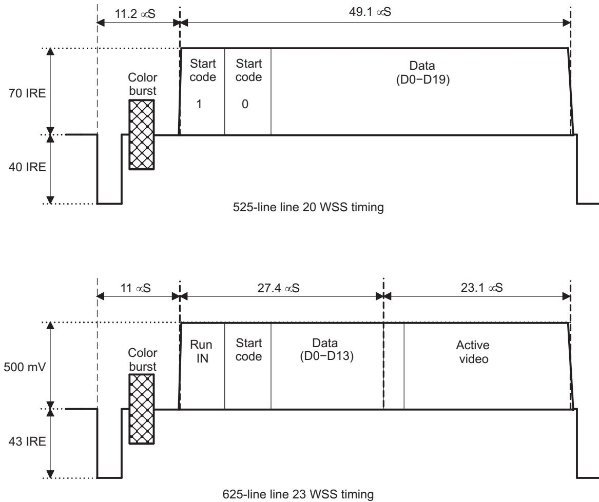
Figure 7-108. WSS Timing
