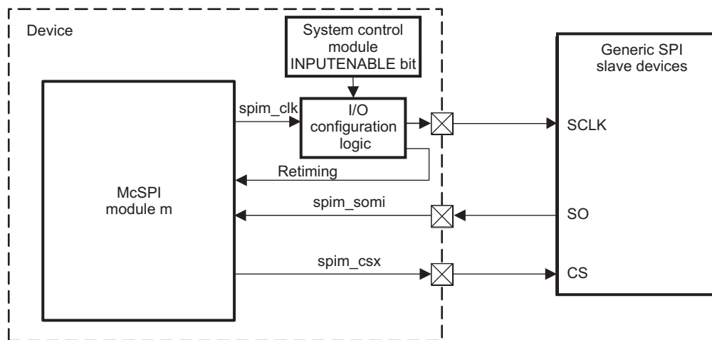
Figure 20-4. McSPI Master Single Mode (Receive-Only)
