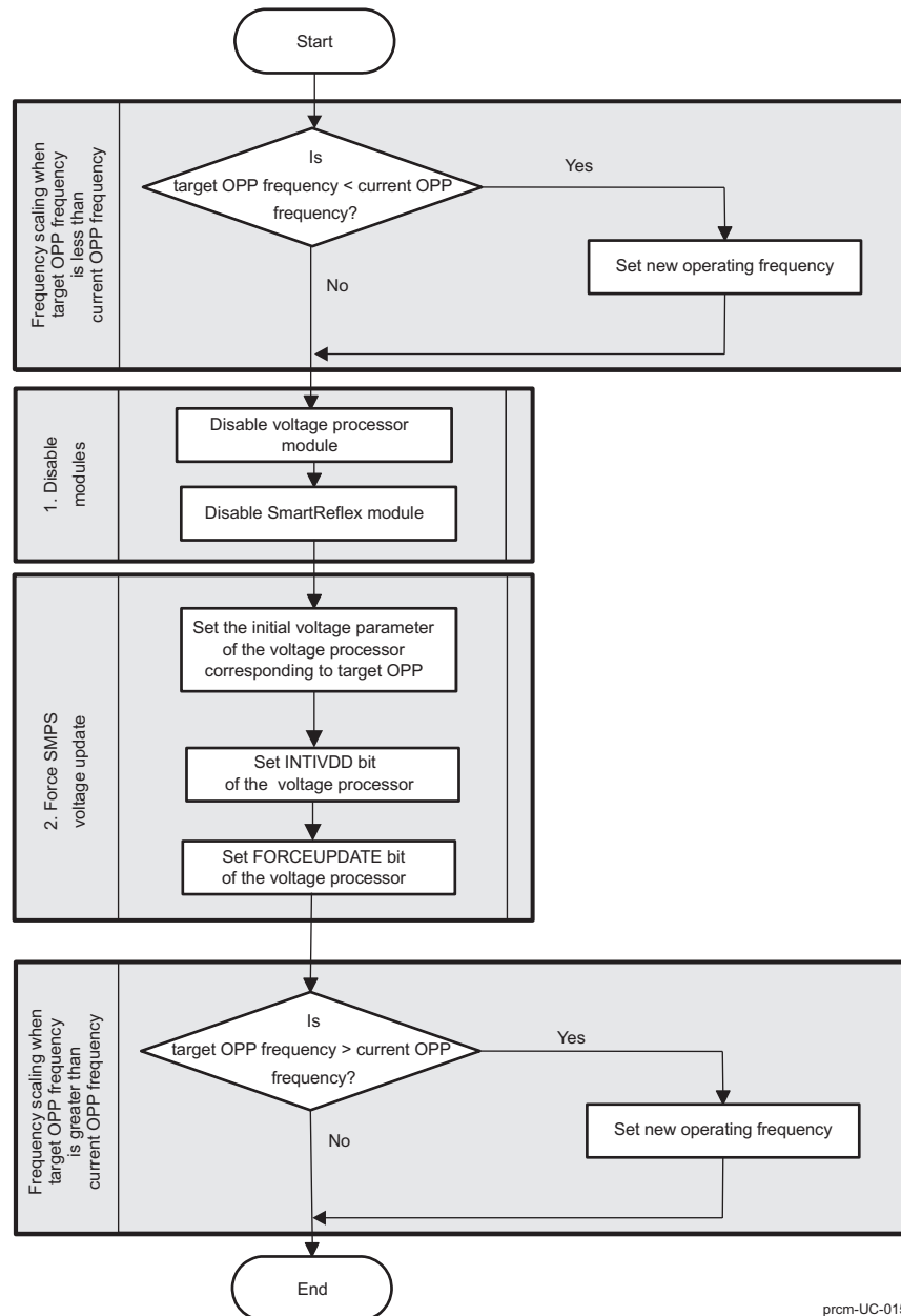
Figure 3-100. Voltage Processor - OPP Change Flow Chart
