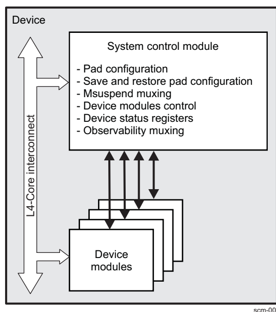
Figure 13-1. SCM Overview
