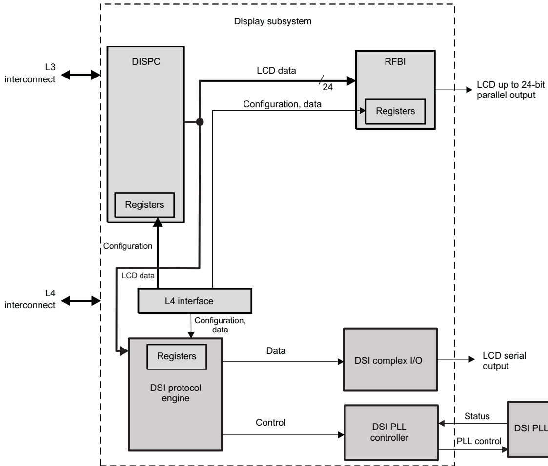
Figure A-4. Display Subsystem Block Diagram
