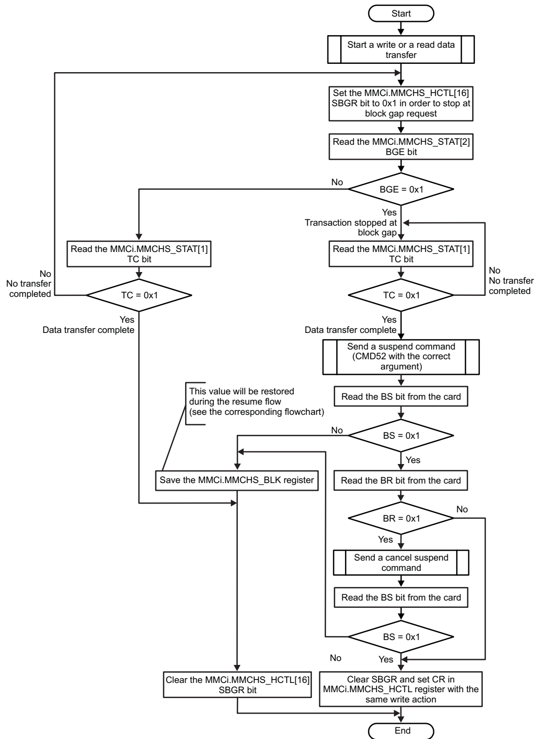
Figure 24-41. MMC/SD/SDIO Controller Suspend Flow
