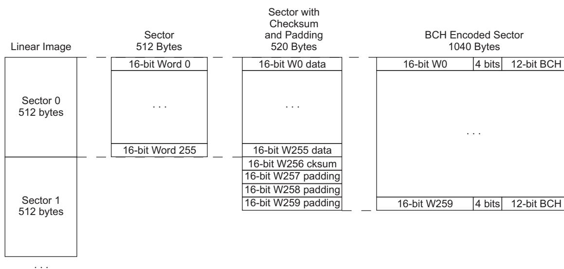
Figure 26-21. MLC NAND Data Encoding
