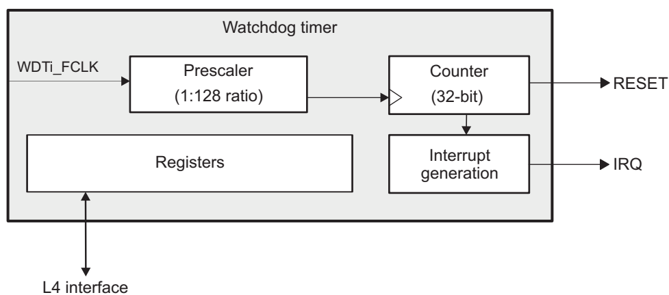
Figure 16-16. 32-Bit WDT Functional Block Diagram
