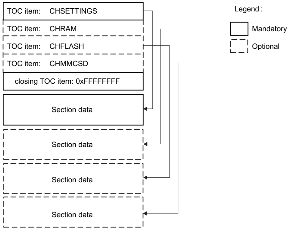
Figure 26-33. CH Format
