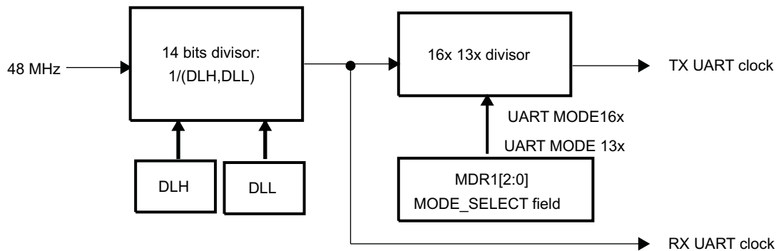
Figure 19-31. Baud Rate Generation
