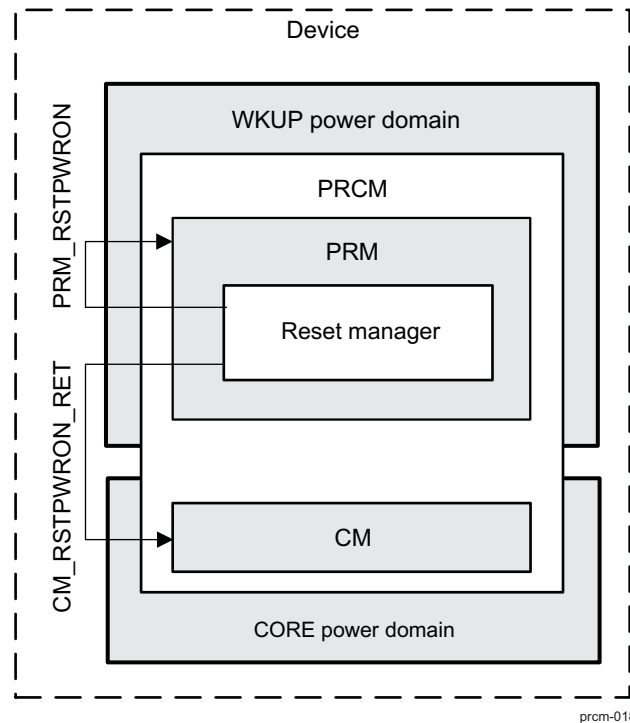
Figure 3-19. PRCM Reset Signals
