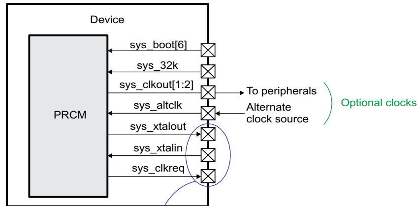
Figure 26-4. Clock Interface
