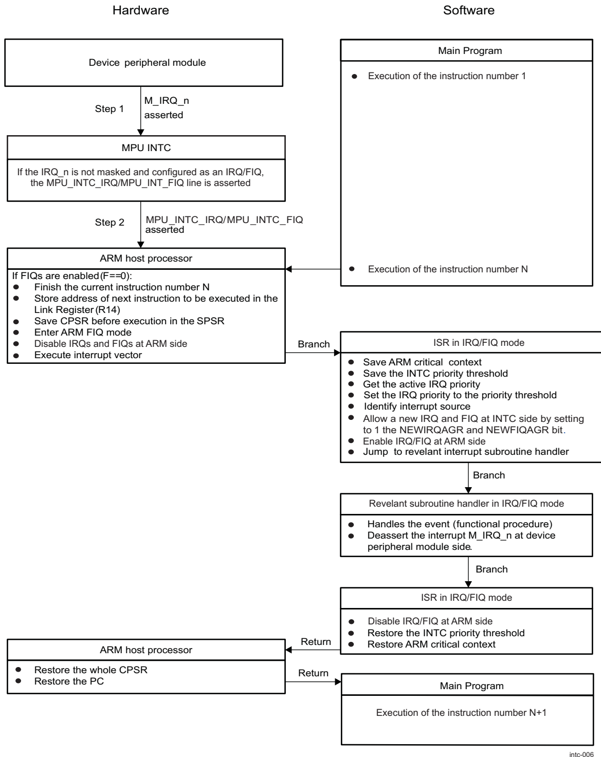
Figure 12-6. Nested IRQ/FIQ Sequence
