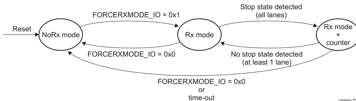
Figure 6-74. Camera ISP CSI2 RxMode and StopState FSM
