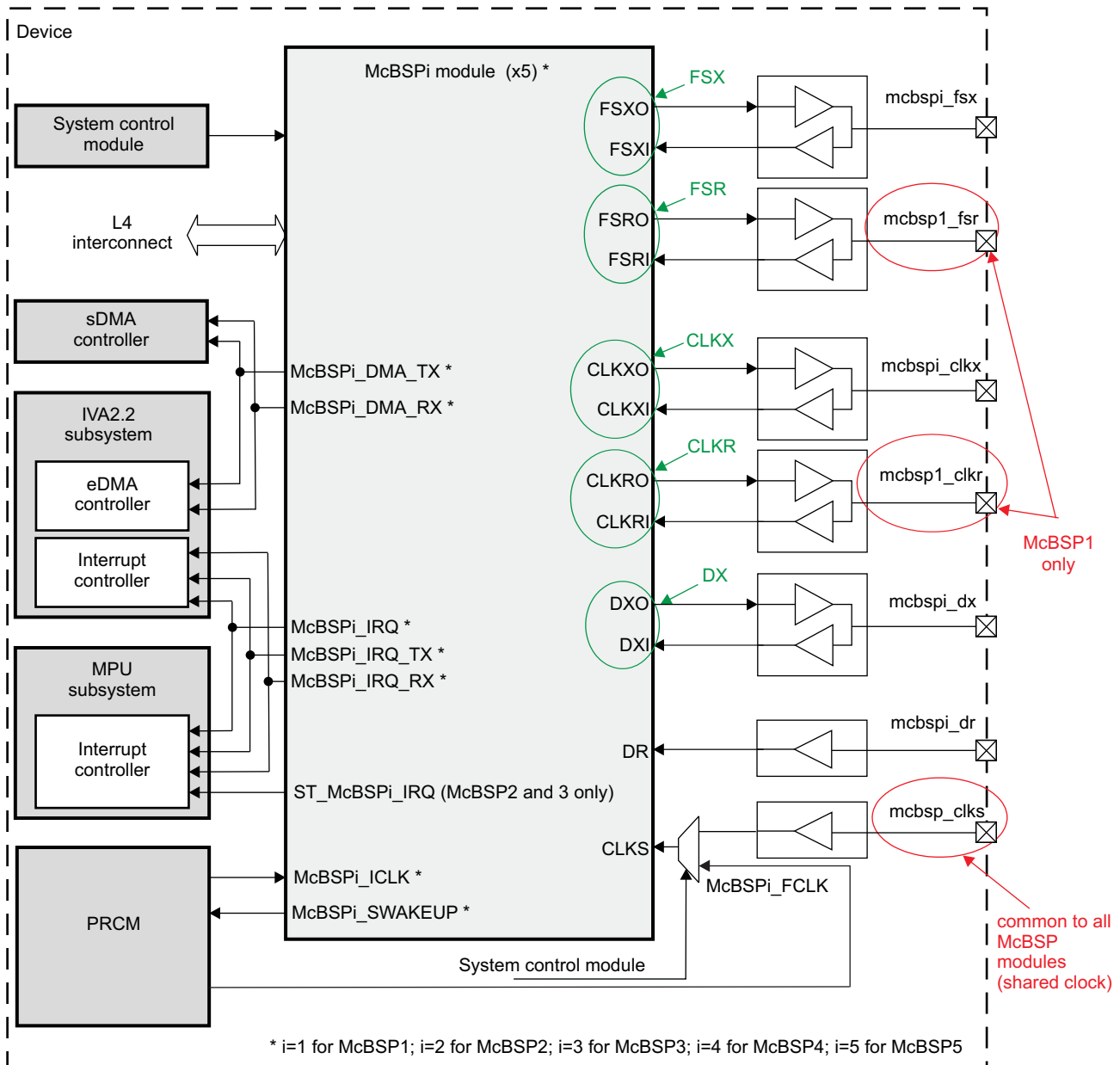
Figure 21-1. McBSP Highlight
