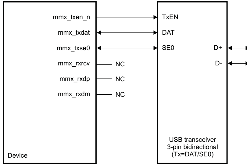
Figure 22-22. 3-Pin Bidirectional Using DAT/SE0 Signaling
