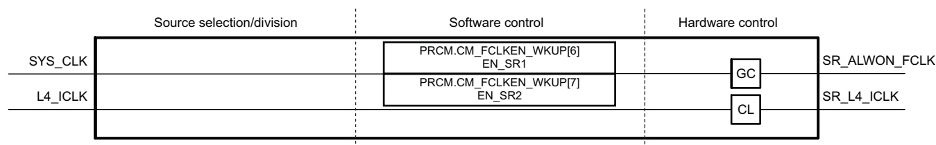
Figure 3-74. SMARTREFLEX Power Domain Clock Controls
