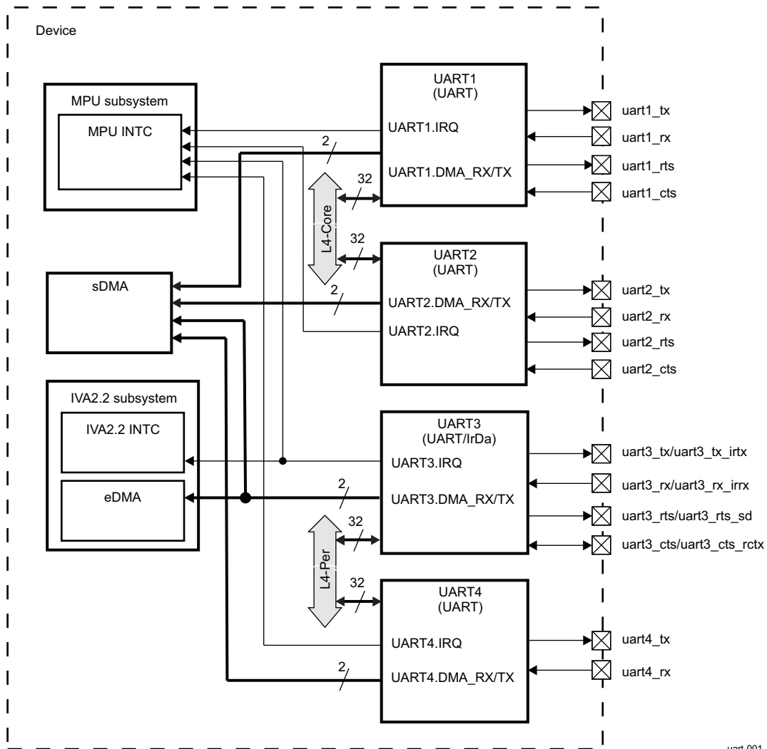
Figure 19-1. UART Module
