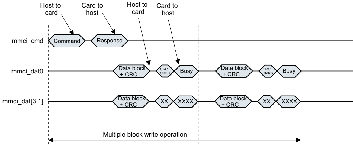
Figure 24-51. Data Write Transfer
