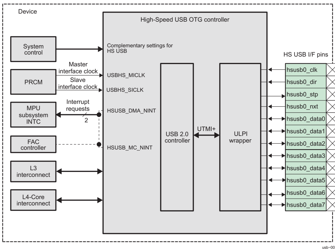
Figure 22-2. High-Speed USB Controller Highlight
