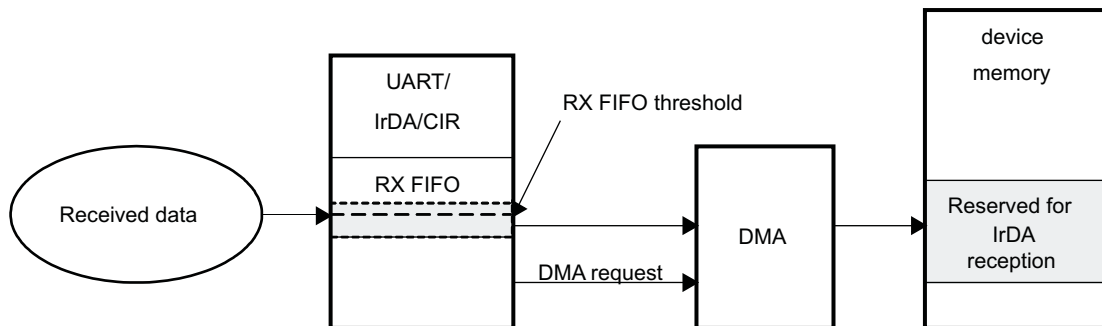
Figure 19-30. Reception Process
