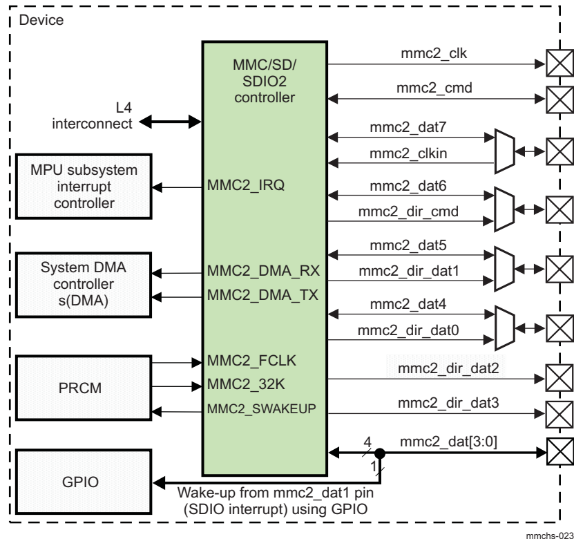
Figure 24-2. MMC/SD/SDIO2 Overview
