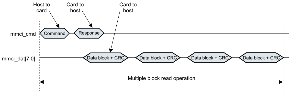
Figure 24-50. Data Read Transfer
