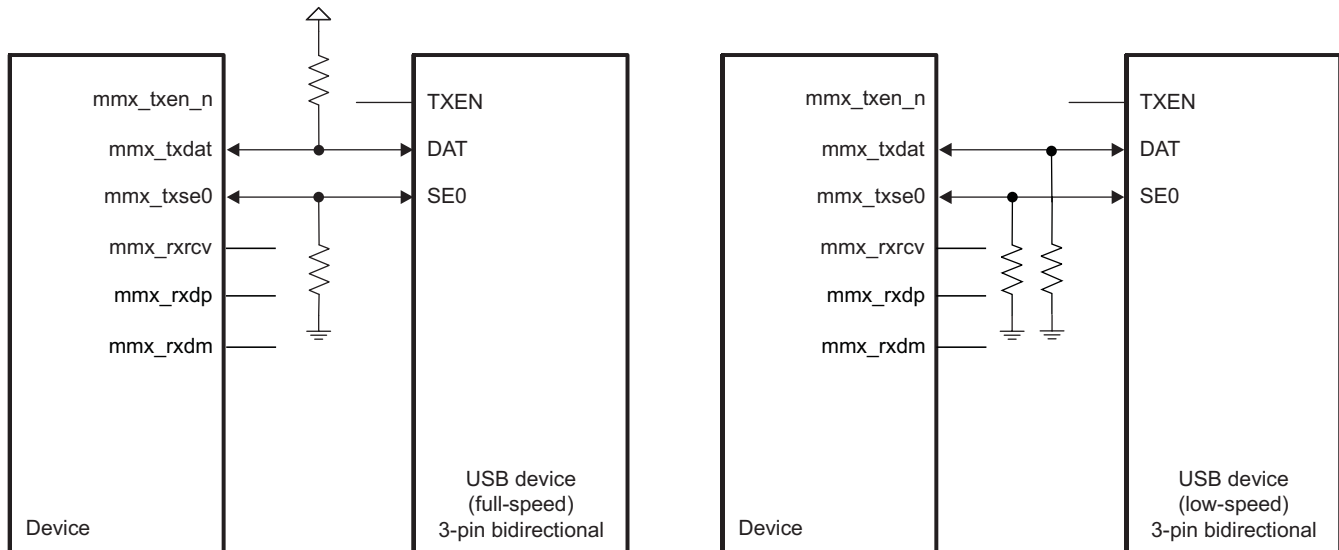
Figure 22-29. 2-Pin Bidirectional TLL Using DAT/SE0 Encoding, With 3-Pin Bidirectional USB Device
