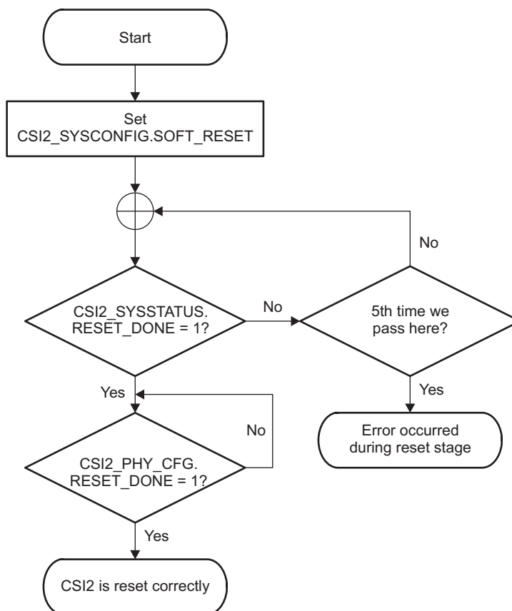
Figure 6-109. Camera ISP CSI2 Receiver Global Reset Flow Chart
