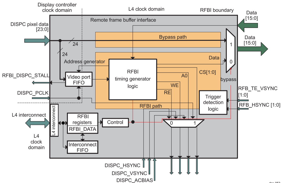
Figure 7-105. RFBF Architecture Overview
