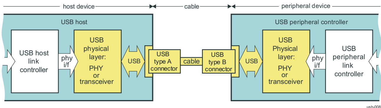
Figure 22-9. USB Connection
