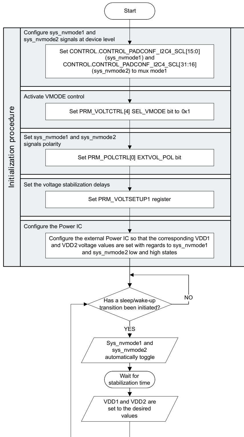
Figure 3-105. Voltage Control Through VMODE Flow Chart
