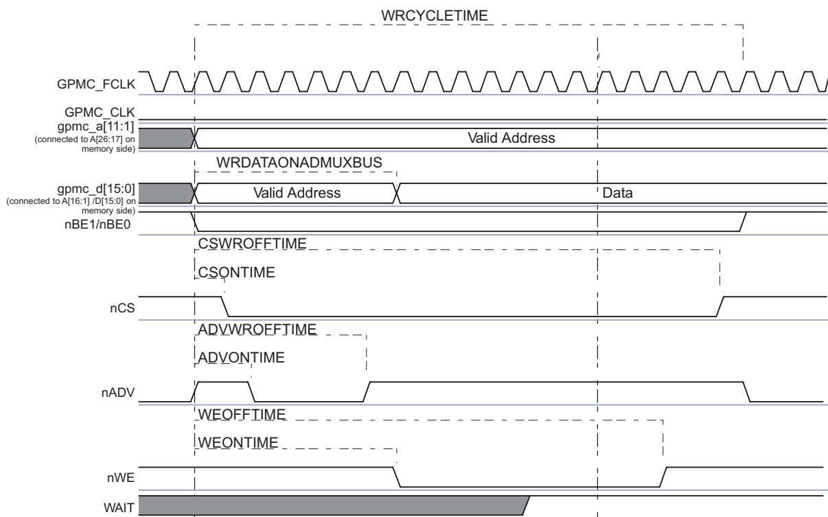
Figure 10-13. Asynchronous Single Write on an Address/Data-Multiplexed Device
