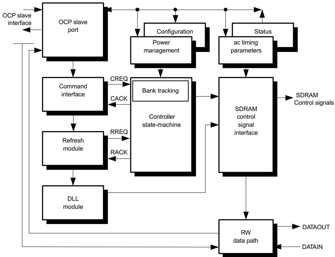
Figure 10-50. SDRC Architecture
