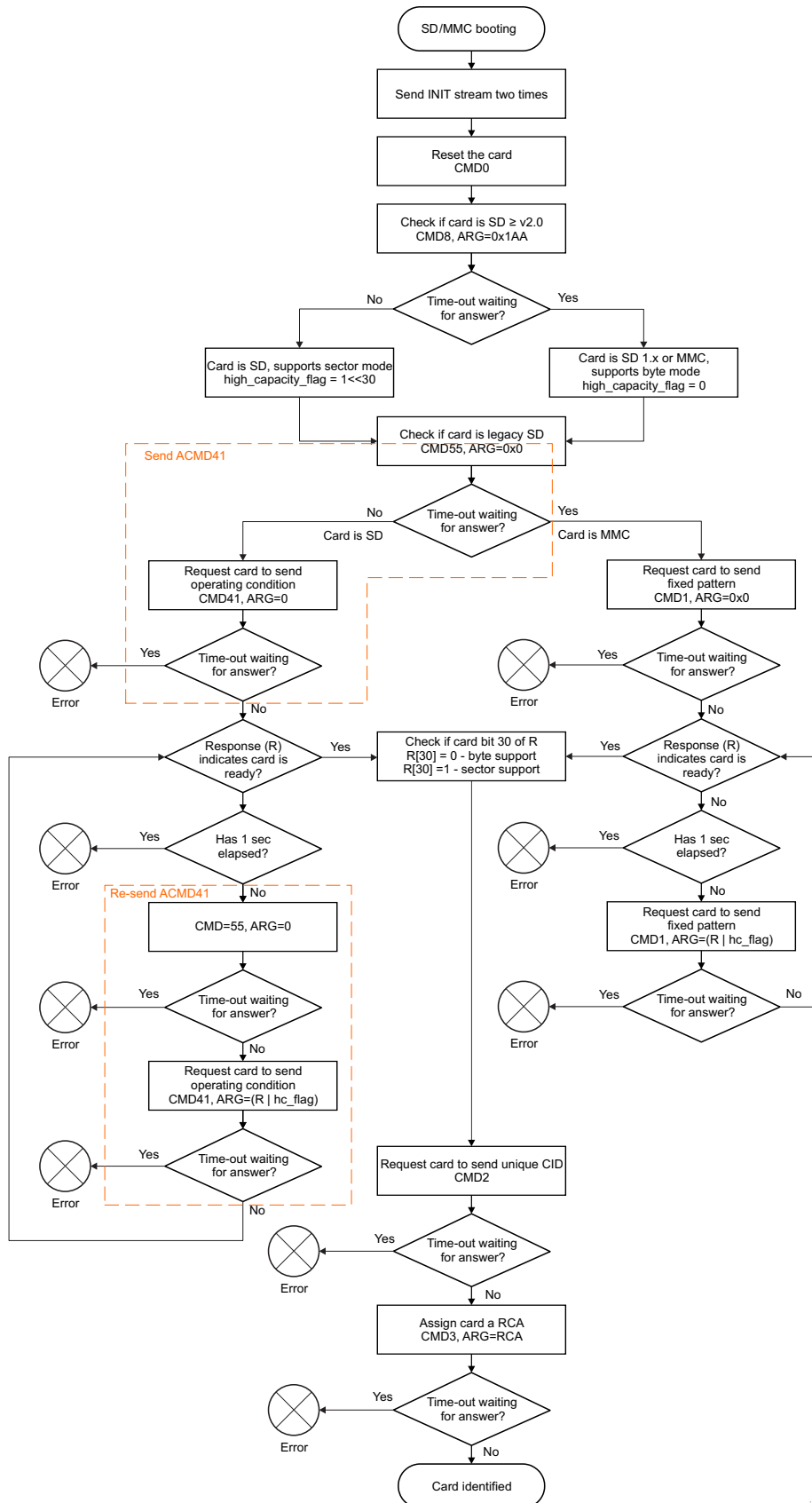
Figure 26-28. MMC/SD Detection Procedure
