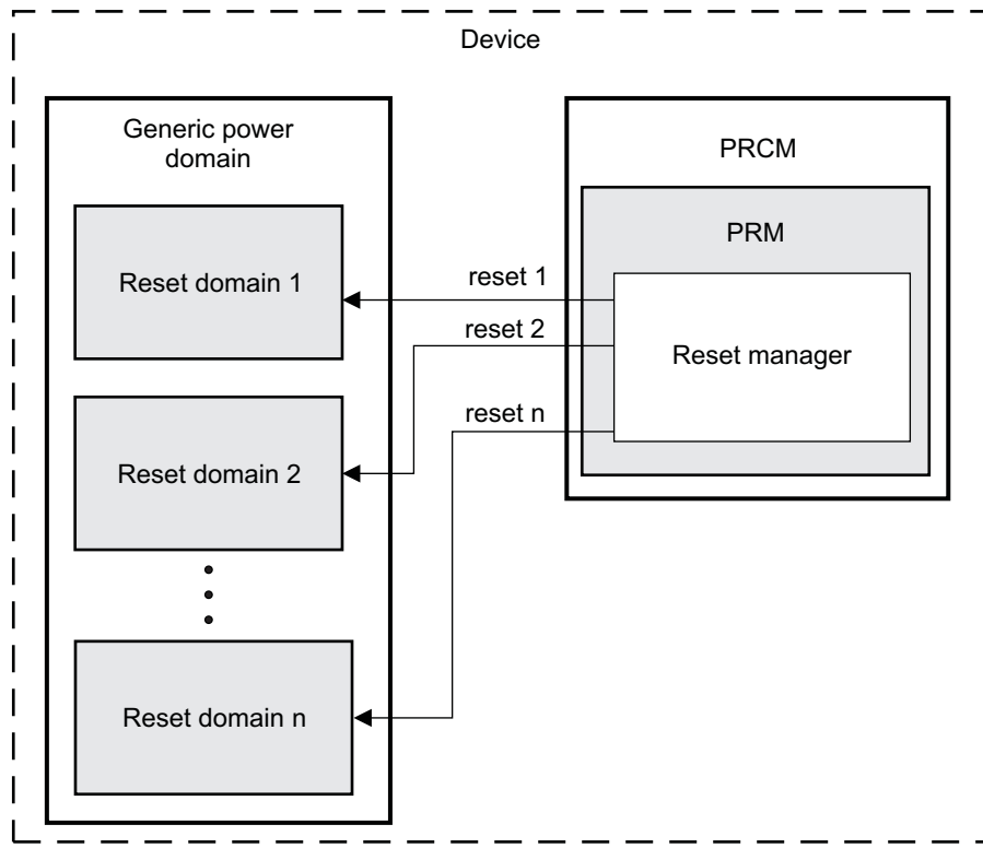
Figure 3-20. Reset Manager Interface With Generic Power Domain
