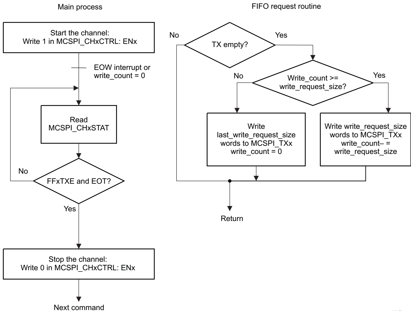
Figure 20-40. Transmit-Only
