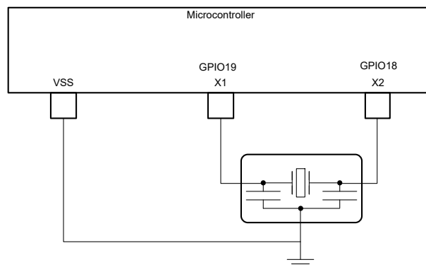
Figure 6-13. External Resonator
