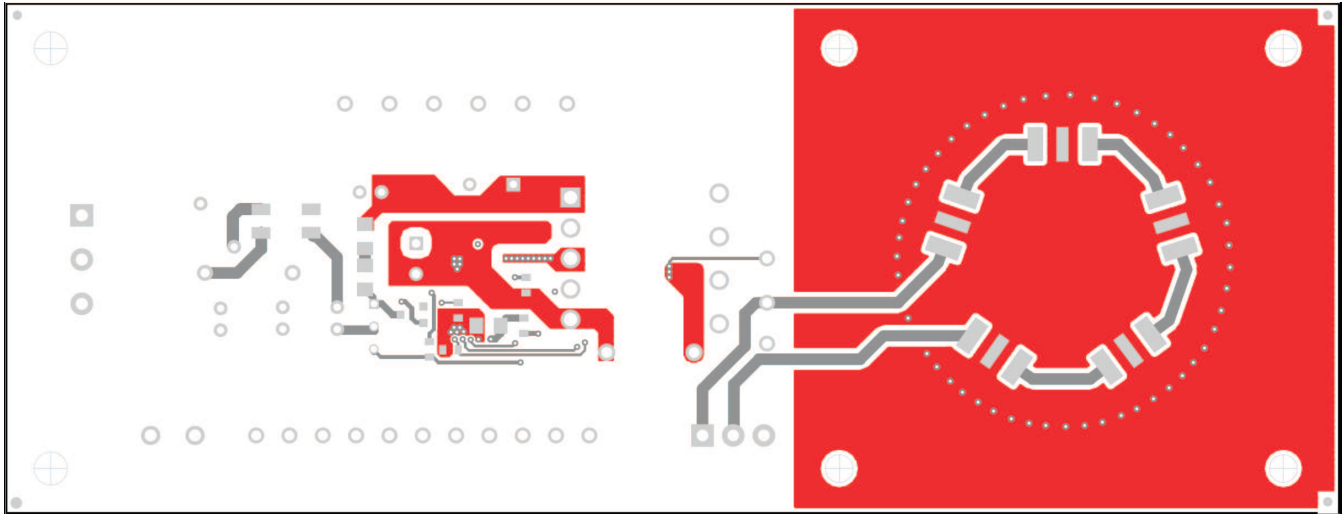
Figure 21. TPS92070EVM-682 Top Copper (top view)
