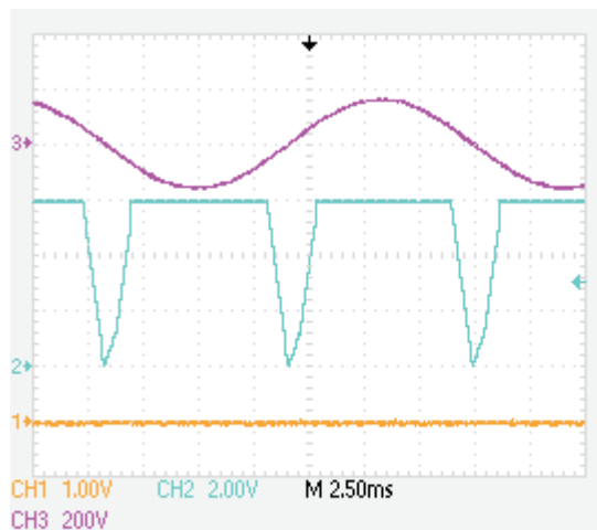
Figure 14. TDD, Full Load, No Dimmer (CH1 = TDD, CH2 = SEN, CH3 = VIN (115 VAC)) (TDD signal low when there is no dimmer detected on the input, Valley Fill PFC is enabled)
