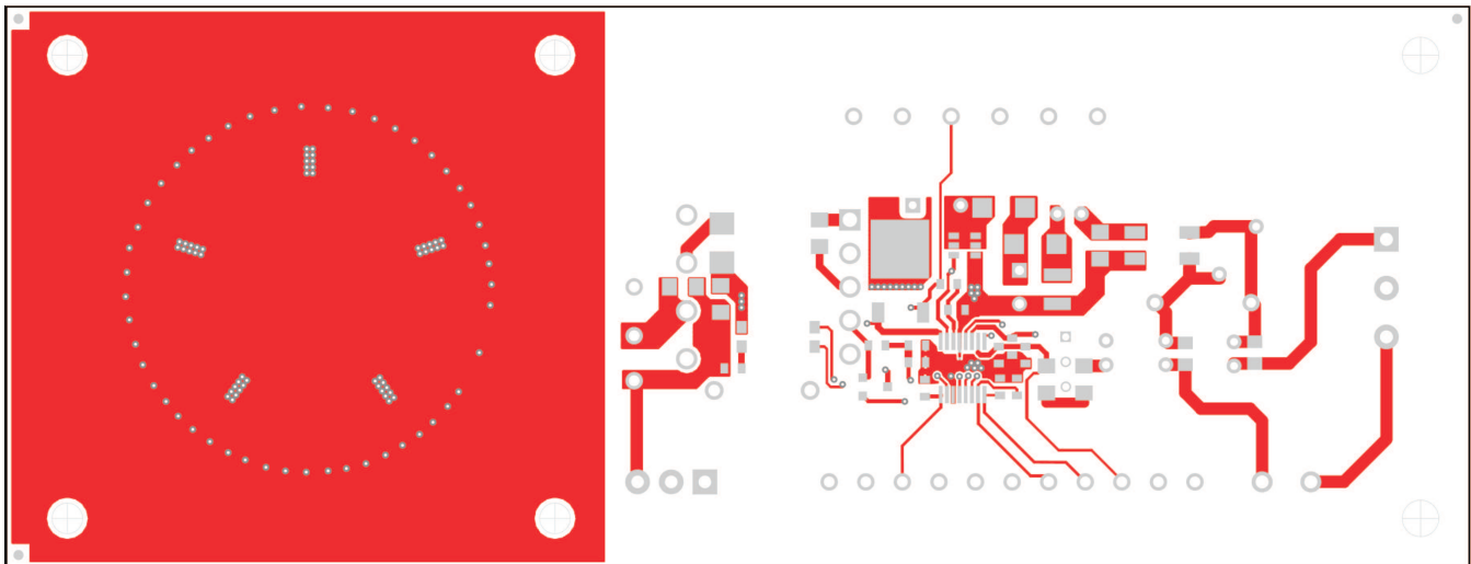
Figure 24. TPS92070EVM-682 Bottom Copper (bottom view)
