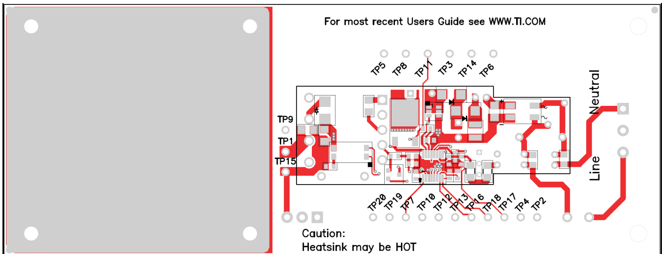
Figure 22. TPS92070EVM-682 (bottom view)
