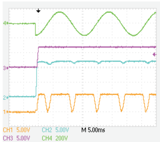
Figure 7. Turn On, Full Load, No Dimmer (CH1 = SEN, CH2 = VDD, CH3 = BP, CH4 = VIN (115 VAC))
