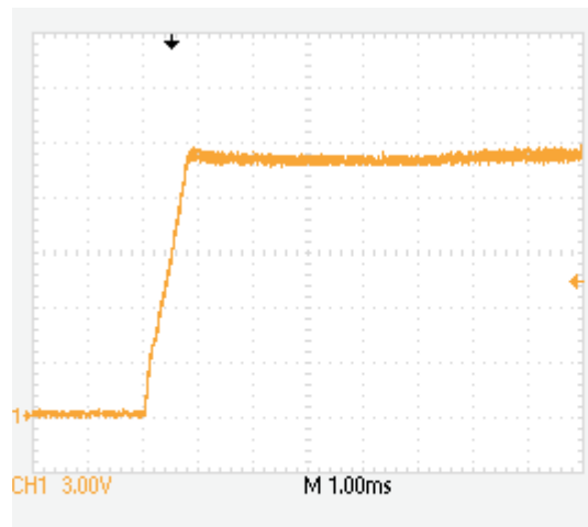
Figure 8. LED Turn On, Full Load, No Dimmer (VIN = 115 VAC, CH1 = VOUT)
