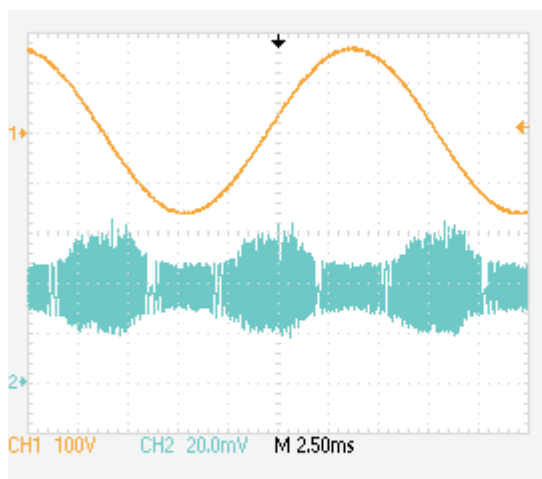
Figure 10. LED Output Voltage Ripple, Full Load, No Dimmer ( V_{IN} = 115 VAC, CH1 = V_{OUT} )
