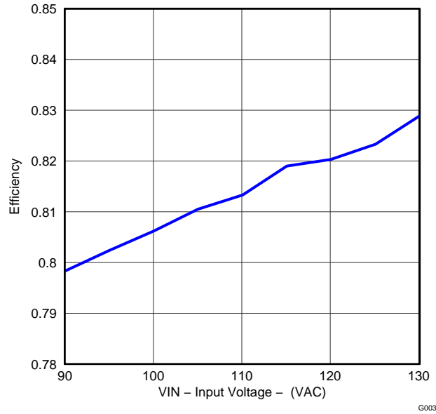
Figure 3. TPS92070EVM-682 Efficiency with Respect to Line Voltage, No Dimmer
