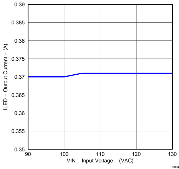
Figure 4. TPS92070EVM-682 LED Current Regulation with Respect to Line Voltage, No Dimmer
