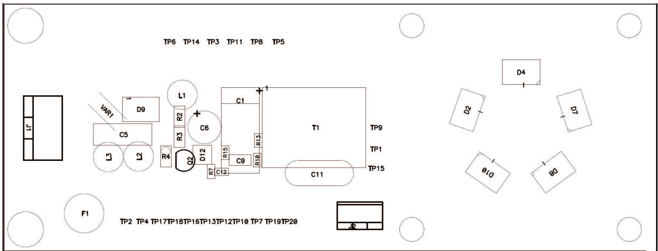
Figure 20. TPS92070EVM-682 Top Layer Assembly Drawing (top view)
