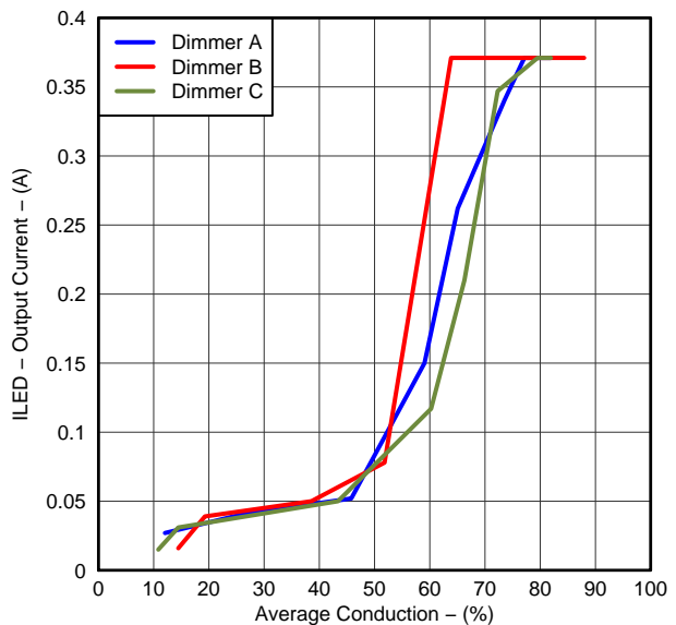
Figure 6. LED Current with Respect to Average Dimmer Conduction
