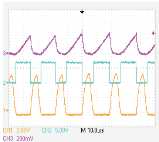
Figure 16. Valley Detect, Full Load, No Dimmer (VIN = 115 VAC, CH1 = VD, CH2 = GATE, CH3 = PCS)
