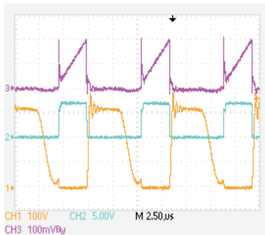
Figure 13. Switching Waveforms, Full Load, No Dimmer (VIN = 115 VAC, CH1 = Q3 Drain, CH2 = GATE, CH3 = PCS)
