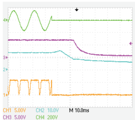
Figure 17. Turn Off, Full Load, No Dimmer (CH 1 = SEN, CH2 = VDD, CH3 = BP, CH4 = VIN (115 VAC))
