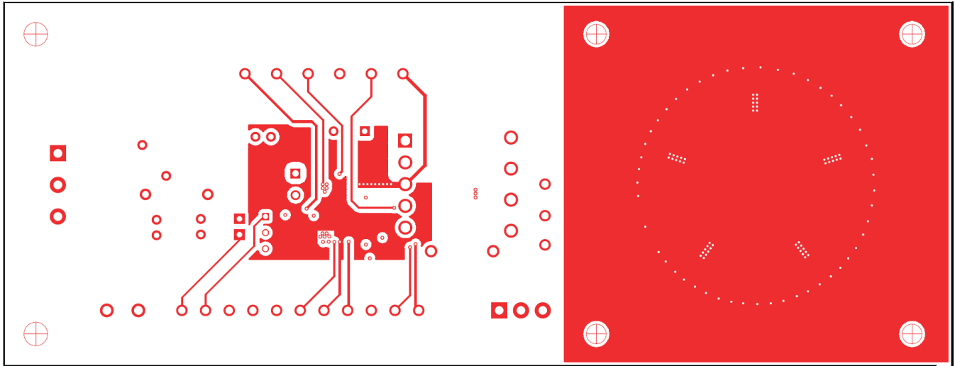
Figure 25. TPS92070EVM-682 Internal Layer 1 (top view)
