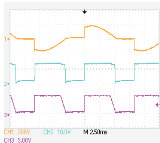
Figure 18. Dimmer Detection, With Dimmer (CH1 = VIN (115 VAC), CH2 = DTC, CH3 = SEN) (DTC sinks current during AC zero crossing to allow the TRIAC timing circuit to charge, initiating next TRIAC firing)
