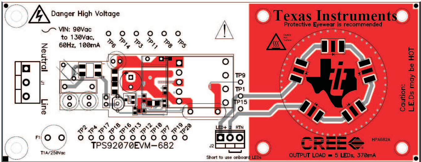
Figure 19. TPS92070EVM-682 (top view)
