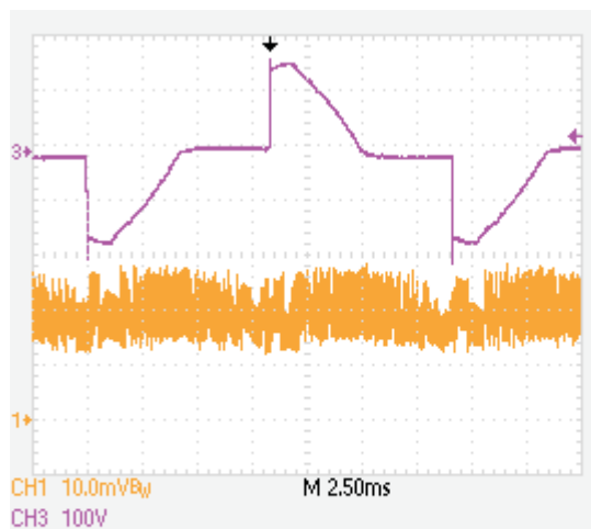
Figure 12. LED Output Current Ripple, With Dimmer (CH1 = I LED , scale = 50 mA/div, CH3 = VIN (115 VAC))
