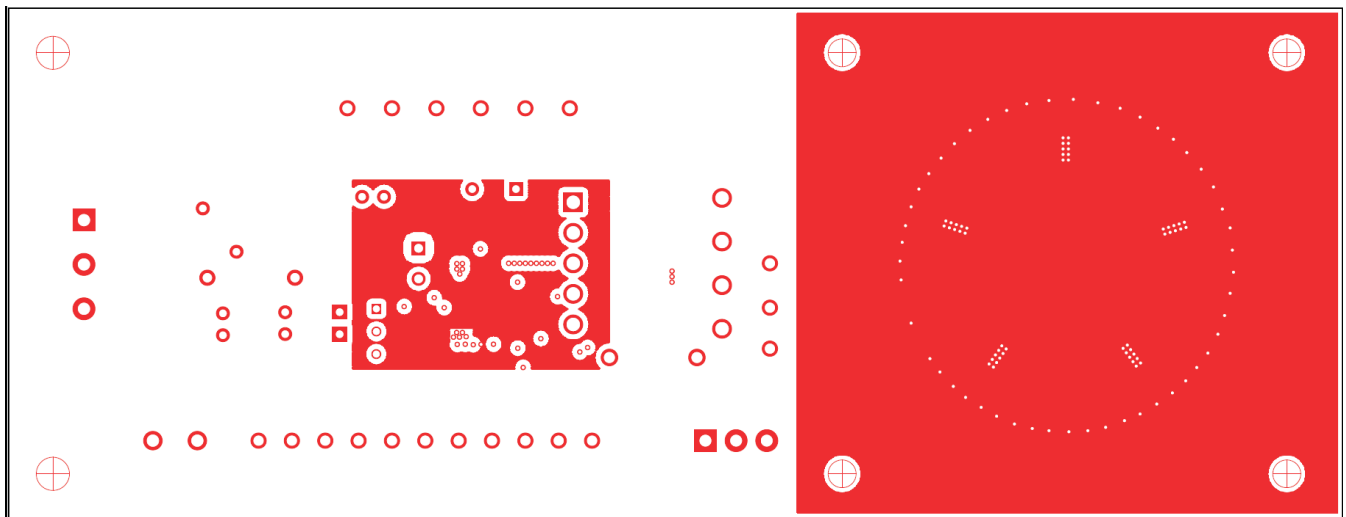
Figure 26. TPS92070EVM-682 Internal Layer 2 (top view)
