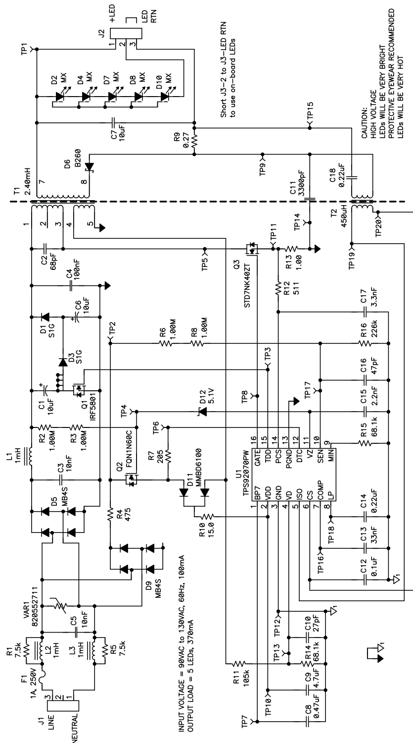
Figure 1. TPS92070EVM-682 Schematic
