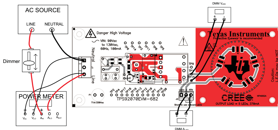
Figure 2. TPS92070EVM-682 Recommended Test Set Up
