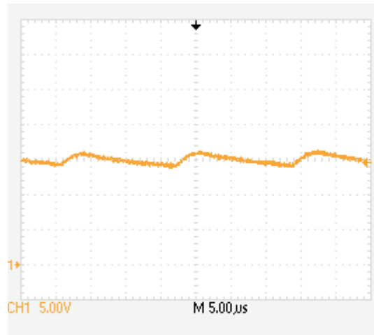
Figure 11. LED Output Current Ripple, Full Load, No Dimmer (CH1 = VIN (115 VAC), CH2 = I LED , scale = 200 mA/div)
