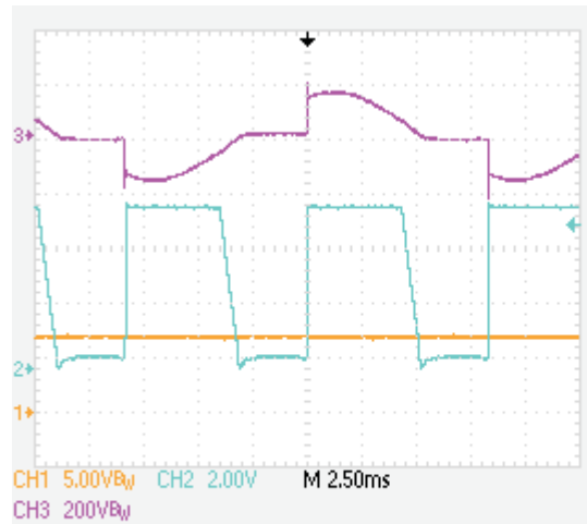
Figure 15. TDD, With Dimmer (CH1 = TDD, CH2 = SEN, CH3 = VIN (115 VAC)) (TDD signal high when there is a dimmer detected on the input, Valley Fill PFC is disabled)
