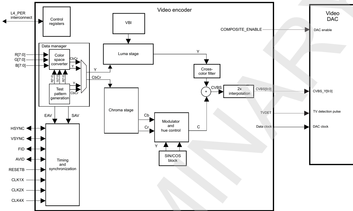
Figure 10-180. Video Encoder Architecture Overview
