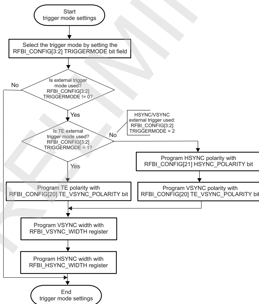
Figure 10-172. Trigger Mode Settings
