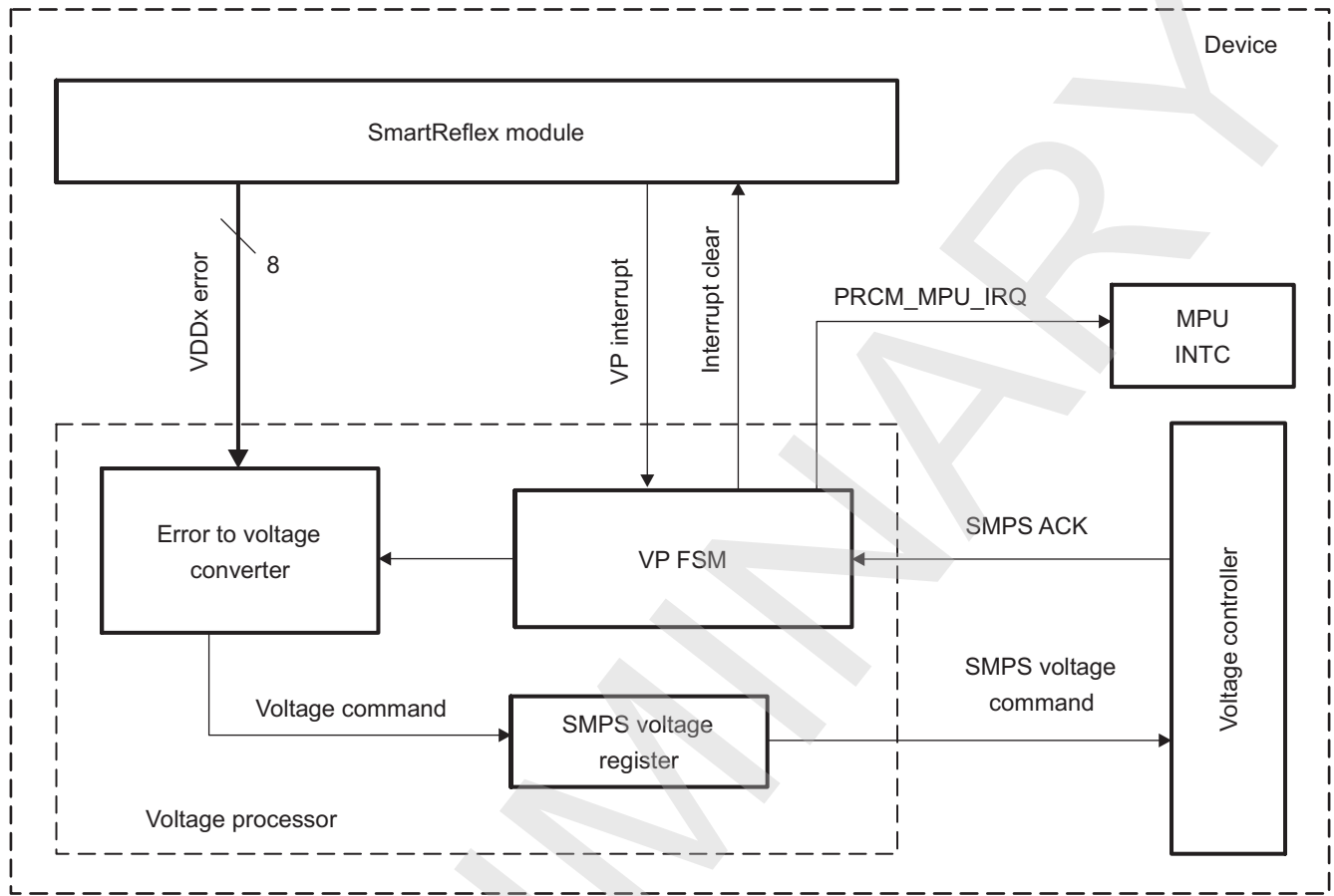
Figure 3-72. Voltage Processor Functional Overview
