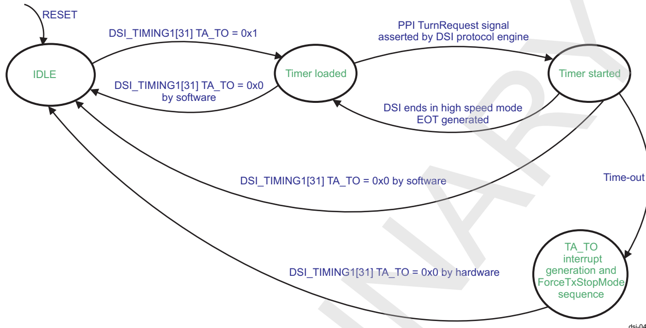
Figure 10-137. TurnRequest FSM
