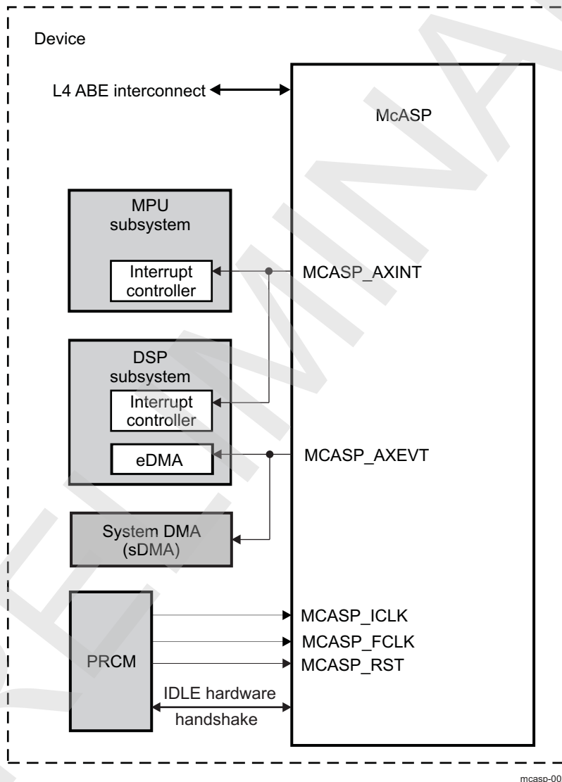
Figure 23-192. McASP Integration
