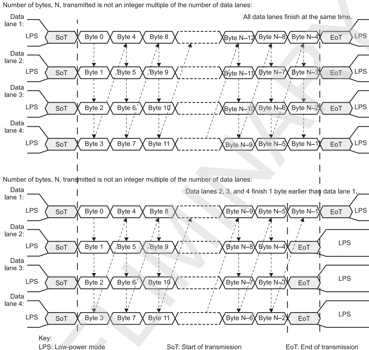
Figure 8-35. ISS CSI2 Four Data-Lane Merger Configuration
