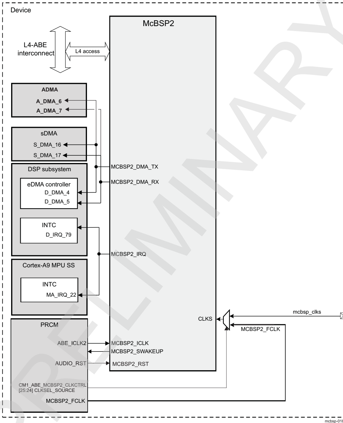
Figure 23-125. McBSP2 Integration
