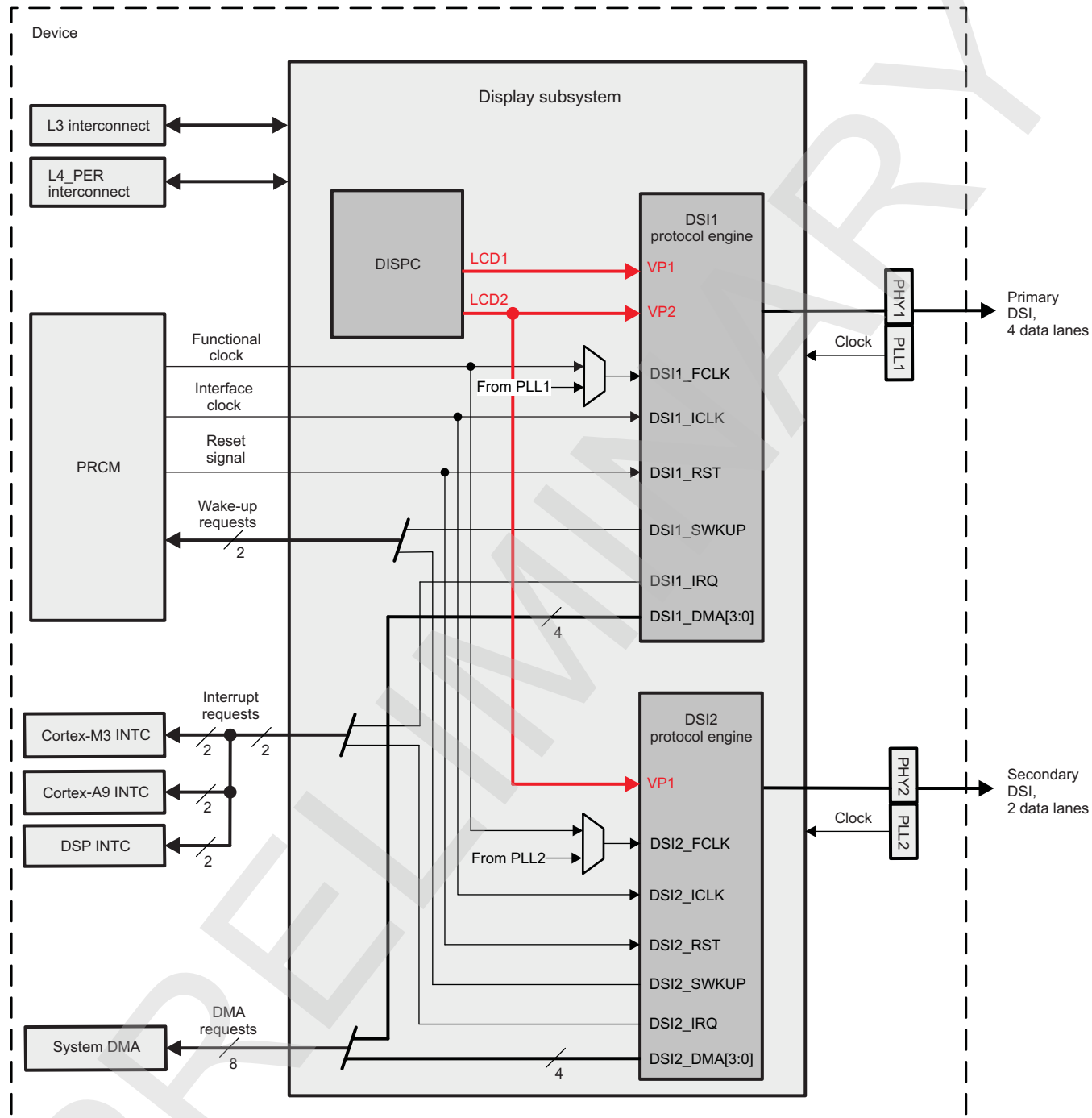
Figure 10-94. DSI Overview
