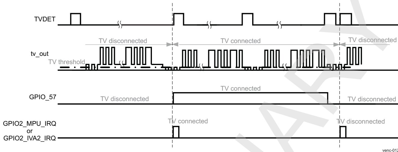
Figure 10-187. GPIO Signal Waveform Proposal for TV Detection/Disconnection in AC-Coupling Mode
