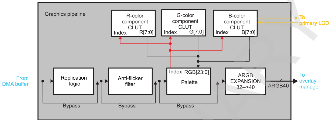
Figure 10-41. Graphics Pipeline
