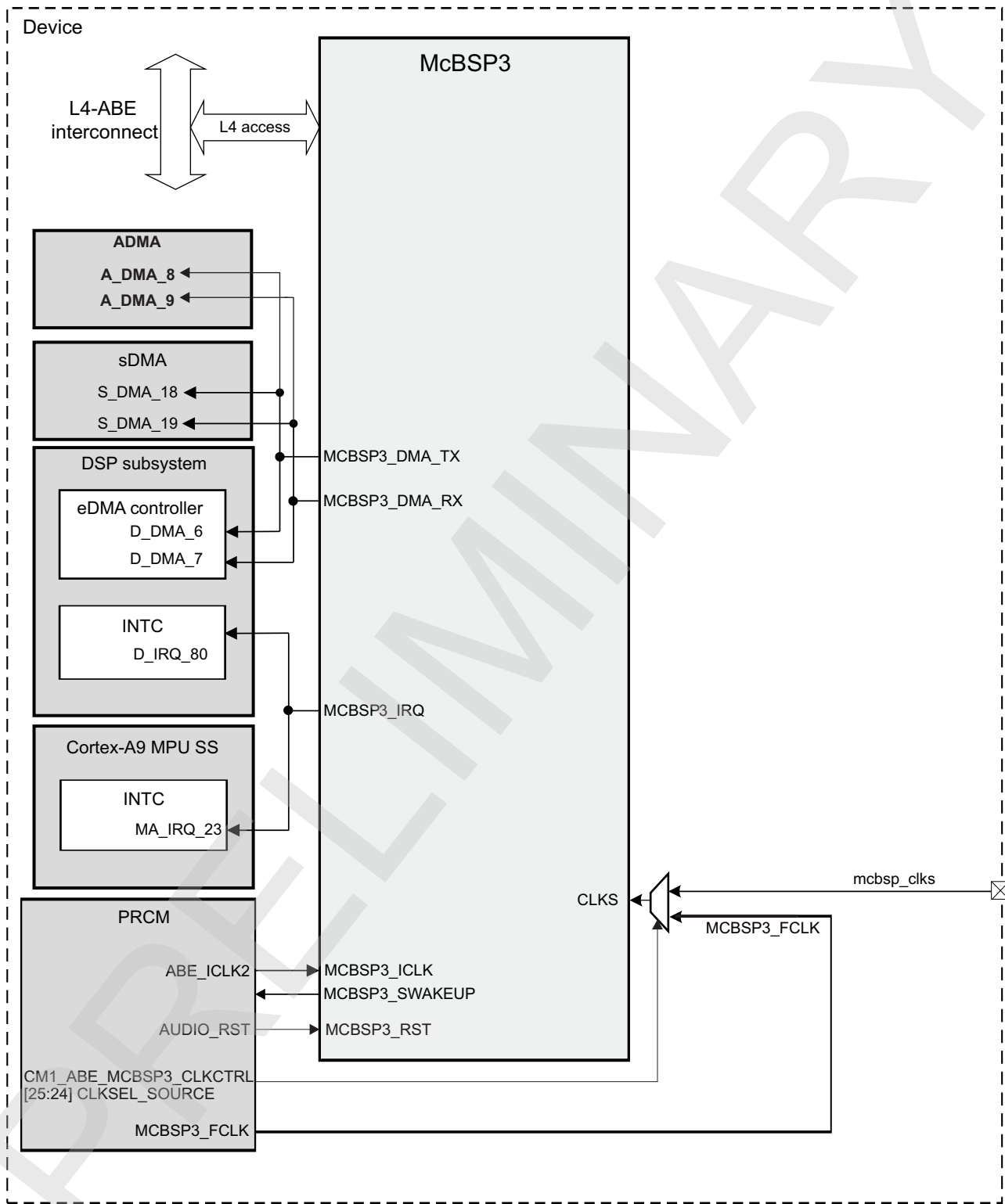
Figure 23-126. McBSP3 Integration
