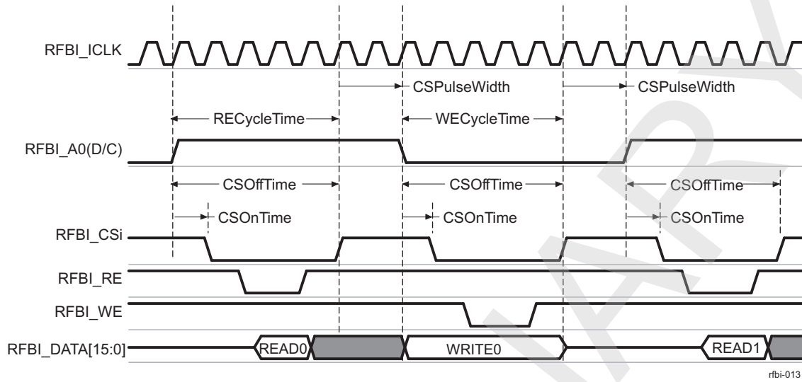
Figure 10-163. Read to Write and Write to Read
