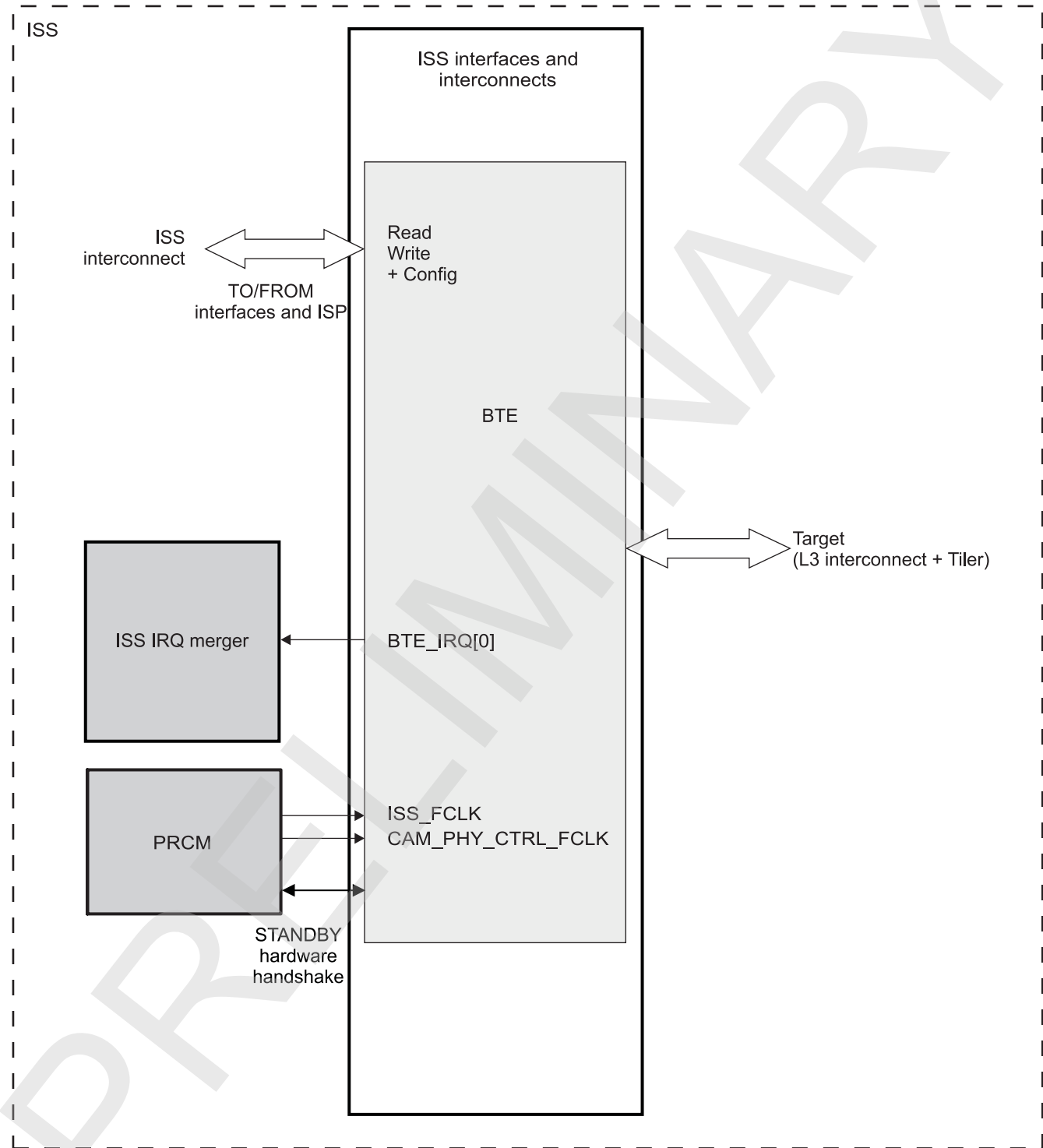
Figure 8-76. ISS BTE Integration
