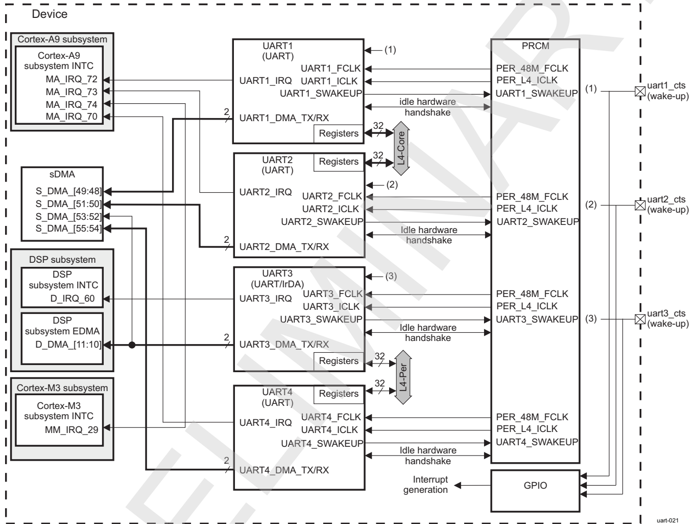
Figure 23-71. UART/IrDA/CIR Integration
