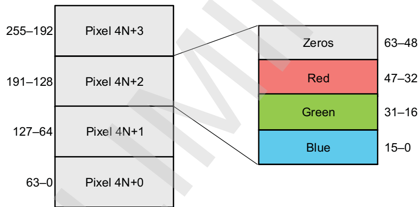
Figure 8-154. ISS ISP IPIPE Boxcar Data Packing in SDRAM
