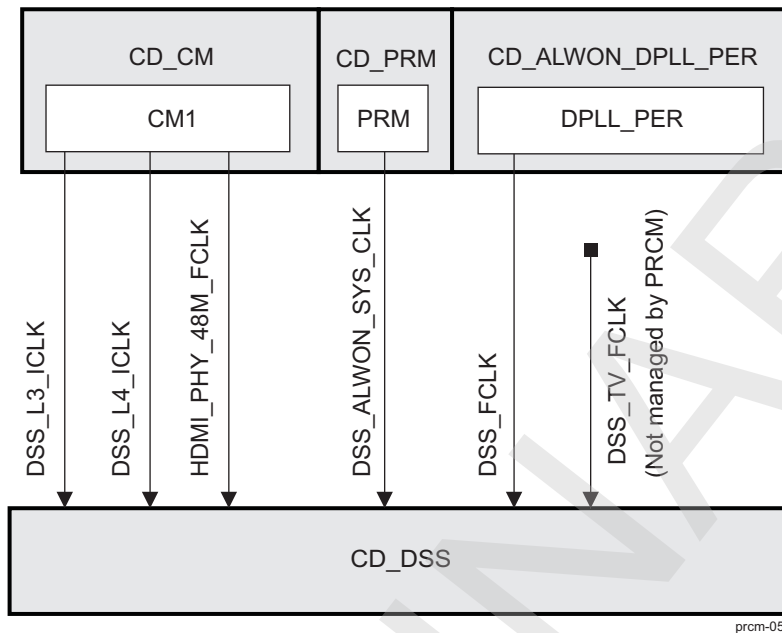
Figure 3-57. CD_DSS Overview
