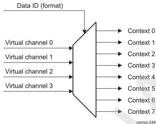
Figure 8-66. ISS CSI2 Virtual Channel to Context
