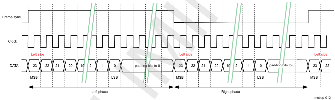
Figure 23-120. Left Justified Data Format; Word Width: 32 Bits; Data Length: 24 Bits
