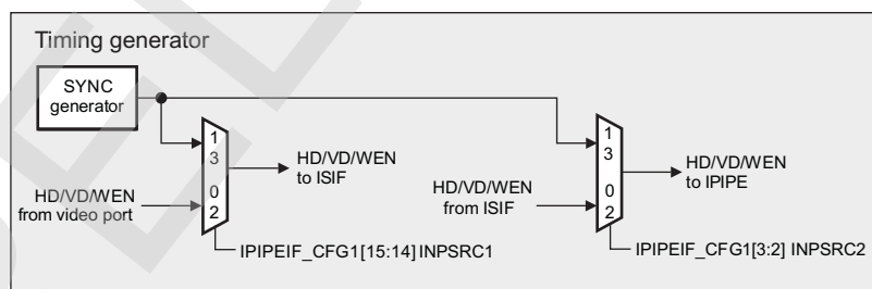
Figure 8-120. ISS ISP IPIPEIF Timing Generator Submodule Description
