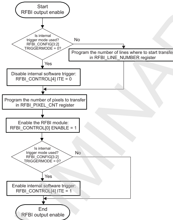
Figure 10-173. RFBI Output Enable Flow Chart
