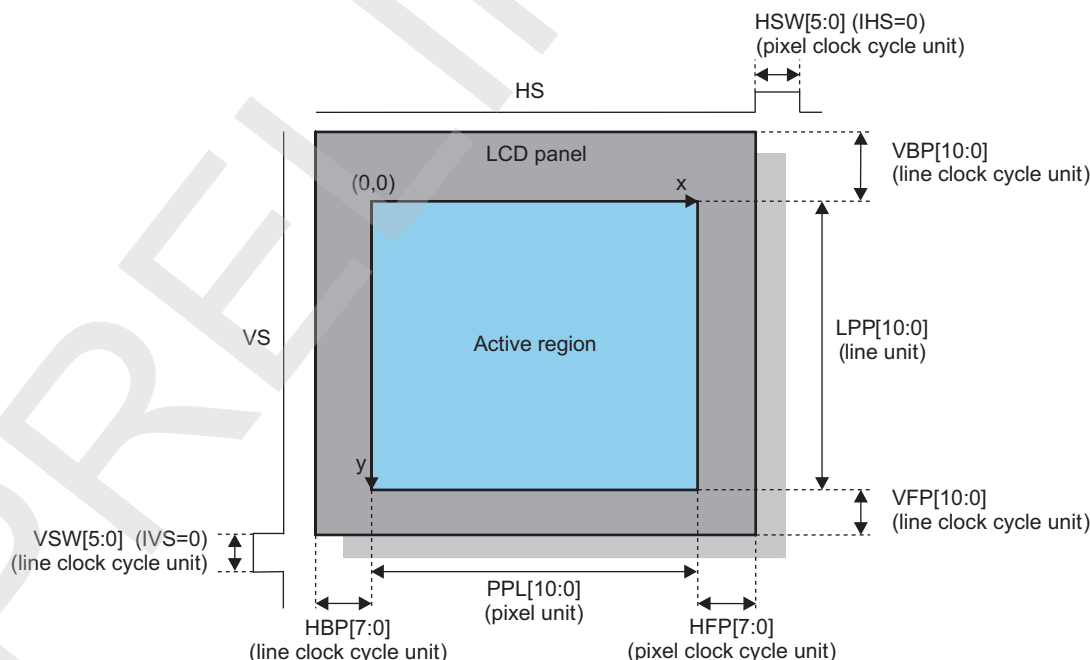
Figure 10-84. Timing Values (Active Matrix Display)
