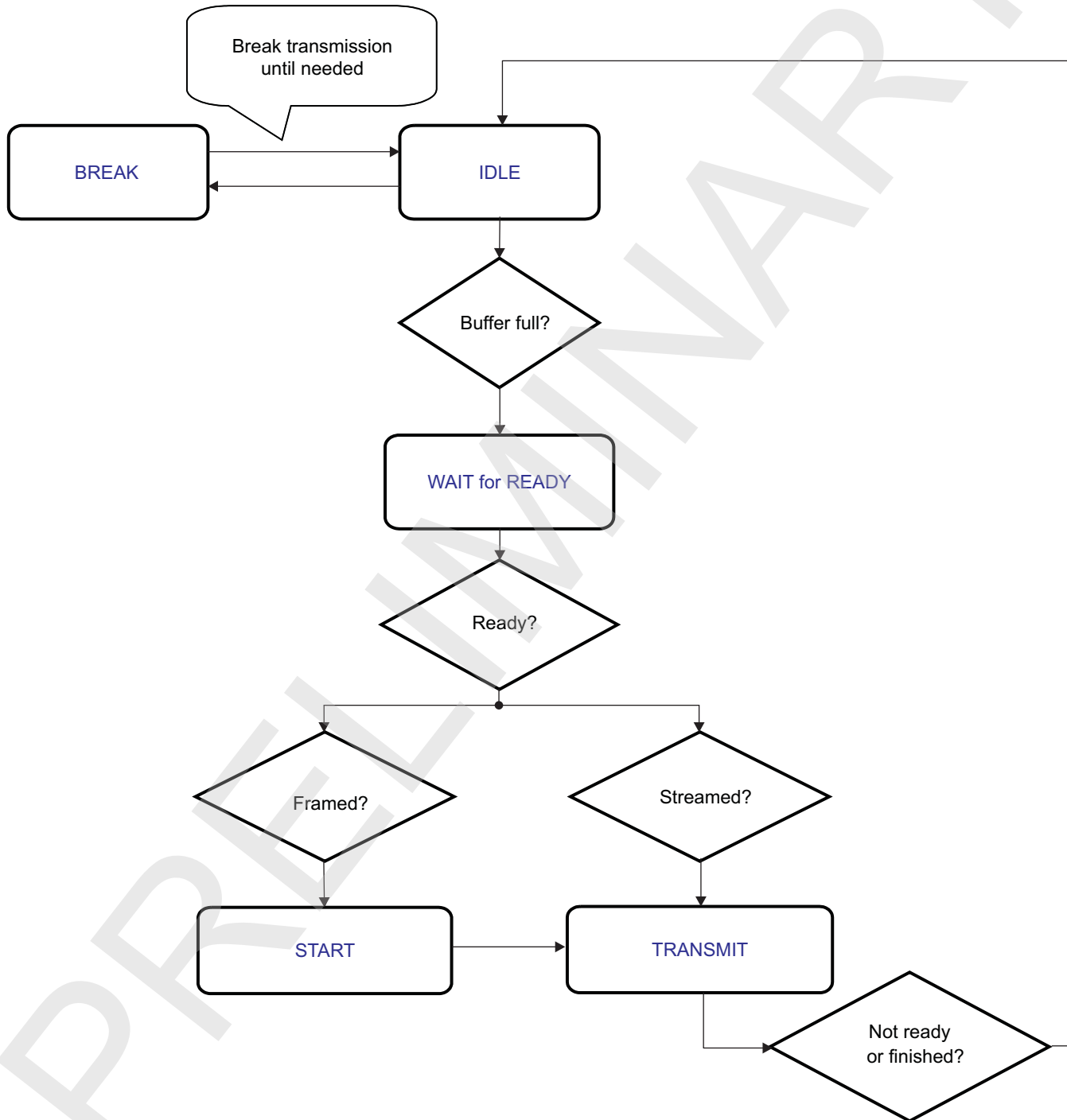
Figure 23-226. Transmit FSM
