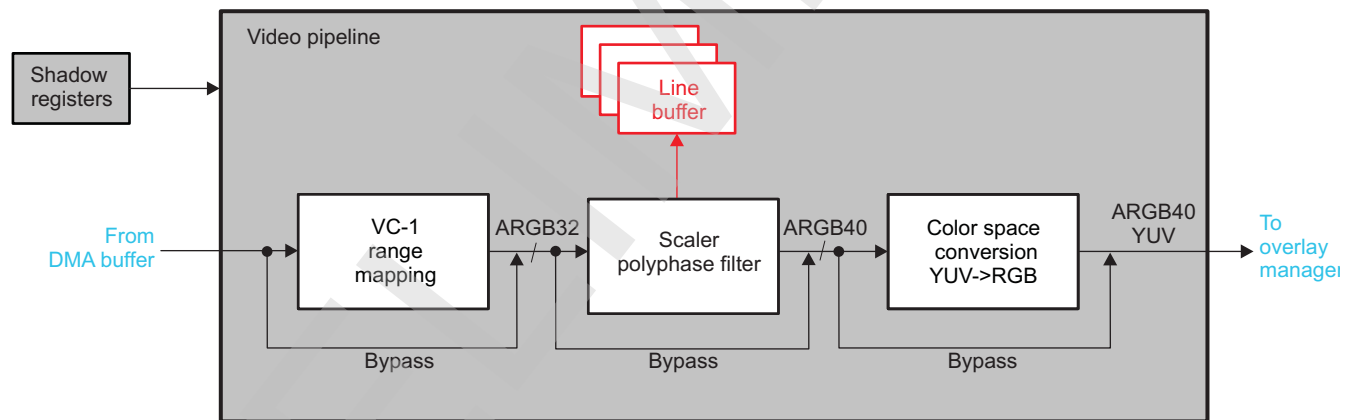
Figure 10-47. Configuration 2: Video Pipeline
