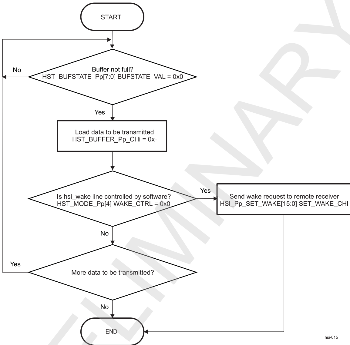
Figure 23-232. HSI Transmit in Polling Method
