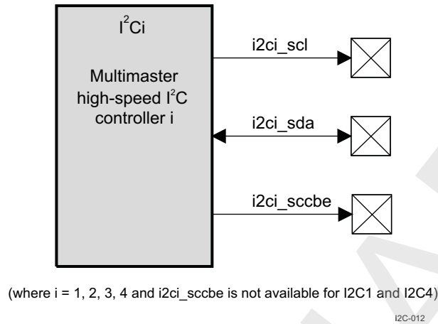
Figure 23-12. HS I 2 C Interface Signals in SCCB Mode
