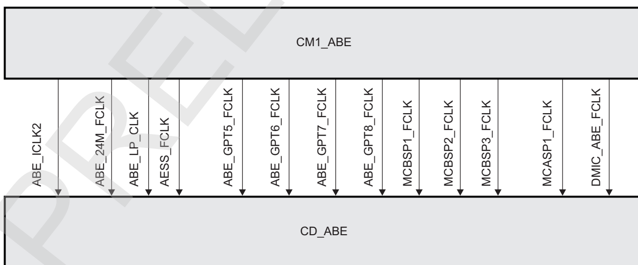
Figure 3-67. CD_ABE Overview
