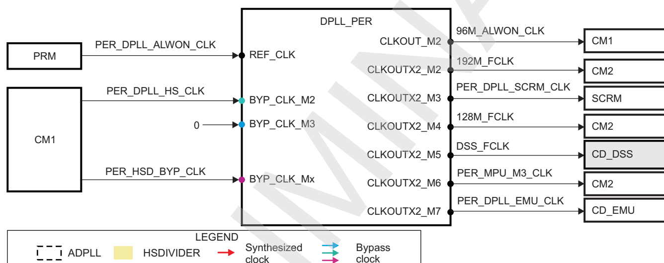
Figure 3-41. DPLL_PER Overview
