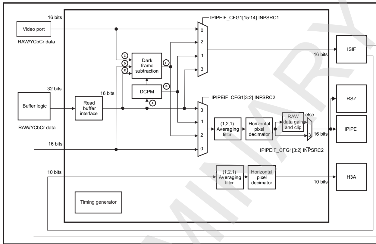
Figure 8-108. ISS ISP IPIPEIF Top-Level Block Diagram
