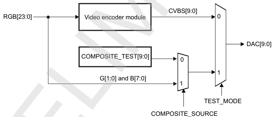
Figure 10-188. DAC Test Mode in Composite Video Mode
