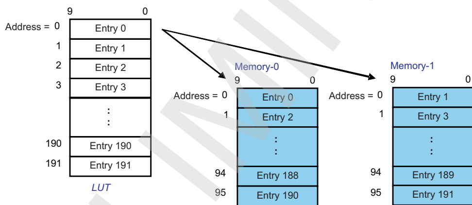
Figure 8-185. ISS ISP ISIF Linearization LUT Memories
