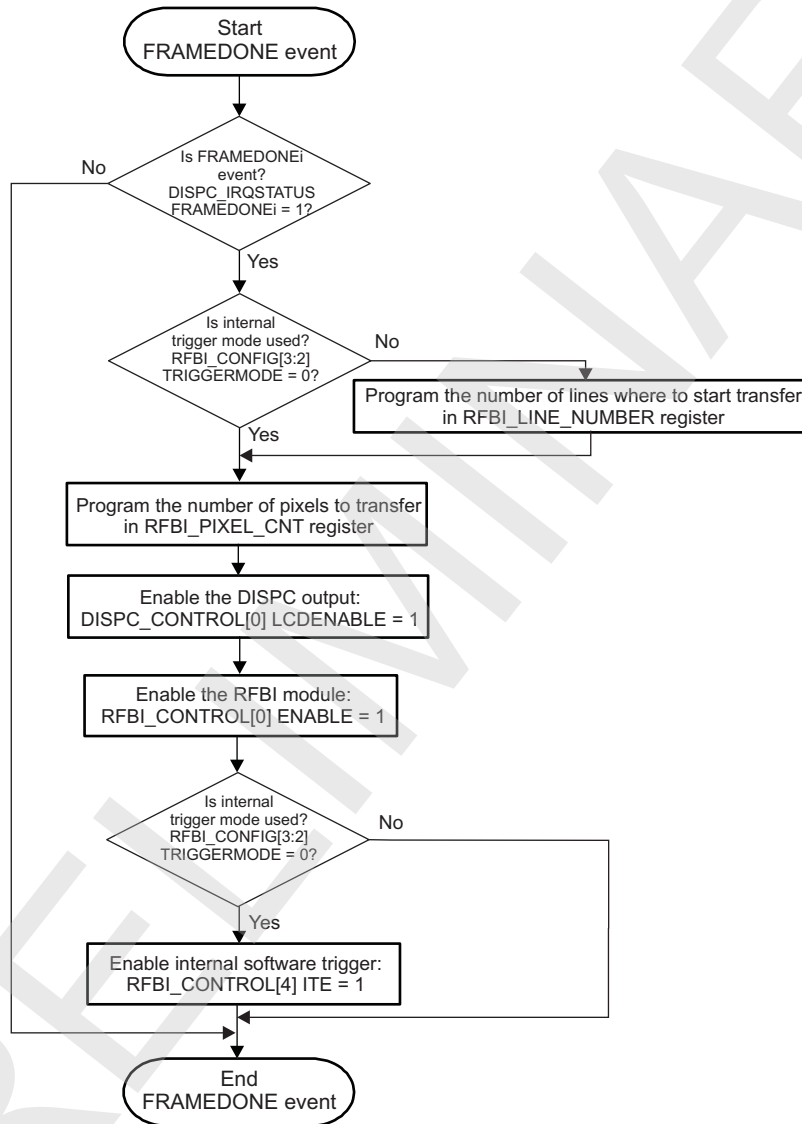
Figure 10-174. FRAMEDONE Event Servicing Flow Chart
