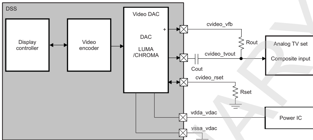
Figure 10-177. Video Encoder Environment, AC-Coupling
