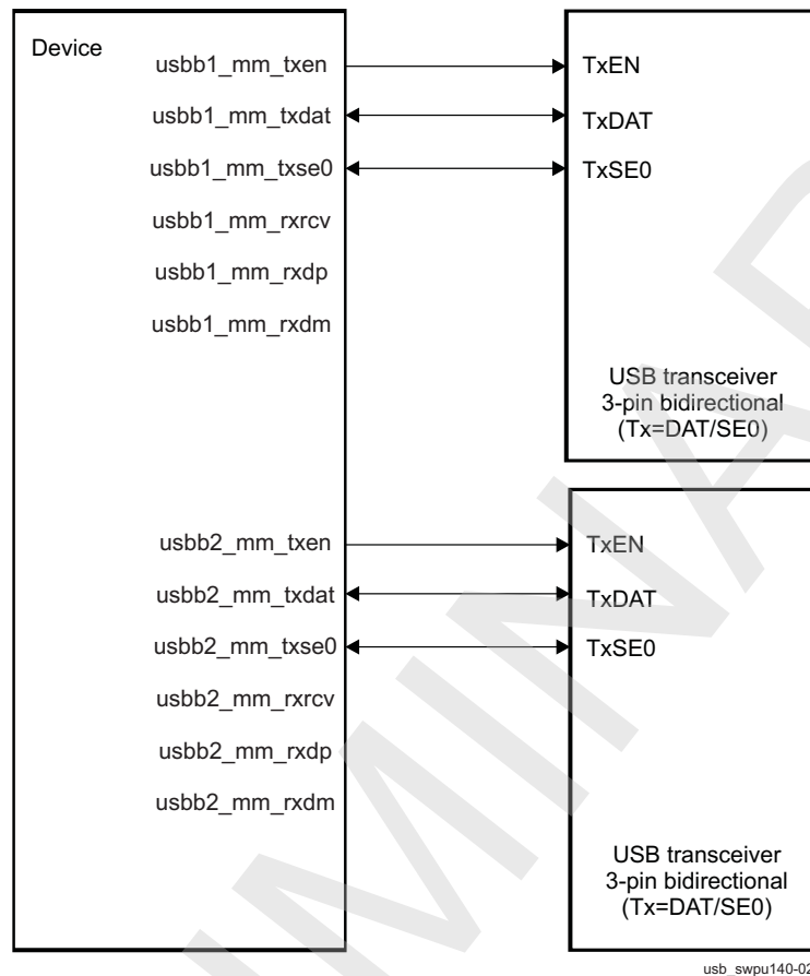
Figure 23-245. 3-Pin Bidirectional Using DAT/SE0 Signaling
