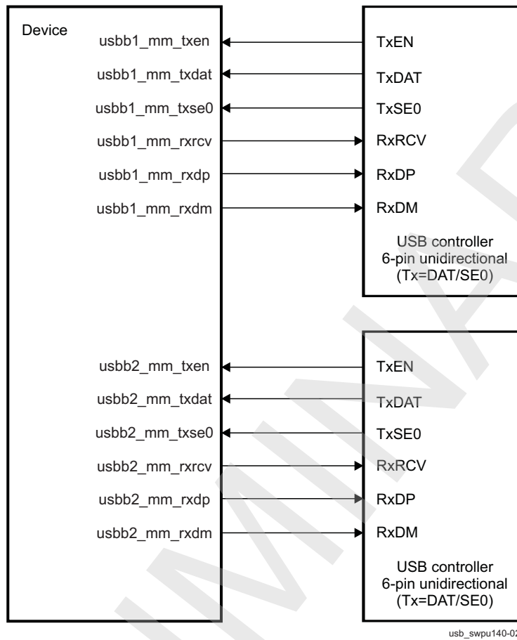
Figure 23-247. 6-Pin Unidirectional TLL Using DAT/SE0 Signaling
