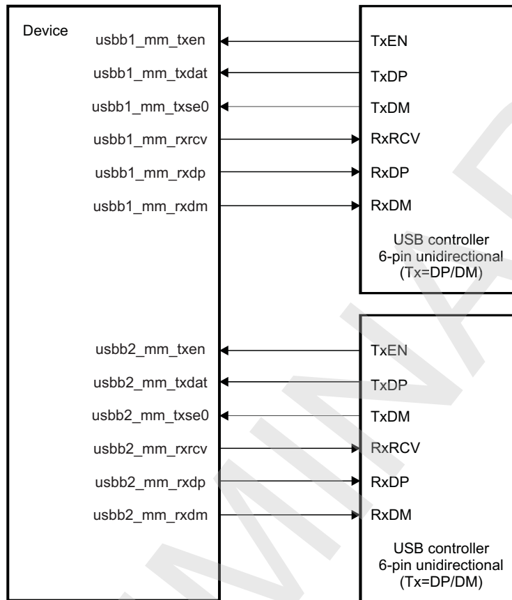
Figure 23-248. 6-Pin Unidirectional TLL Using DP/DM Signaling
