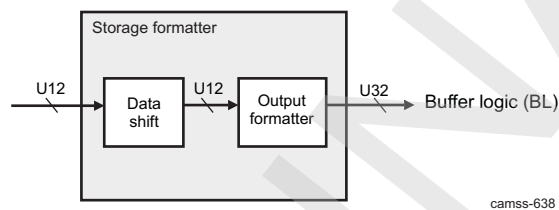
Figure 8-225. ISS ISP ISIF Storage Formatter Block Diagram
