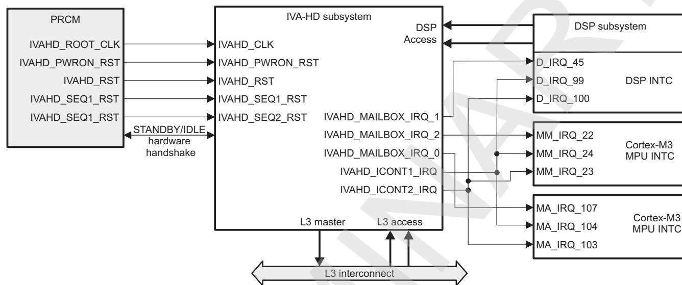
Figure 6-2. IVA-HD Integration
