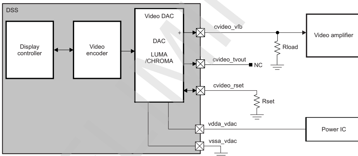
Figure 10-178. Video Encoder Environment, Bypass Mode
