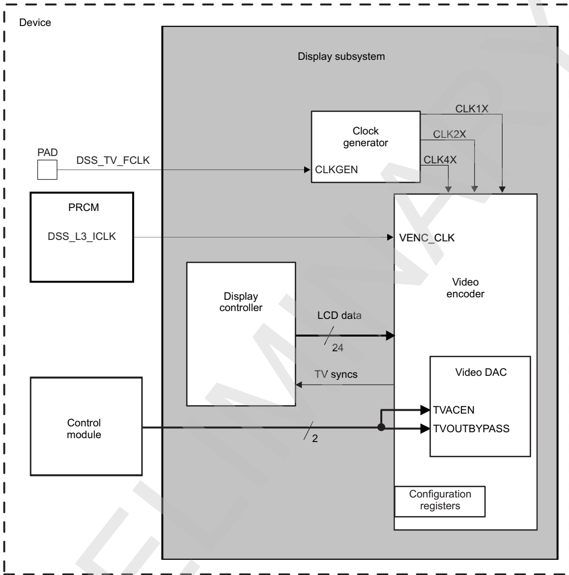
Figure 10-179. Video Encoder Integration
