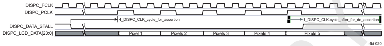
Figure 10-166. RFBI Data Stall Signal Diagram With PCD=3
