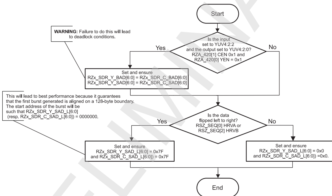
Figure 8-235. ISS ISP RSZ Global Image Processing Settings – Subsequence 2
