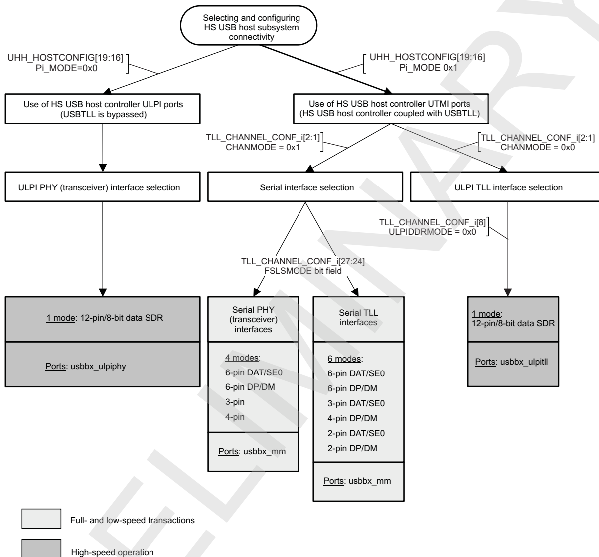
Figure 23-257. Selecting and Configuring HS USB Host Subsystem Connectivity
