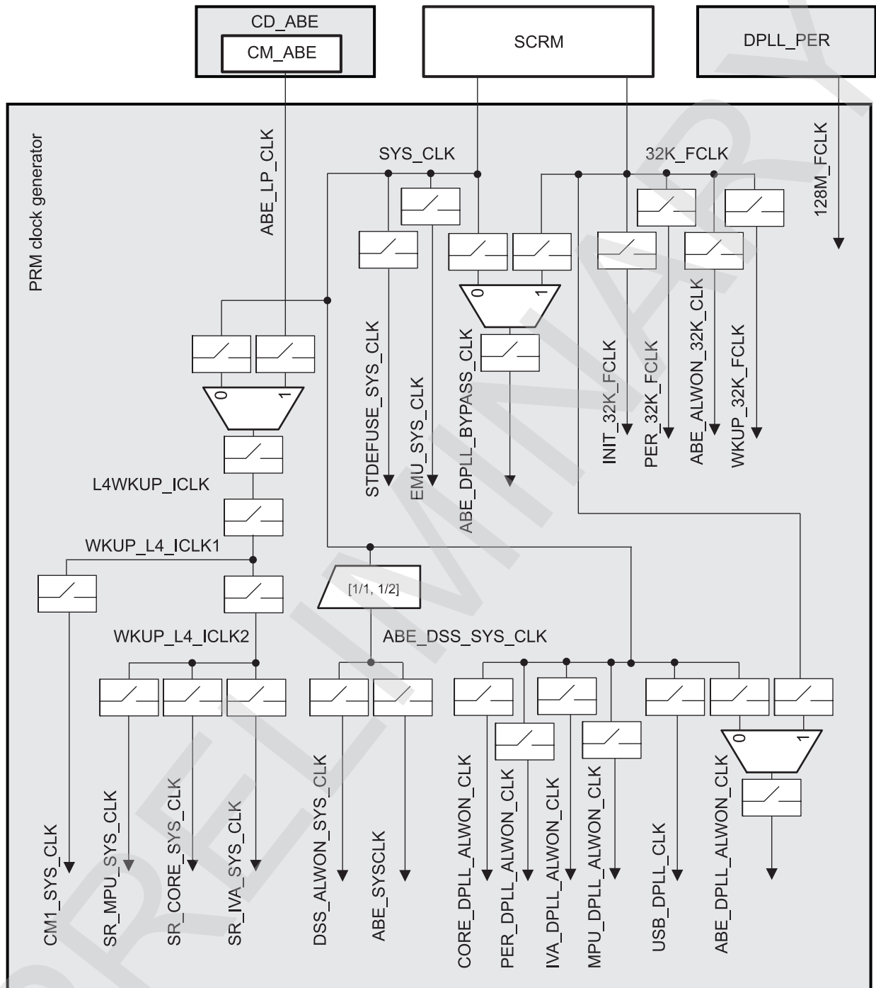
Figure 3-33. PRM Clock Manager Overview (a)
