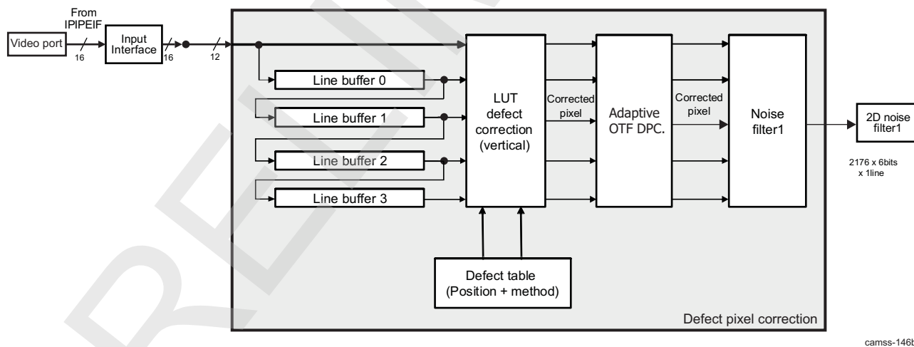
Figure 8-130. ISS ISP IPIPE Defect Pixel Correction
