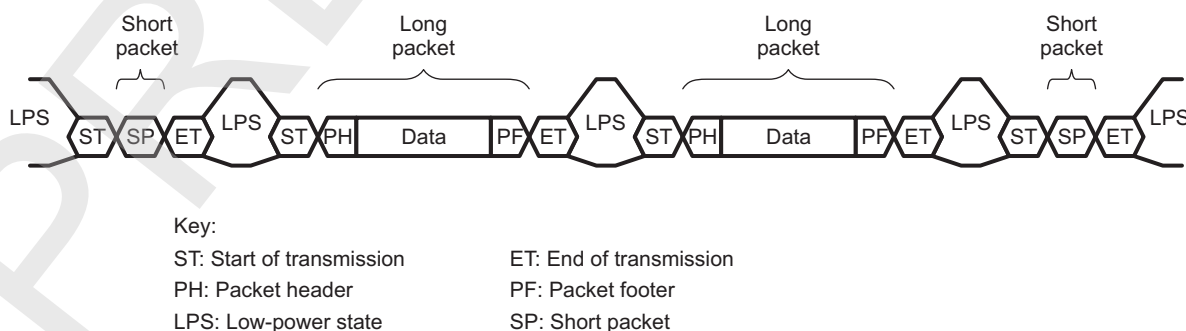
Figure 10-97. Protocol Layer With Short and Long Packets
