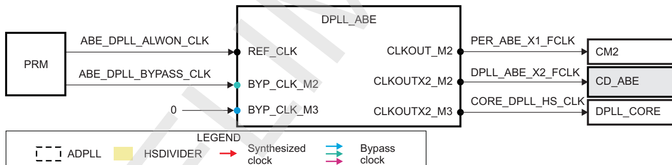
Figure 3-43. DPLL_ABE Overview
