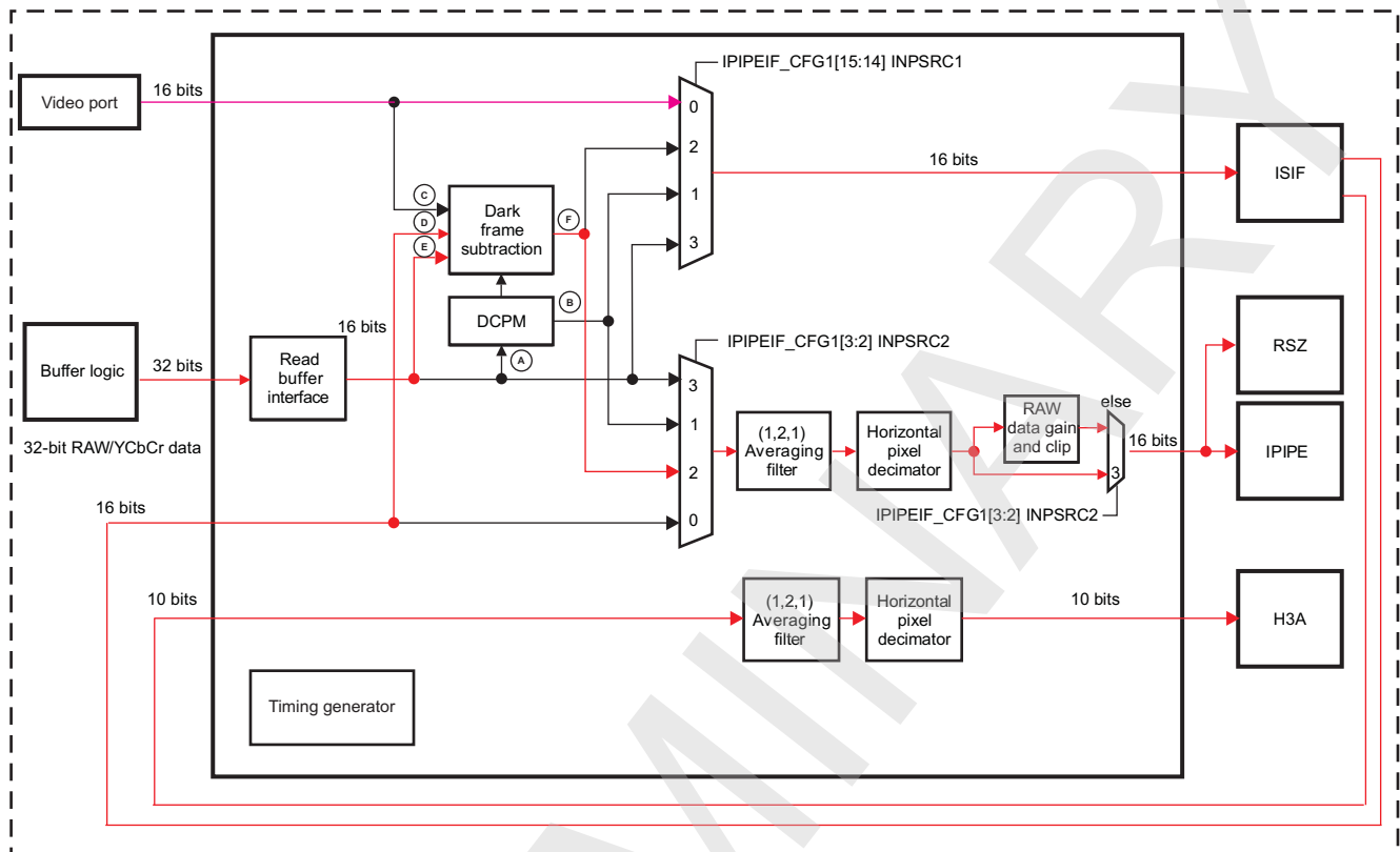
Figure 8-114. ISS ISP IPIPEIF INPSRC1= 0 and INPSRC2 = 2 Data Paths
