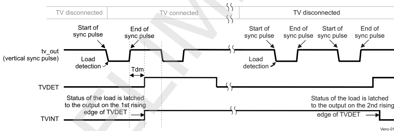
Figure 10-184. DC-Coupling TV Detect Waveforms for TV Connected and Disconnected
