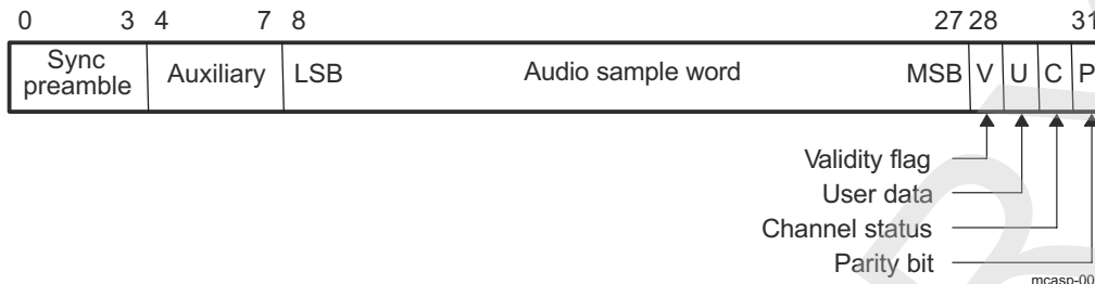
Figure 23-190. S/PDIF Subframe Format
