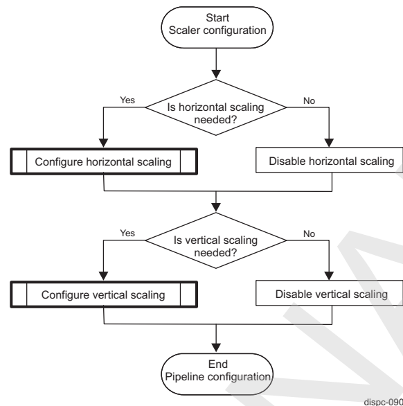
Figure 10-93. Scaler Unit Programming Flow
