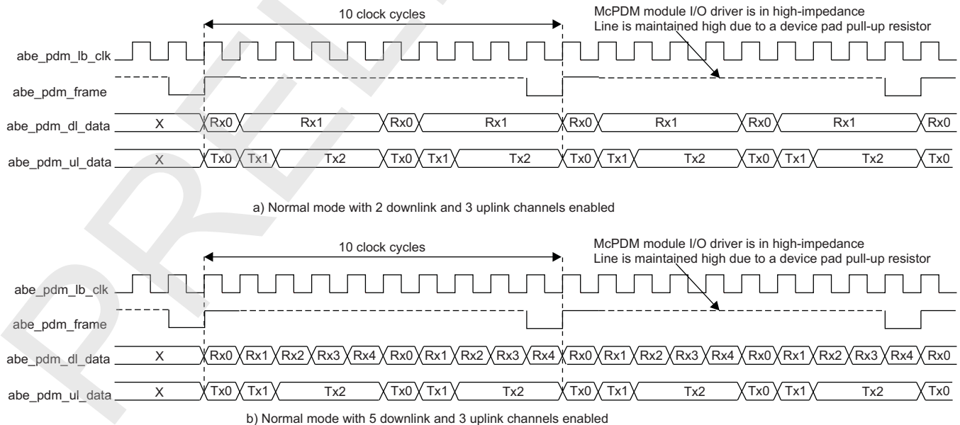
Figure 23-162. Protocols and Data Formats in Normal Mode
