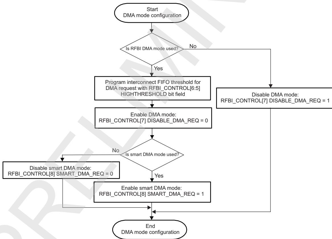
Figure 10-171. DMA Mode Configuration
