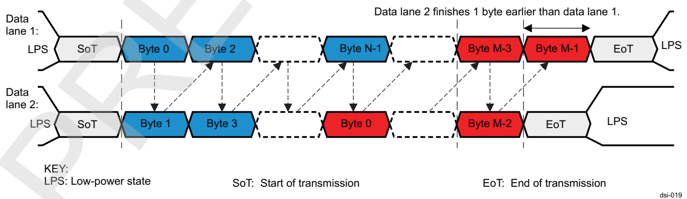
Figure 10-112. Two Packets Using Two-Data Lane Configuration (Example)
