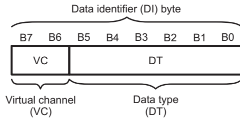
Figure 8-39. ISS CSI2 Data Identifier Structure
