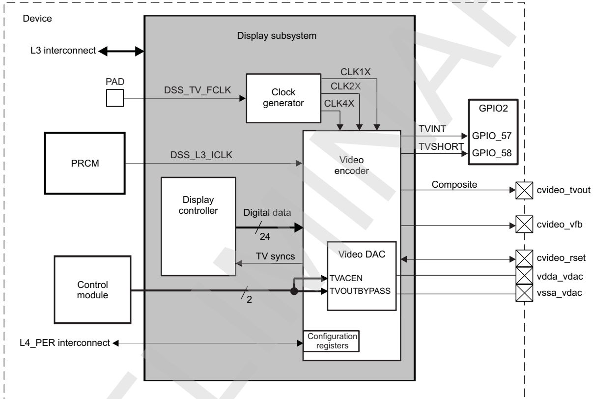
Figure 10-175. Video Encoder Overview
