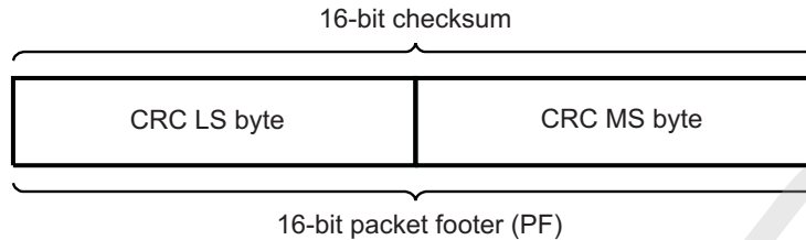
Figure 10-141. Checksum Transmission
