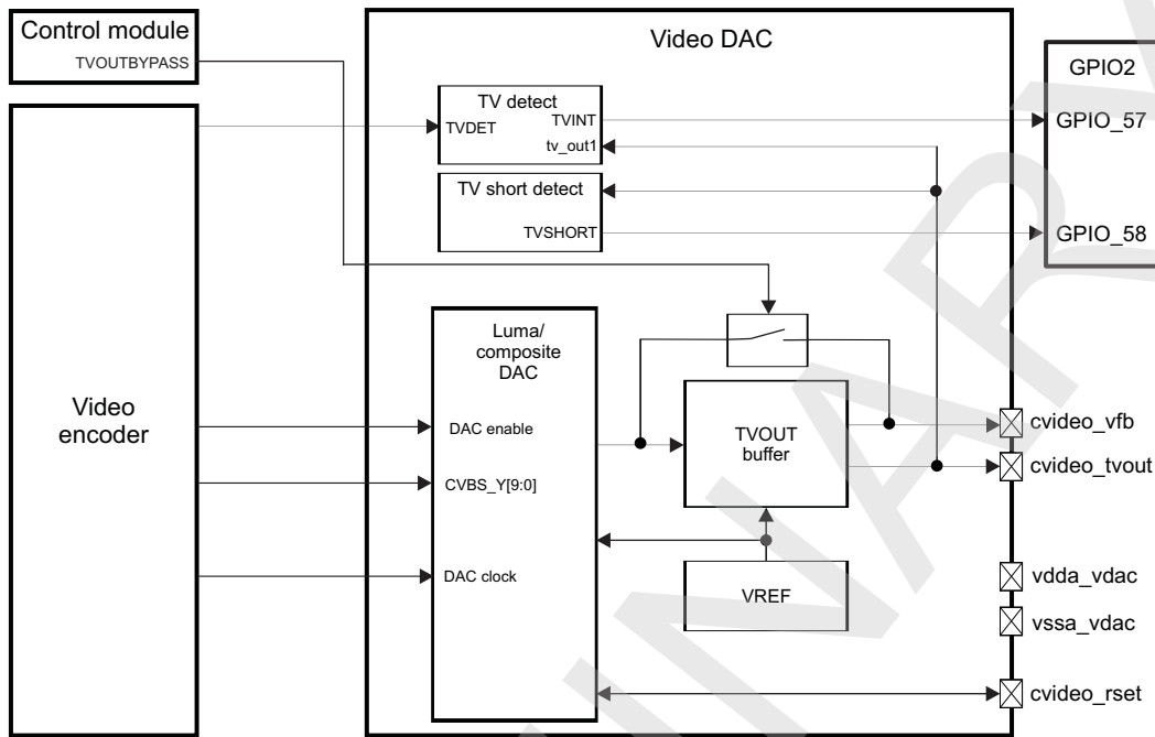
Figure 10-183. 10-Bit Video DAC Architecture
