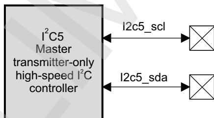
Figure 23-16. HS I 2 C I2C5 Interface Signals
