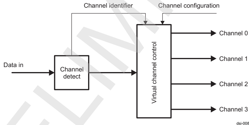
Figure 10-101. VC Controller
