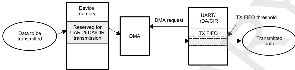
Figure 23-80. DMA Transmission
