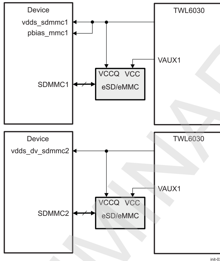
Figure 27-27. eMMC/eSD Connection
