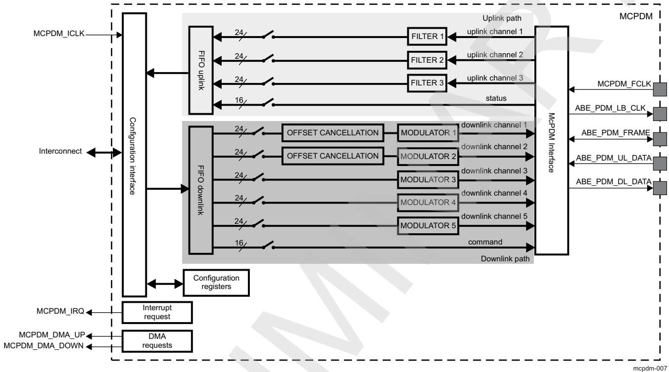
Figure 23-166. McPDM Block Diagram
