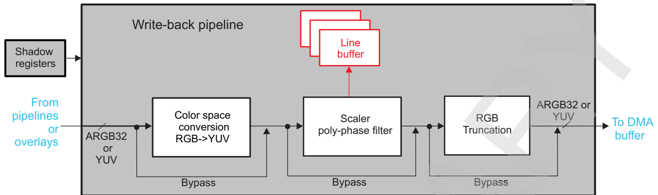
Figure 10-64. Write-back Pipeline
