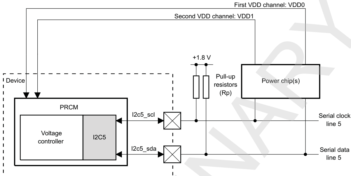
Figure 23-15. HS I 2 C and Typical Connection Between the HS I 2 C and Power Chip(s)
