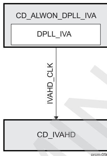
Figure 3-54. CD_IVAHD Overview
