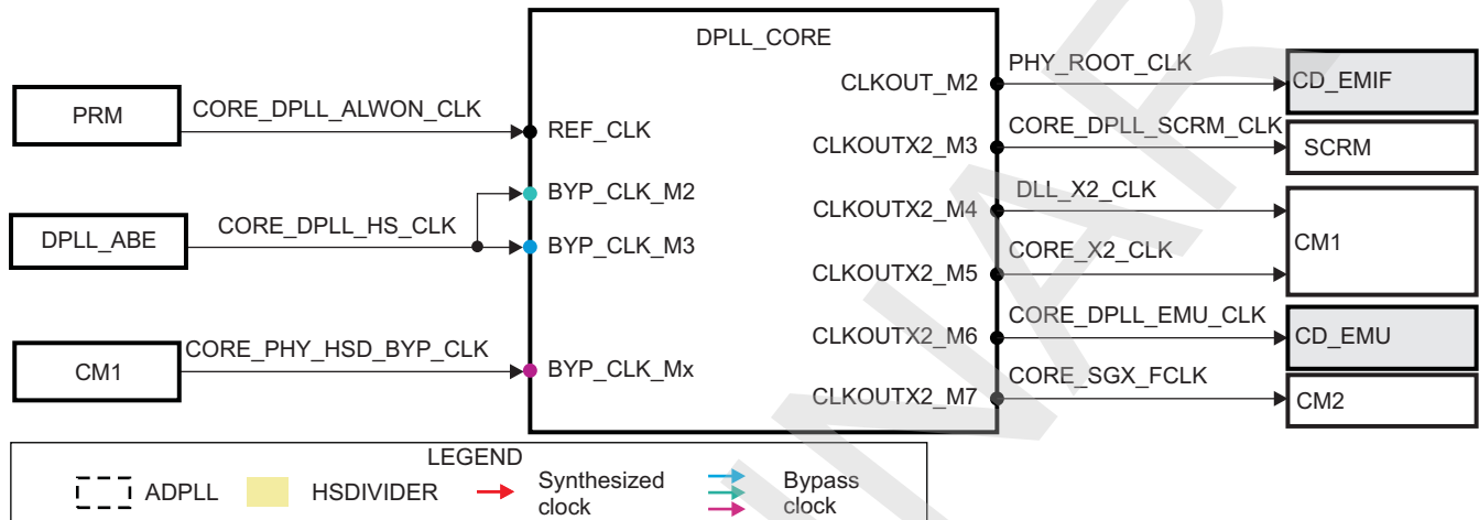
Figure 3-42. DPLL_CORE Overview
