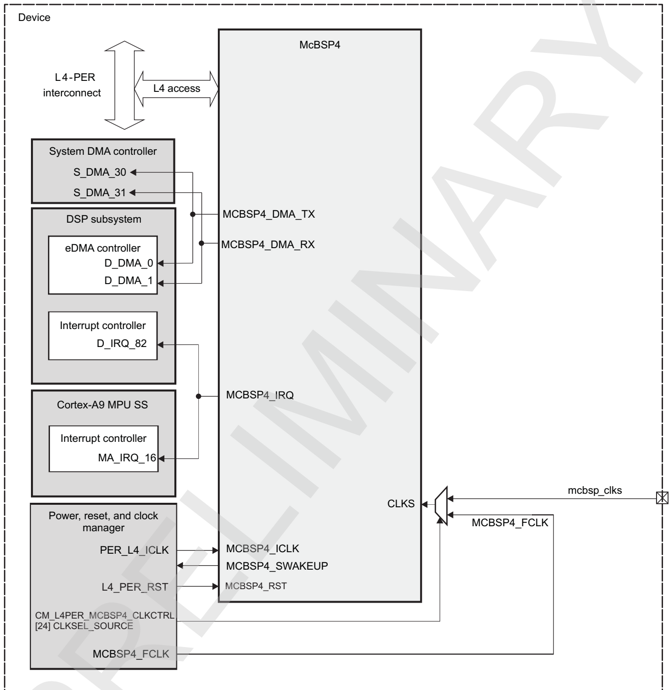
Figure 23-127. McBSP4 Integration
