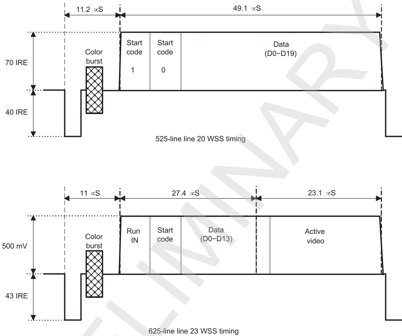
Figure 10-182. WSS Timing
