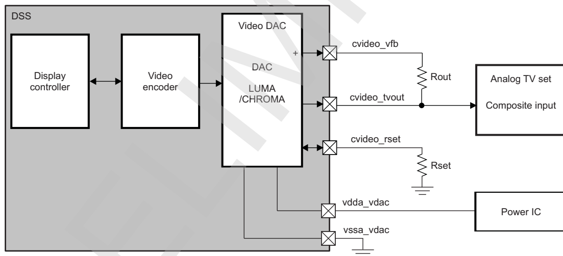
Figure 10-176. Video Encoder Environment, DC-Coupling
