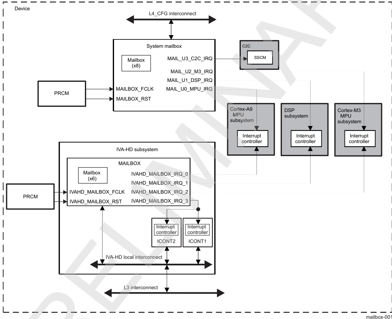
Figure 19-1. Mailbox Overview
