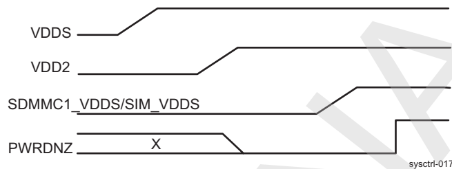
Figure 18-13. VDDS Ramps Up Before VDD2
