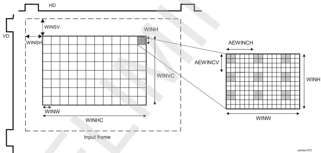
Figure 8-178. ISS ISP H3A AE/AWB Window Configurations
