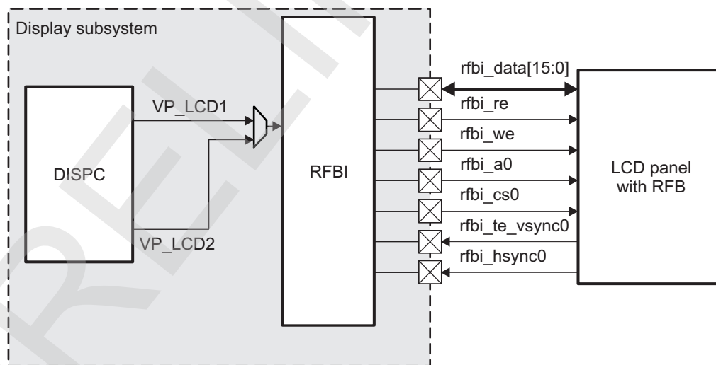
Figure 10-159. RFBI LCD Support Interface
