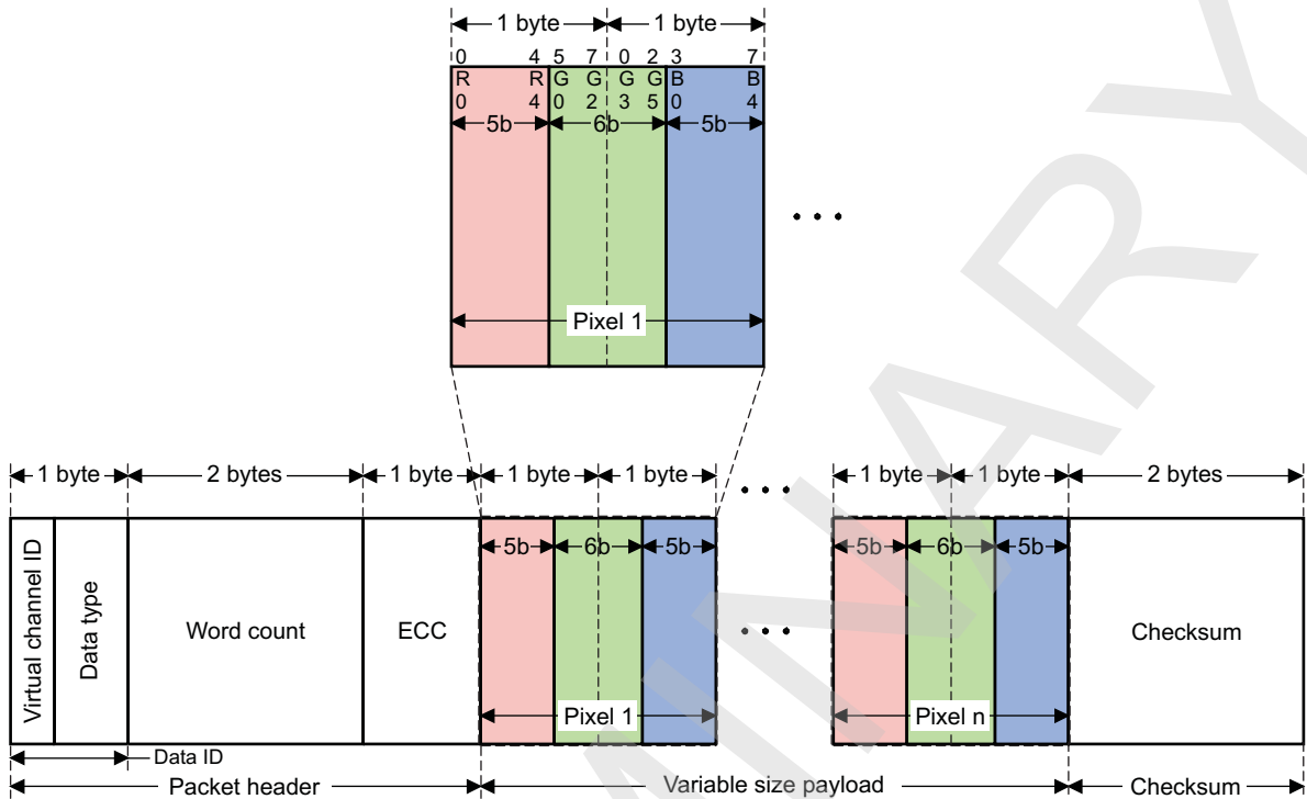
Figure 10-118. 16-bpp RGB Color Format, Long Packet (Video Mode)
