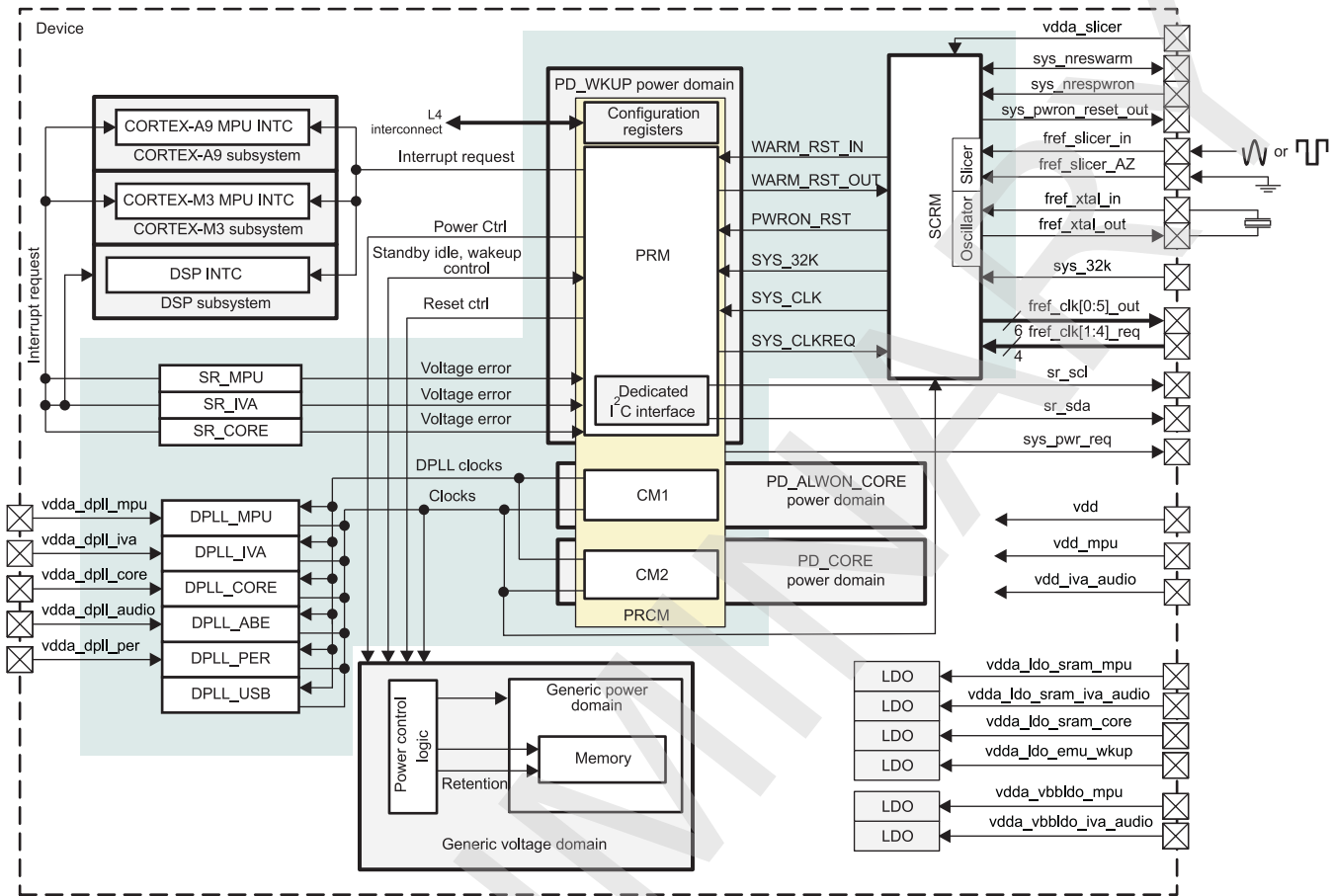
Figure 3-18. PMFW Overview
