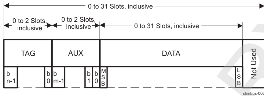
Figure 23-211. Segment Organization
