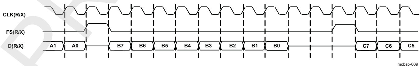
Figure 23-117. Serial Data Formats
