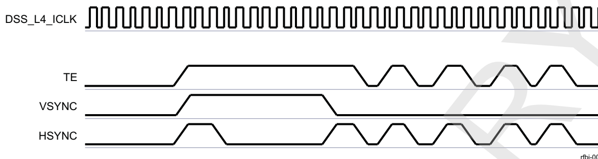
Figure 10-160. External Generation of TE Signal Based on Logical OR Operation Between HSYNC and VSYNC (Active-High)
