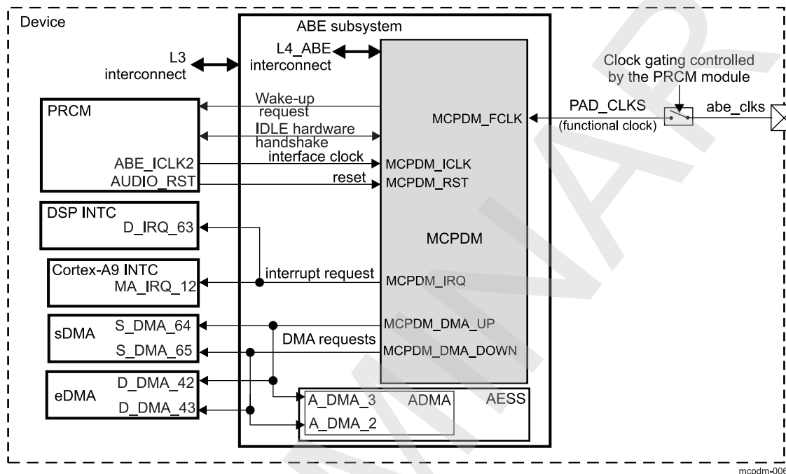
Figure 23-165. McPDM Integration
