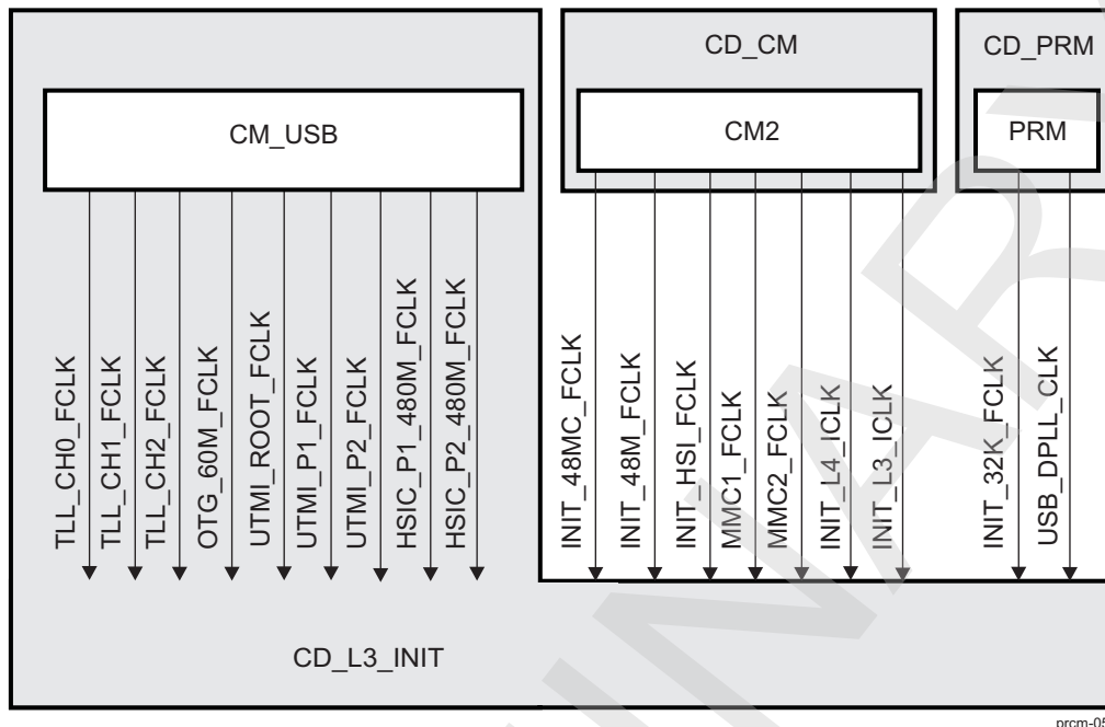
Figure 3-53. CD_L3_INIT Overview
