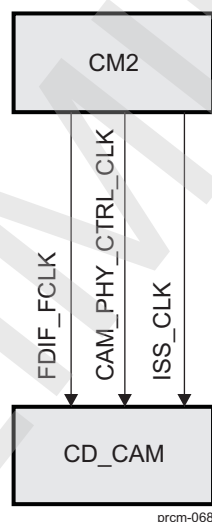
Figure 3-66. CD_CAM Overview
