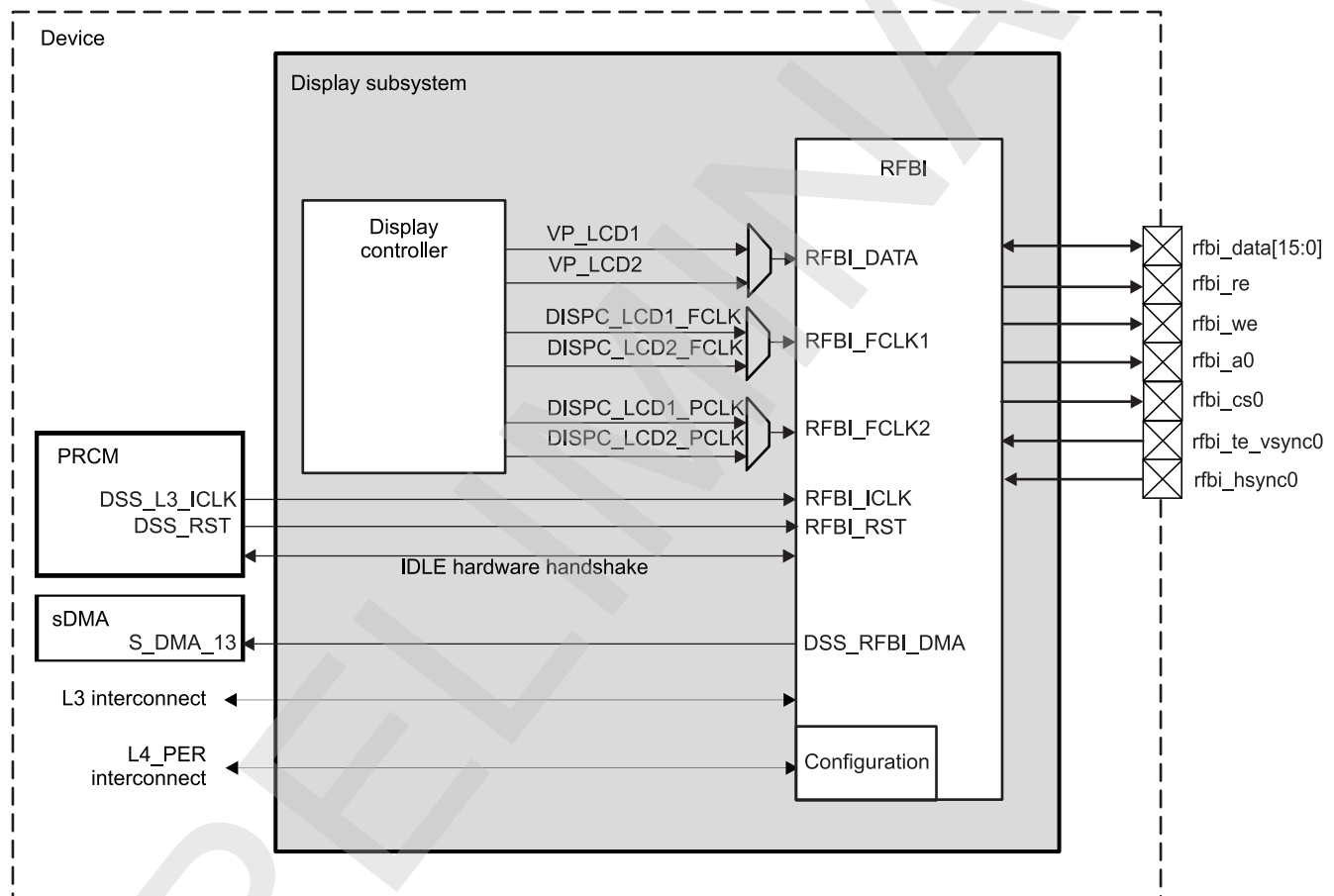
Figure 10-158. RFBI Highlight
