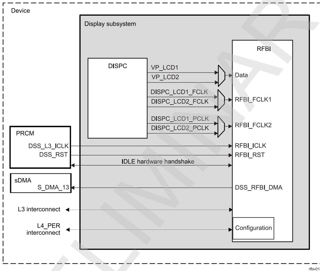
Figure 10-164. RFBI Integration
