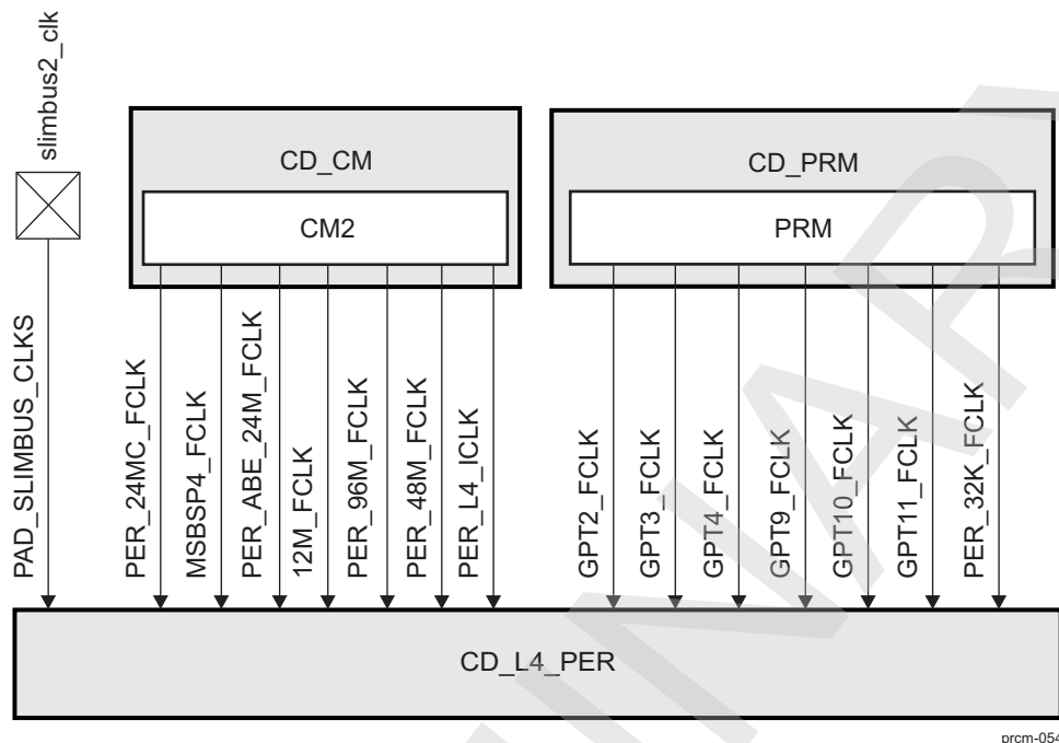
Figure 3-52. CD_L4_PER Overview
