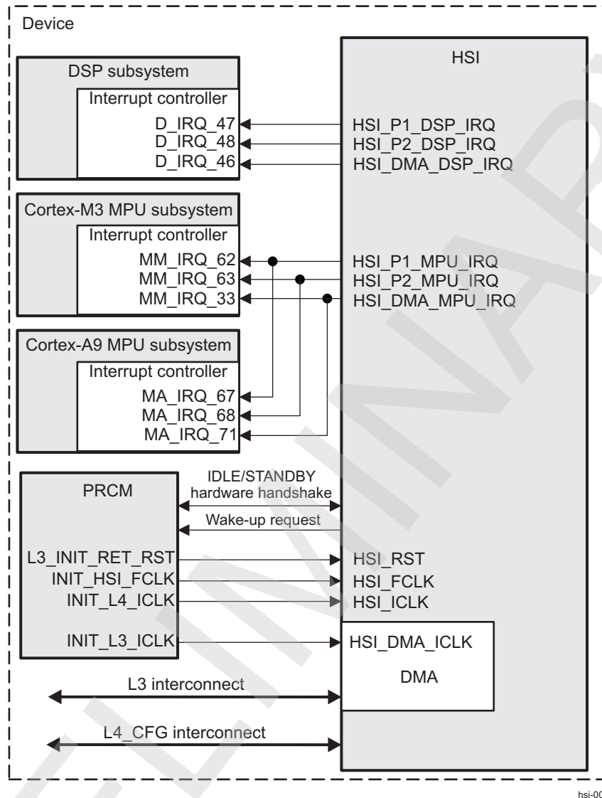
Figure 23-222. HSI Integration
