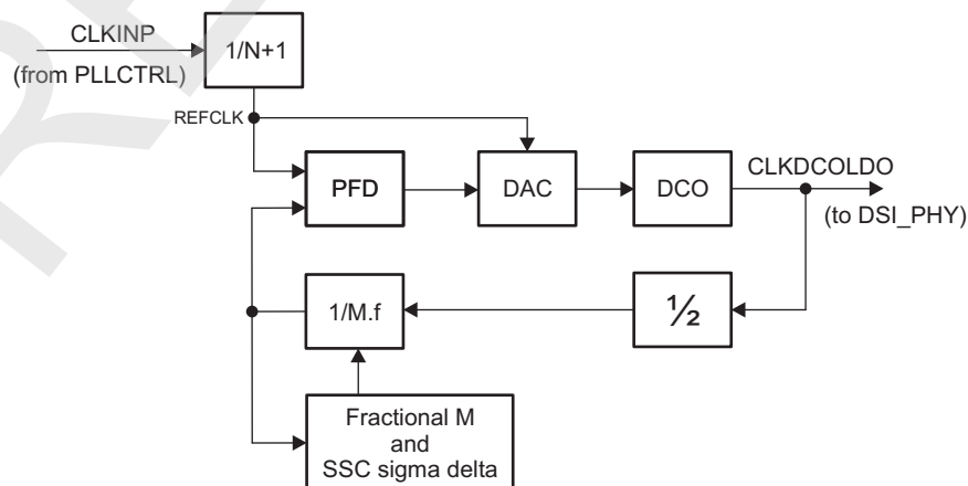
Figure 10-148. ADPLLM Functional Block Diagram
