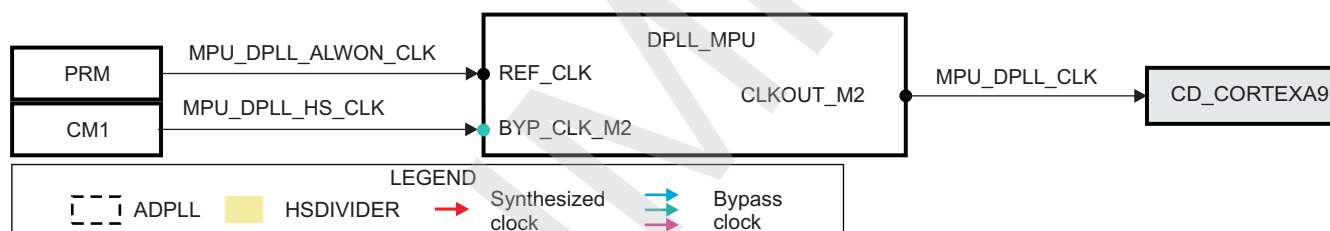
Figure 3-44. DPLL_MPU Overview
