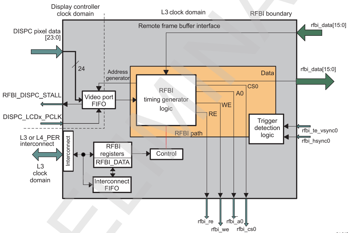
Figure 10-165. RFBI Architecture Overview
