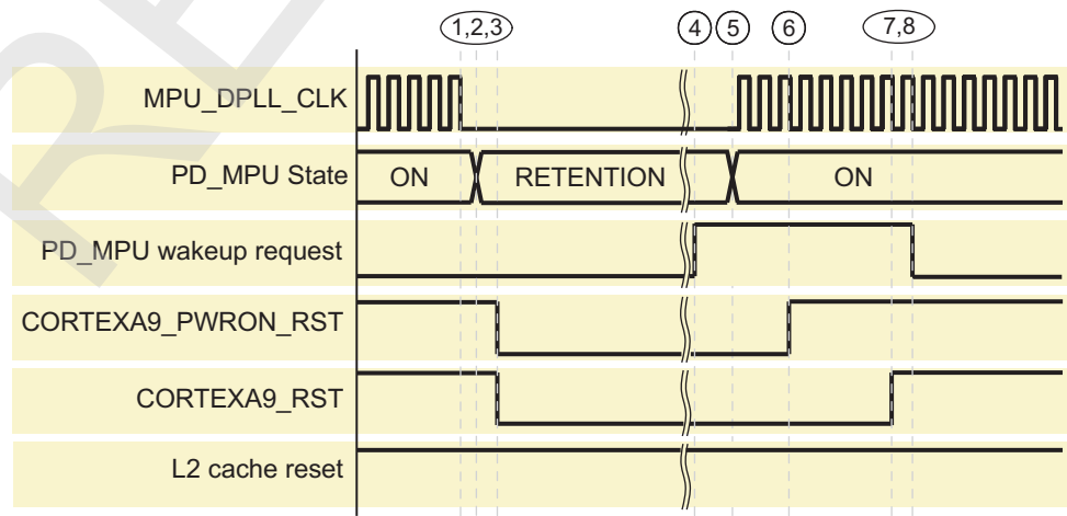
Figure 3-23. Cortex-A9 MPU Reset Sequence on Sleep and Wake-Up Transition
