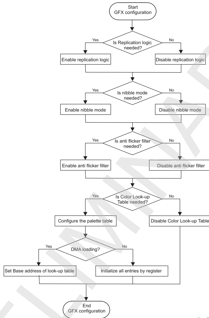
Figure 10-91. Video Pipeline Processing Configuration
