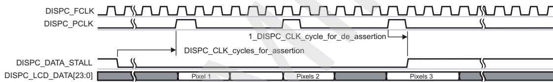
Figure 10-167. RFBI Data Stall Signal Diagram With Handshake With PCD=3
