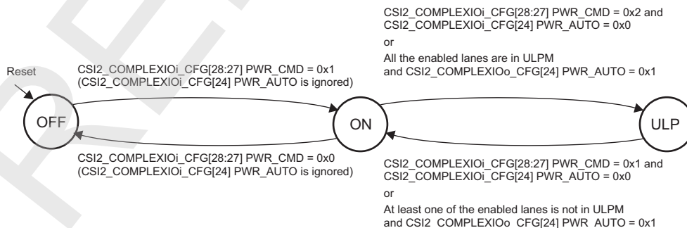
Figure 8-8. ISS CSI2 Complex I/O Power FSM
