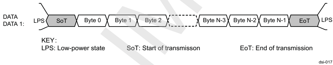
Figure 10-111. One-Data Lane Configuration
