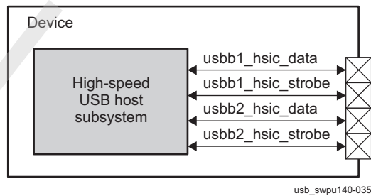
Figure 23-253. HSIC Interface
