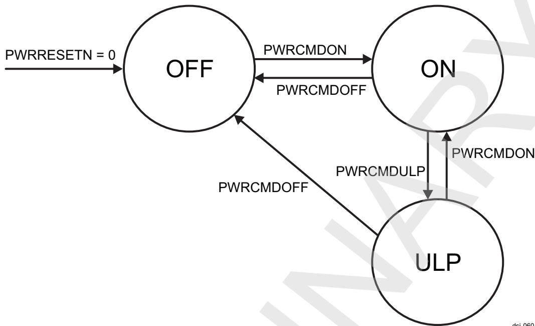
Figure 10-156. Power State Diagram
