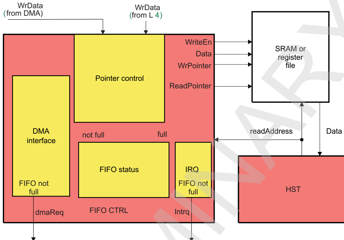
Figure 23-230. Transmission FIFO Architecture
