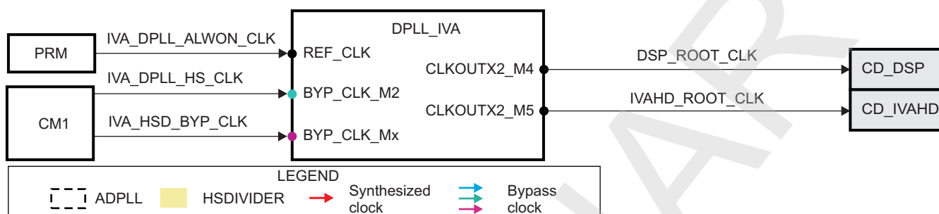
Figure 3-45. DPLL_IVA Overview
