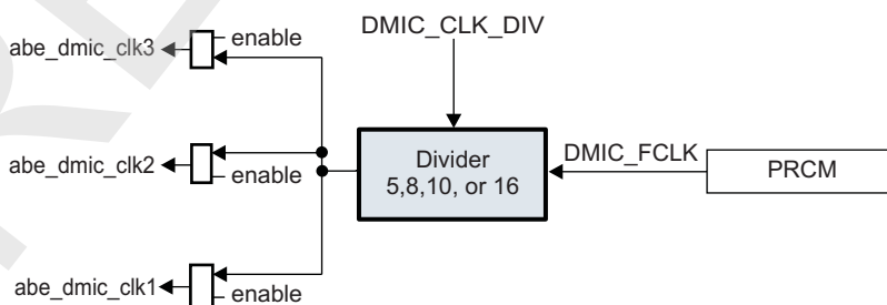
Figure 23-180. DMIC Clock Selection
