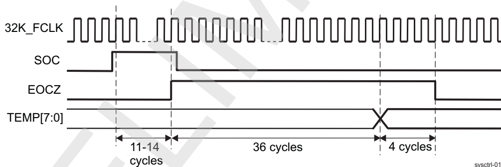
Figure 18-15. Single Conversion Mode (CONTCONV = 0)
