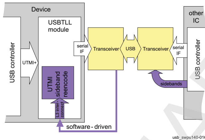
Figure 23-241. Serial Interface Sideband Integration - Transceiver Configuration
