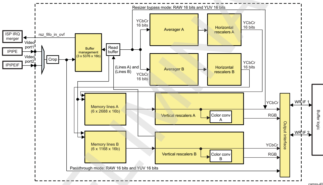
Figure 8-156. ISS ISP RSZ Top-Level Block Diagram
