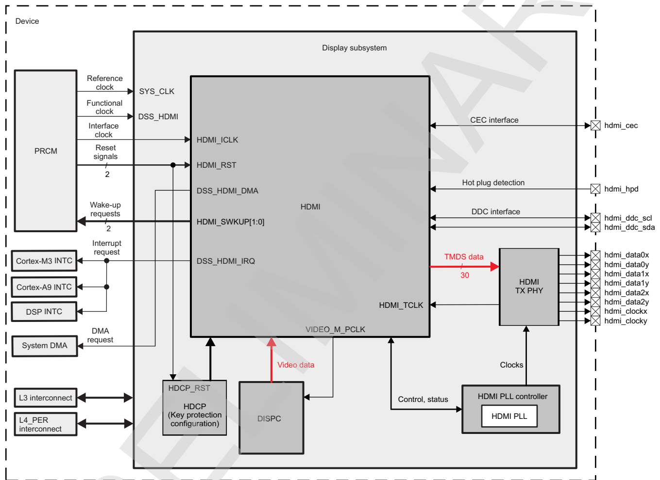
Figure 10-157. HDMI Overview
