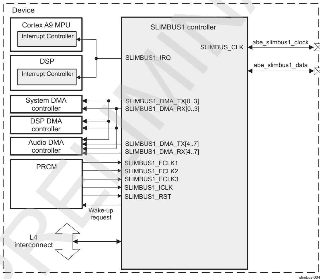
Figure 23-206. SLIMbus1 Highlight
