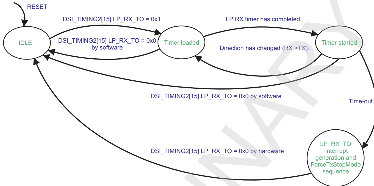
Figure 10-139. LP RX Timer FSM
