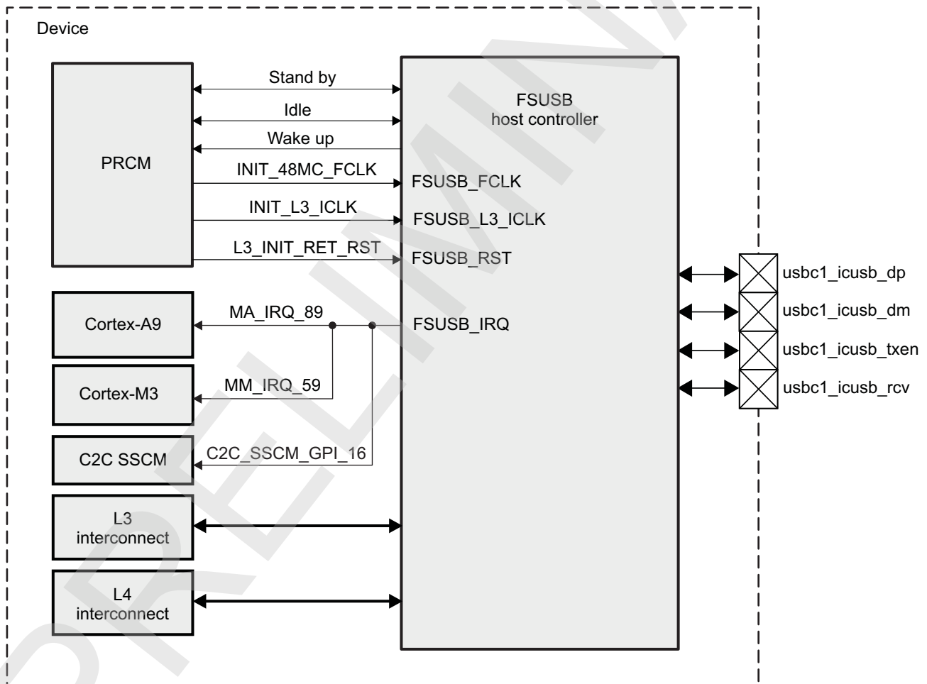
Figure 23-263. FSUSB Host Controller Overview
