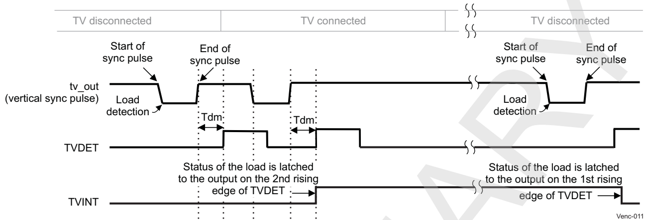
Figure 10-185. AC-Coupling TV Detect Waveforms for TV Connected and Disconnected
