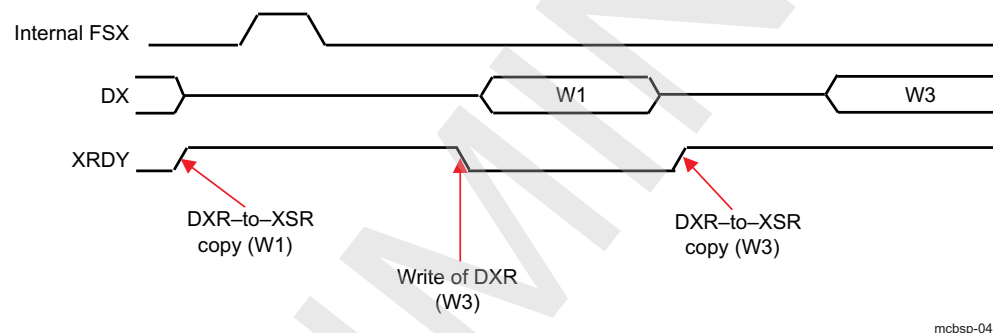
Figure 23-154. Activity on McBSP Pins When XMCM=0b01
