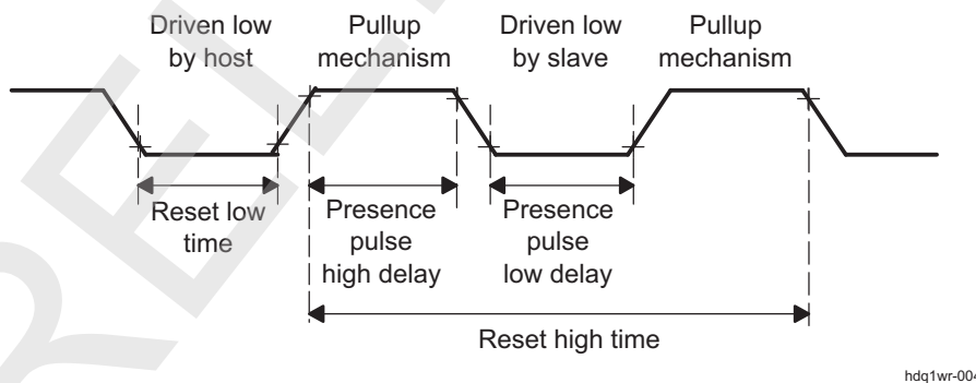
Figure 23-45. 1-Wire (SDQ) Reset Timing Diagram
