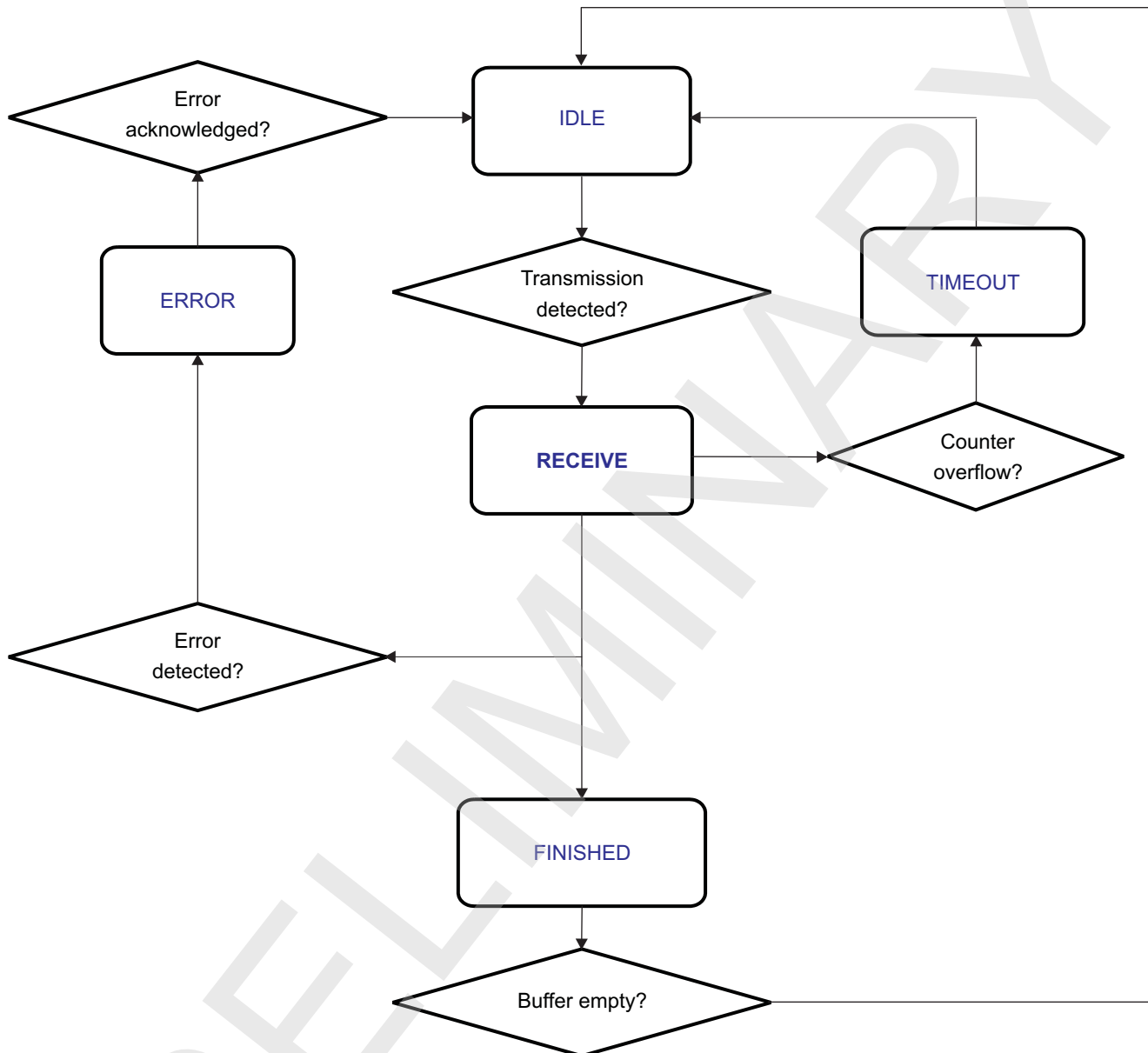
Figure 23-224. Receive FSM
