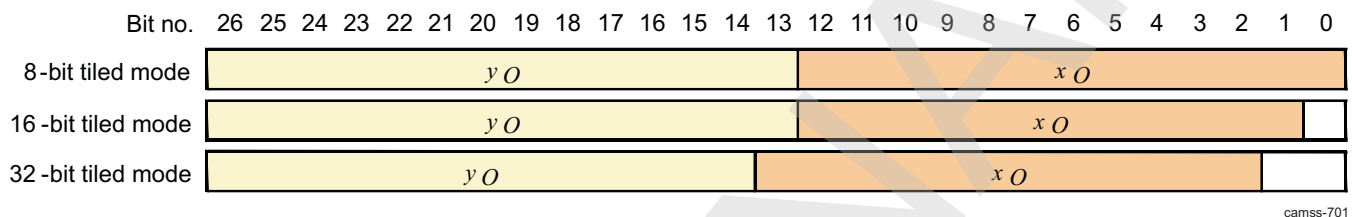
Figure 8-81. ISS BTE TILER Mode Addressing in 90- or 270-Degree Orientation
