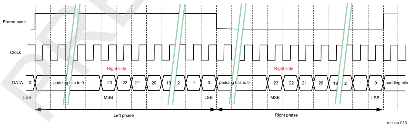
Figure 23-121. Right Justified Data Format; Word Width: 32 Bits; Data Length: 24 Bits
