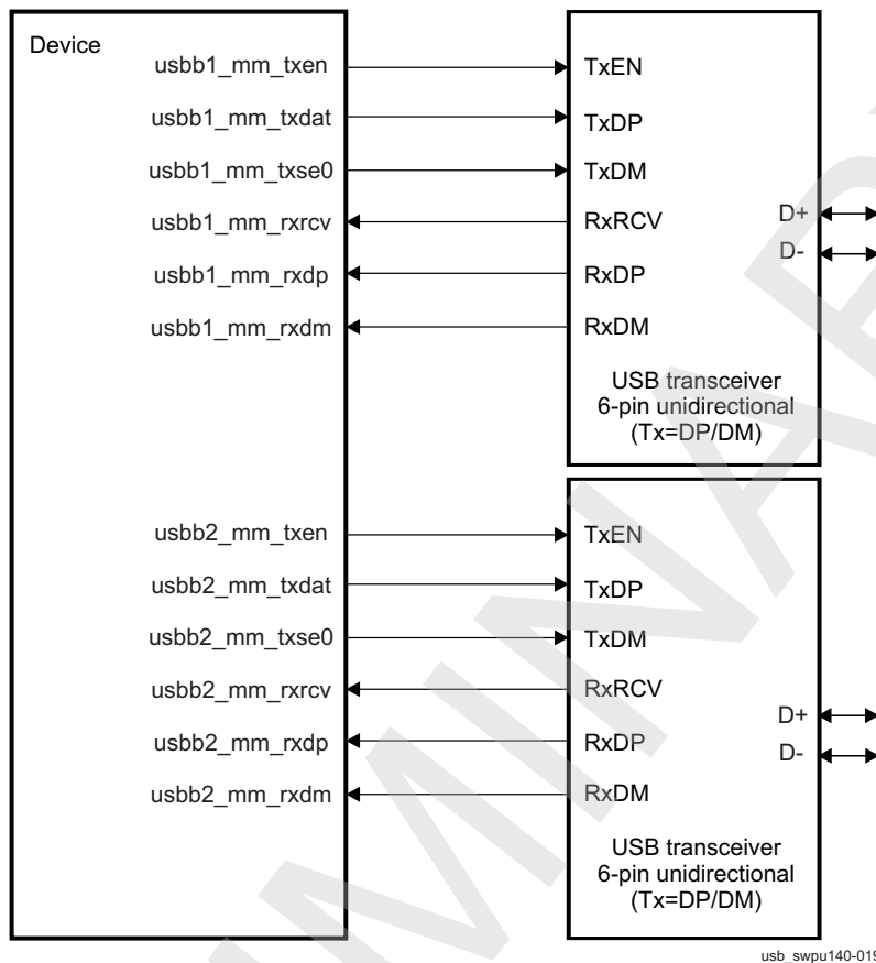
Figure 23-244. 6-Pin Unidirectional Using DP/DM Signaling
