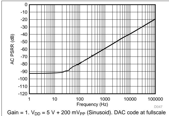
Figure 49. DAC Output AC PSRR vs Frequency
