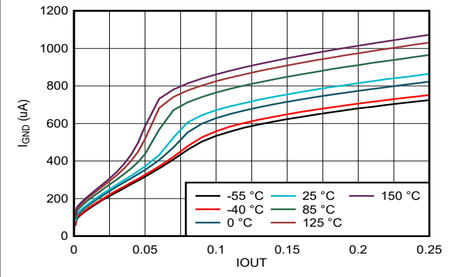
图 5-28. GND Pin vs Load Current for New Chip
