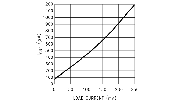
图 5-27. GND Pin vs Load Current for Legacy Chip
