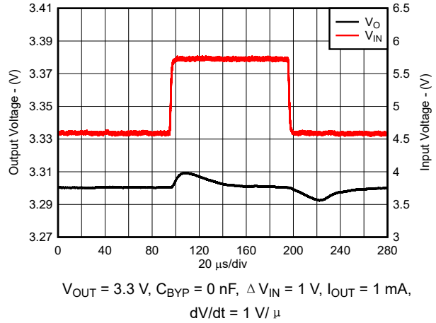
图 5-44. Line Transient Response for New Chip
