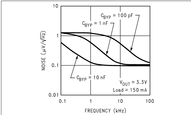
图 5-25. Output Noise Density for Legacy Chip
