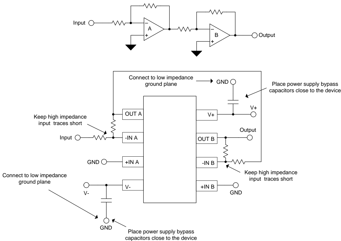
Figure 48. Layout Example
