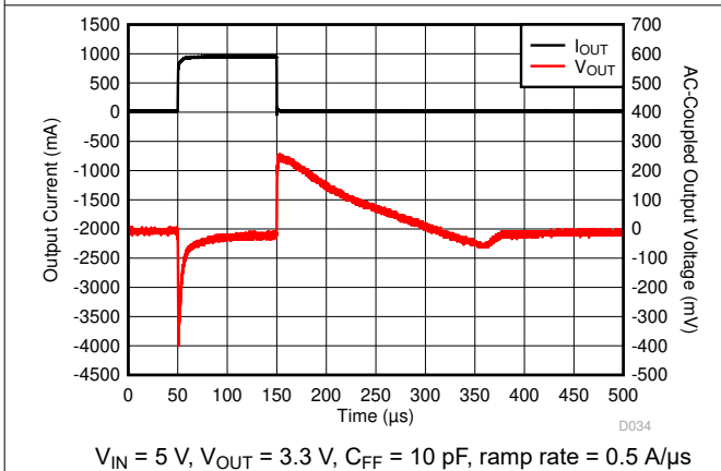
图 7-11. I_{OUT} Transient From 1 mA to 1 A
