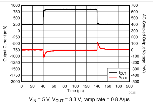
图 7-12. I_{OUT} Transient From 250 mA to 850 mA
