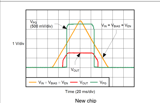
图 5-42. Power-Up, Power-Down
