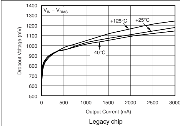
图 5-11. V_{BIAS} Dropout Voltage vs I_{OUT} and Temperature ( T_J )
