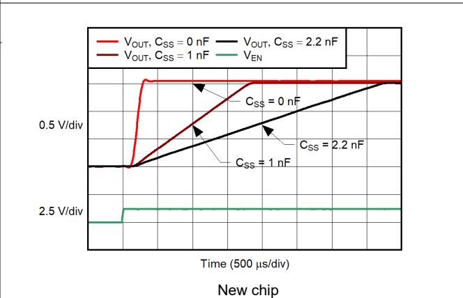
图 5-40. Turn-On Response
