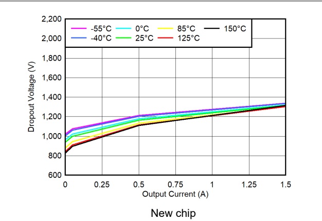
图 5-12. V_{BIAS} Dropout Voltage vs I_{OUT} and Temperature ( T_J )
