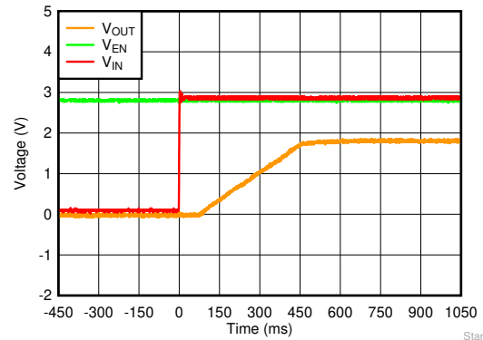
图 6-52. Startup With V_{EN} Before V_{IN}
