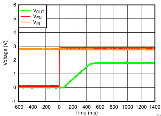
图 6-53. Startup With V_{EN} After V_{IN}
