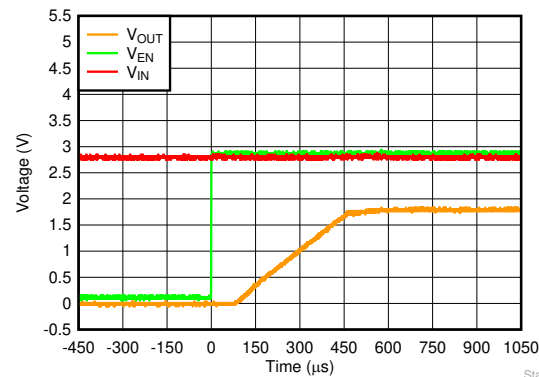
图 6-54. Startup With V_{EN} After V_{IN}
