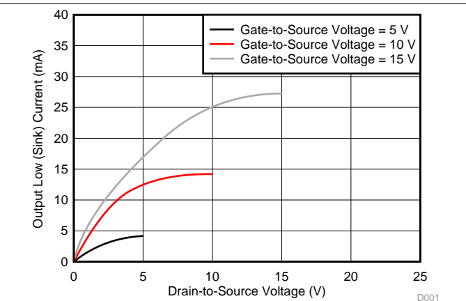
Figure 4. Typical Output Low (Sink) Current Characteristics
