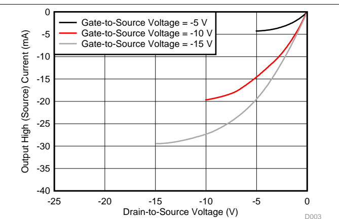
Figure 6. Typical Output High (Source) Current Characteristics
