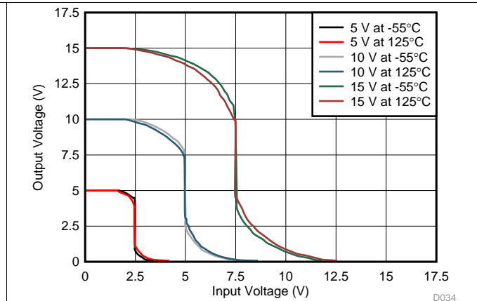
Figure 2. Typical Voltage Transfer Characteristics as a Function of Temperature
