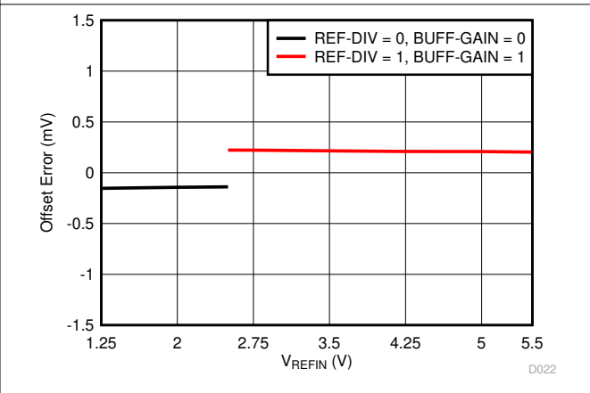
图 7-24. Offset Error vs Reference Voltage
