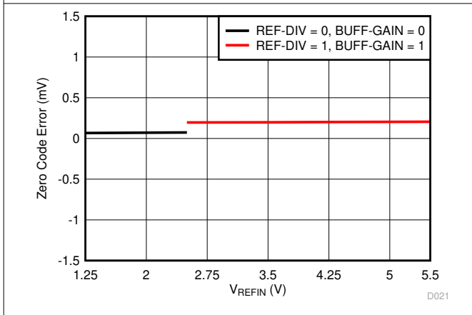
图 7-23. Zero Code Error vs Reference Voltage
