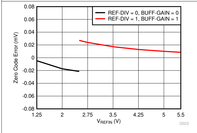
图 7-25. Gain Error vs Reference Voltage
