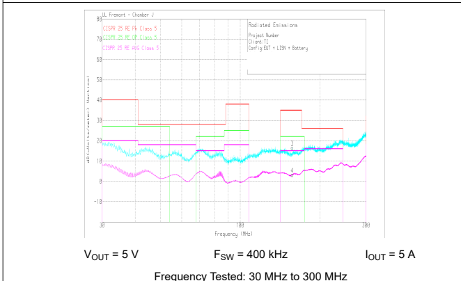
图 9-57. Radiated EMI Bicon Vertical versus CISPR25 Limits
