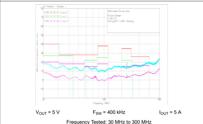
图 9-58. Radiated EMI Bicon Horizontal versus CISPR25 Limits
