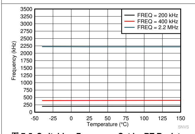
图 7-5. Switching Frequency Set by RT Resistor
