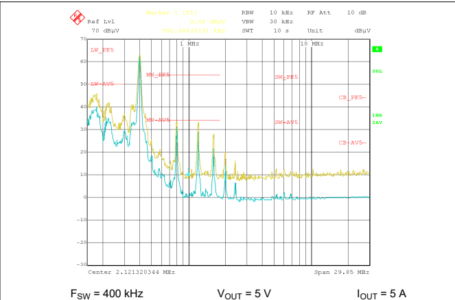
图 9-54. Conducted EMI versus CISPR25 Limits (Yellow: Peak Signal, Blue: Average Signal)
