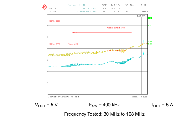
图 9-55. Conducted EMI versus CISPR25 Limits (Yellow: Peak Signal, Blue: Average Signal)
