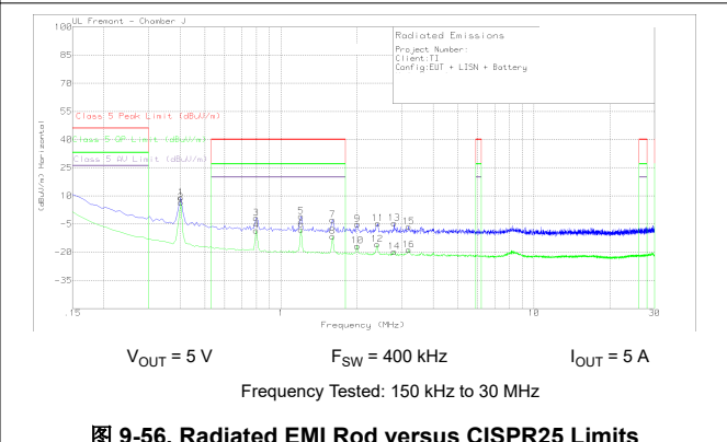
图 9-56. Radiated EMI Rod versus CISPR25 Limits
