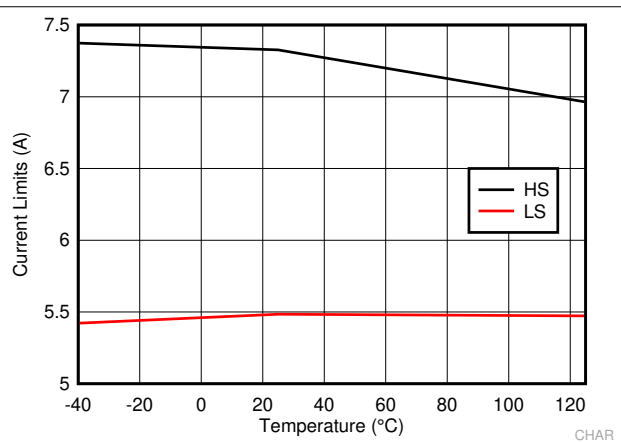
图 7-4. LM73605-Q1 High-Side and Low-Side Current Limits
