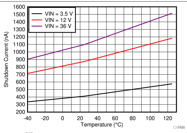
图 7-2. Shutdown Quiescent Current
