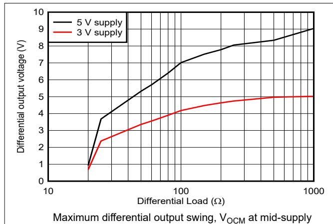
图 7-21. Differential Output Voltage vs Rload
