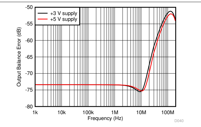
Single-ended input to differential output, gain of 2 (see 图 8-1), simulated with 1% resistor, worst-case mismatch
