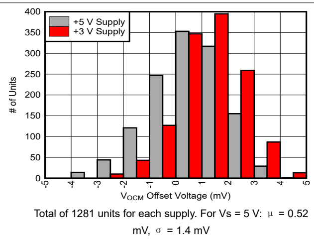
图 7-24. Common-Mode Output Offset from Driven V_{\text{OCM}}
