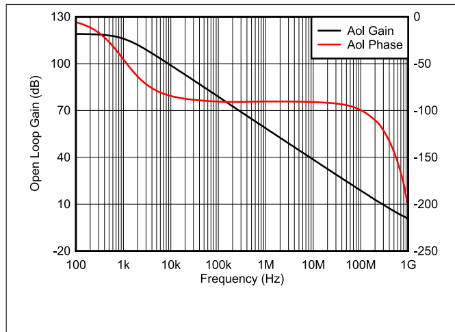
图 7-9. Main Amplifier Differential Open-Loop Gain and Phase vs Frequency
