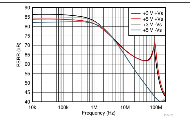
Single-ended to differential, gain of 2 (see 图 8-1) PSRR simulated to differential output
