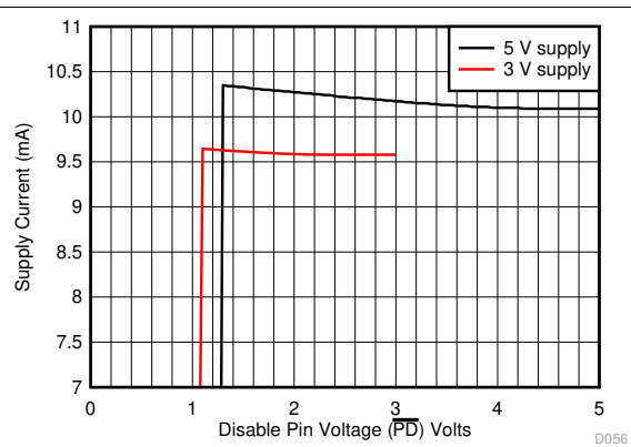
图 7-22. Supply Current vs PD Voltage
