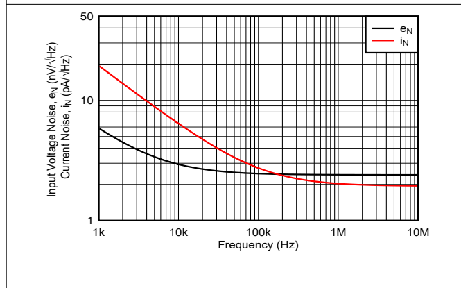
图 7-11. Input Spot Noise Over Frequency
