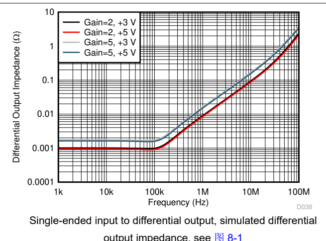
图 7-10. Closed-Loop Output Impedance
