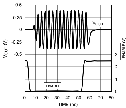
Figure 13. SHUTDOWN Switching
