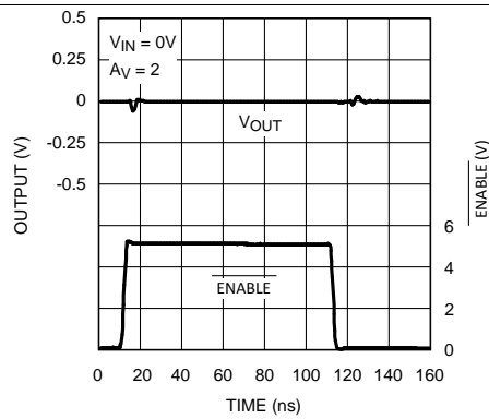
Figure 14. Shutdown Glitch
