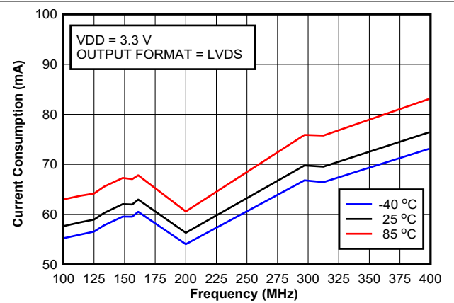
图 6-14. Current Consumption vs Frequency (LVDS, 3.3 V)
