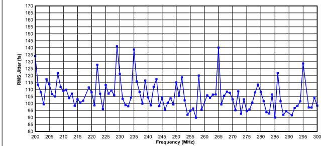
图 6-17. RMS Jitter vs Frequency (200 MHz to 300 MHz) for LVPECL, HCSL; TYPICAL 3.3 V, 25 °C
