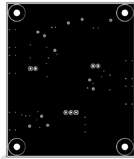
图 9-8. PCB Layout Example From LMK6 EVM - GND Layer 1
