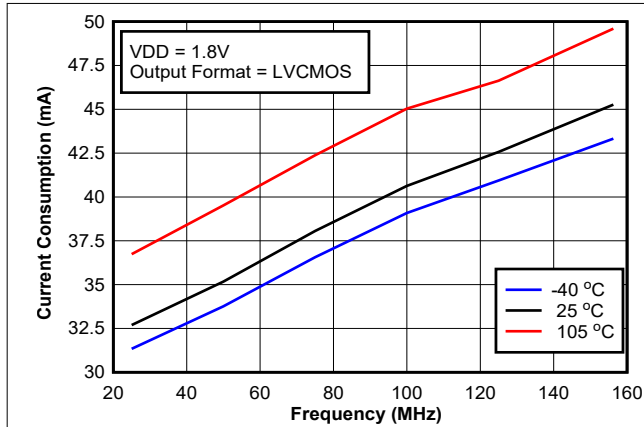
图 6-3. Current Consumption vs Frequency (LVCMOS, 1.8 V)
