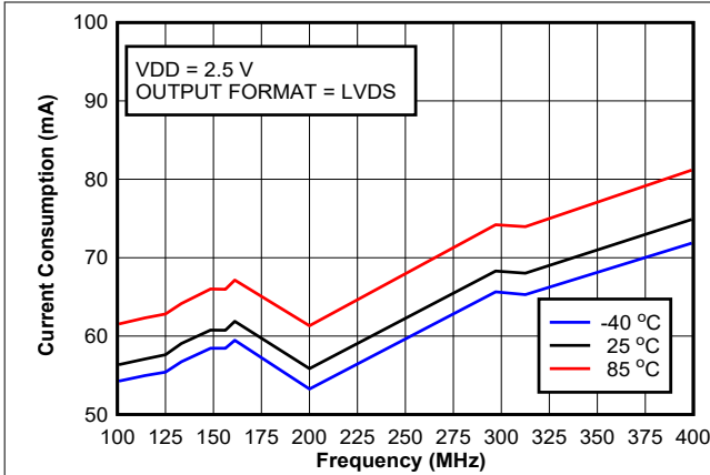
图 6-13. Current Consumption vs Frequency (LVDS, 2.5 V)
