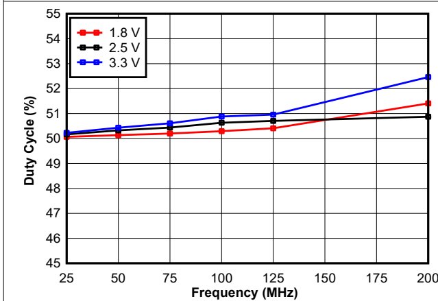
图 6-25. Duty Cycle (%) vs Frequency vs Power Supply; 25°C
