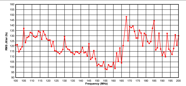
图 6-16. RMS Jitter vs Frequency (100 MHz to 200 MHz) for LVDS; TYPICAL 3.3 V, 25 °C
