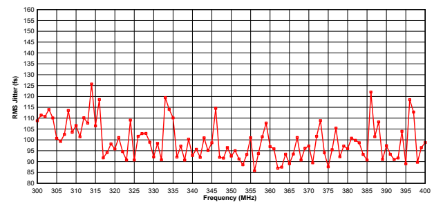
图 6-20. RMS Jitter vs Frequency (300 MHz to 400 MHz) for LVDS; TYPICAL 3.3 V, 25 °C
