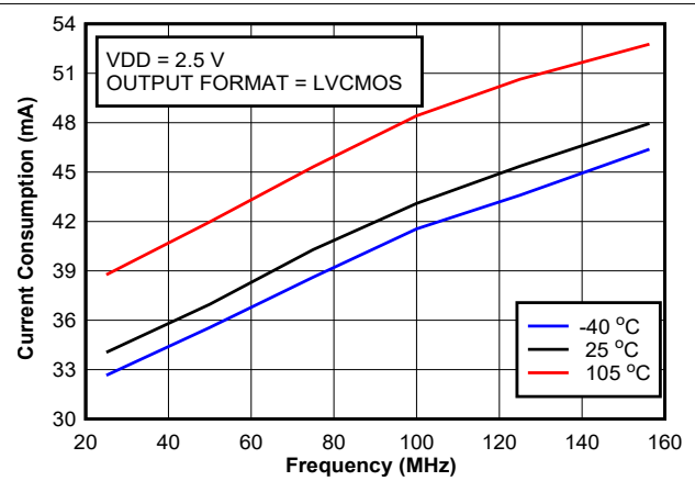
图 6-4. Current Consumption vs Frequency (LVCMOS, 2.5 V)
