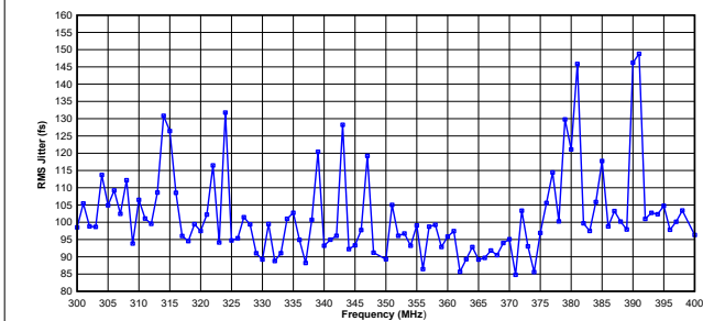
图 6-19. RMS Jitter vs Frequency (300 MHz to 400 MHz) for LVPECL, HCSL; TYPICAL 3.3 V, 25 °C
