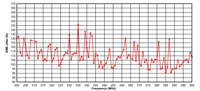
图 6-18. RMS Jitter vs Frequency (200 MHz to 300 MHz) for LVDS; TYPICAL 3.3 V, 25 °C
