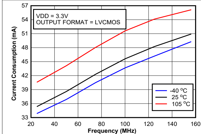
图 6-5. Current Consumption vs Frequency (LVCMOS, 3.3 V)
