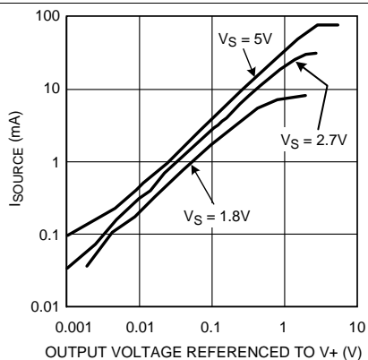
Figure 5. Sourcing Current vs Output Voltage
