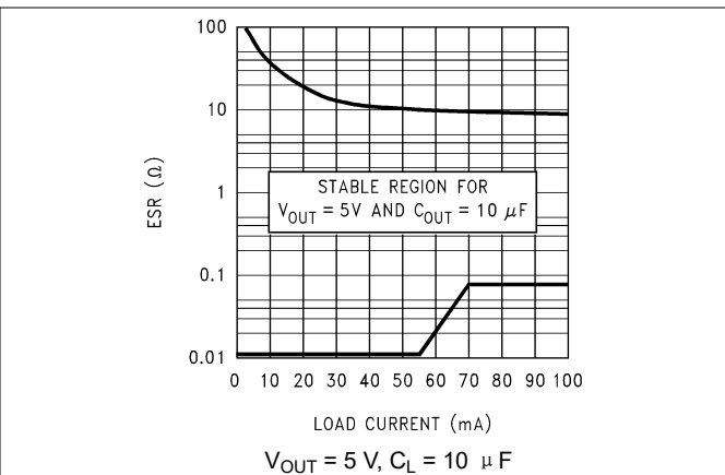
图 7-4. 5-V, 10- \mu\text{F} ESR Curves (Legacy Chip)
