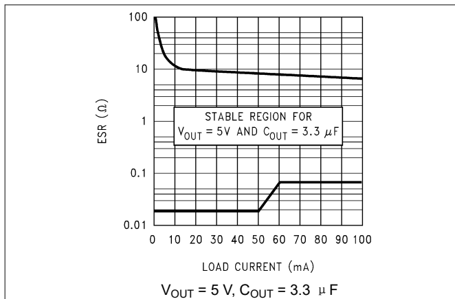
图 7-3. 5-V, 3.3- \mu\text{F} ESR Curves (Legacy Chip)
