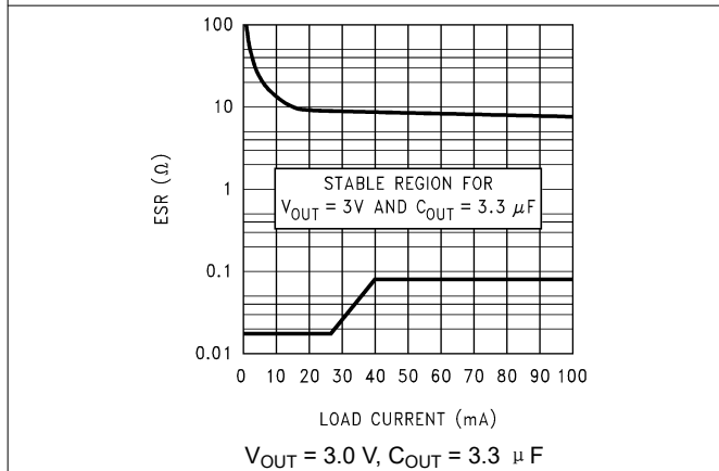
图 7-5. 3.0-V, 3.3- \mu\text{F} ESR Curves (Legacy Chip)
