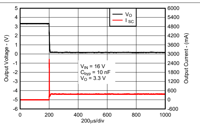
图 6-10. Short-Circuit Current vs Time for New Chip
