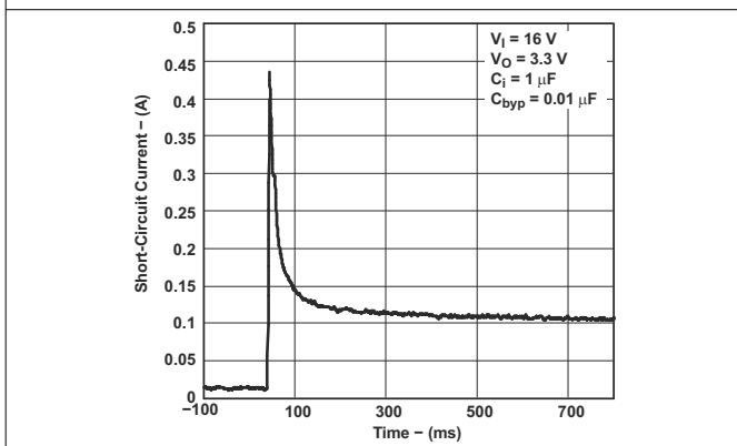
图 6-9. Short-Circuit Current vs Time for Legacy Chip
