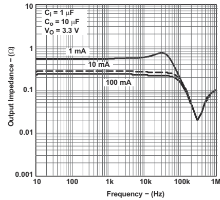
图 6-26. Output Impedance vs Frequency for Legacy Chip
