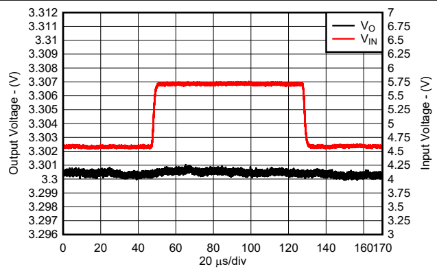
图 8-16. Line Transient Response for New Chip
