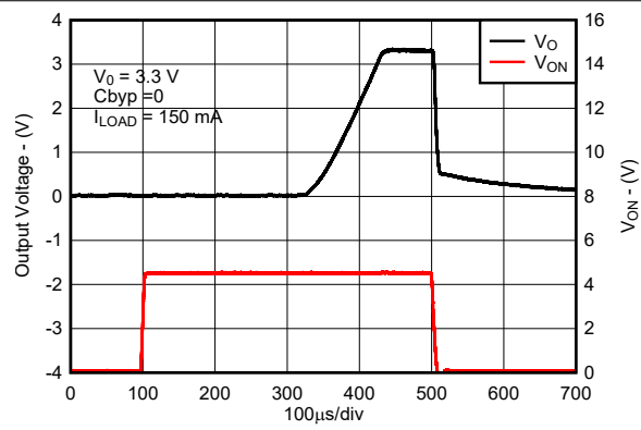
图 8-18. Turn-On Time for New Chip
