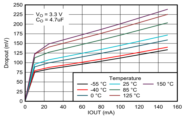
图 6-4. Dropout Voltage vs Temperature for Legacy Chip
