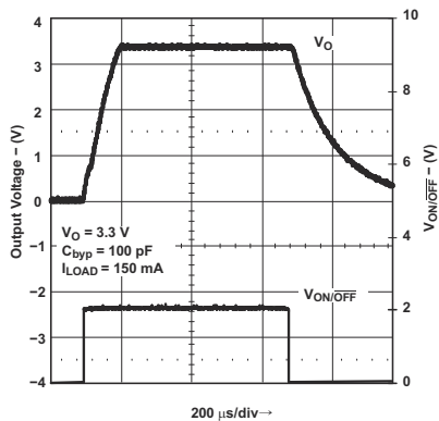
图 8-17. Turn-On Time for Legacy Chip
