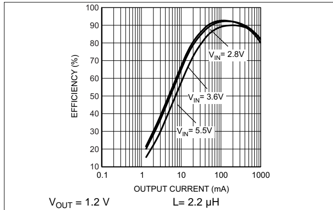
Figure 14. Efficiency vs Output Current (Forced PWM Mode)
