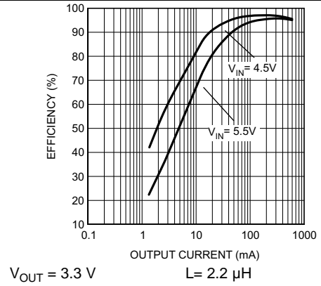
Figure 19. Efficiency vs Output Current (Forced PWM Mode)
