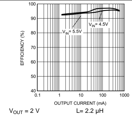
Figure 21. Efficiency vs Output Current (PWM-to-PFM Mode)
