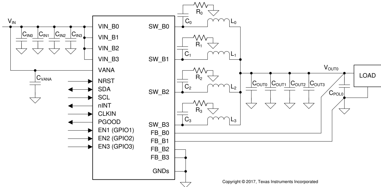
图 8-1. 4-Phase Configuration
