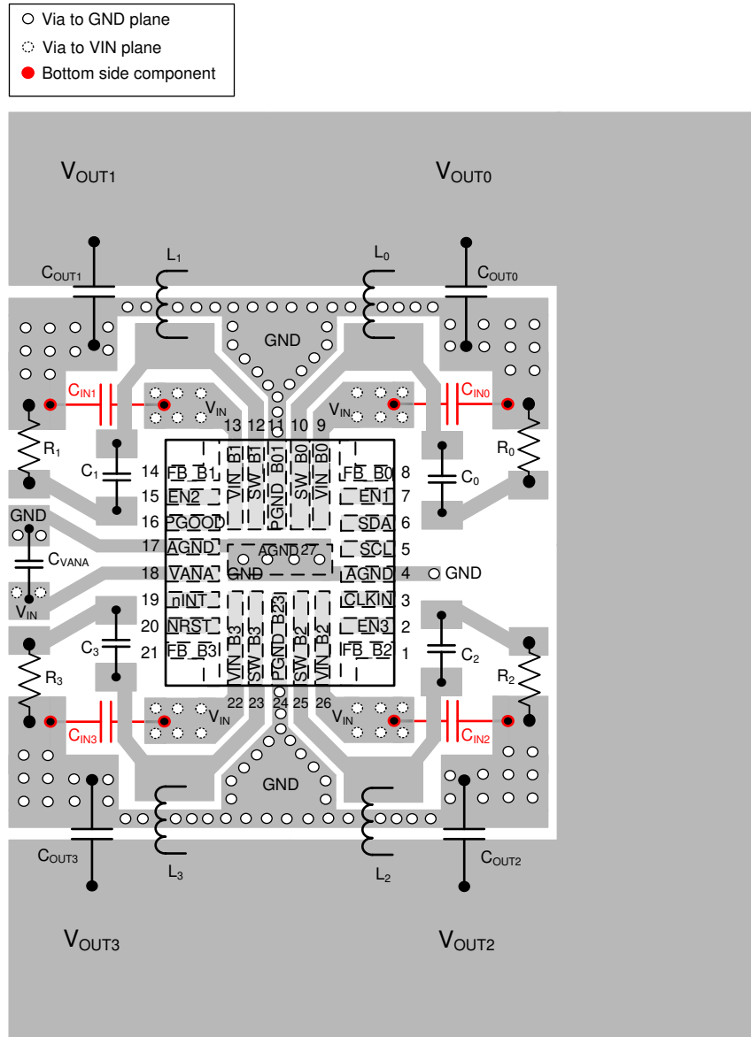
图 10-1. Board Layout
