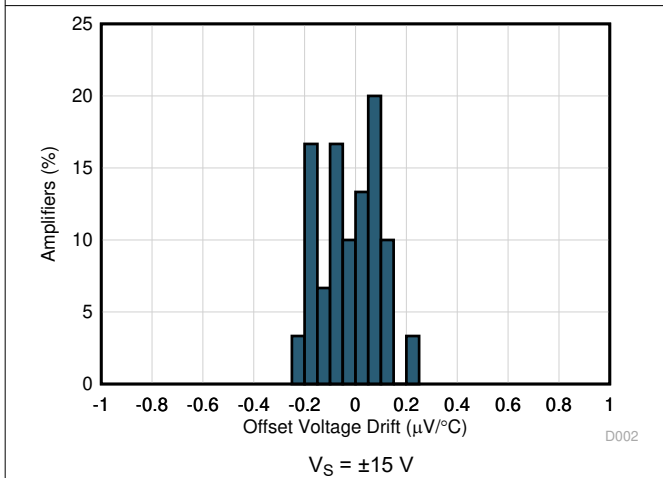
图 6-15. Input Offset Voltage Drift Histogram
