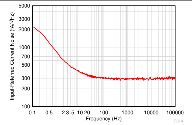
图 6-2. Current Noise vs Frequency
