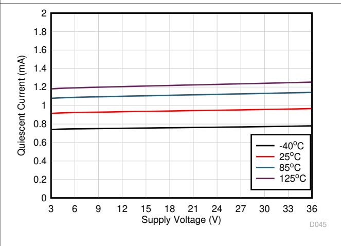
图 6-18. Quiescent Current vs Supply Voltage
