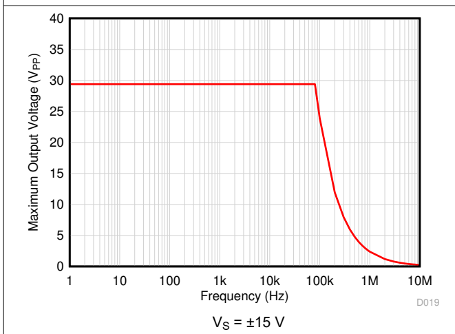
图 6-11. Maximum Output Voltage vs Frequency
