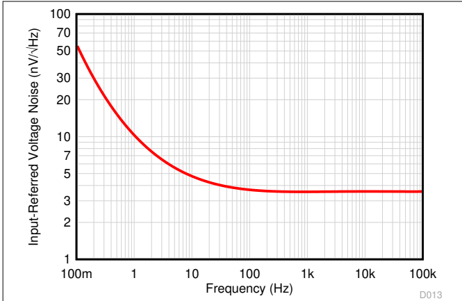
图 6-1. Input-Referred Voltage Noise vs Frequency
