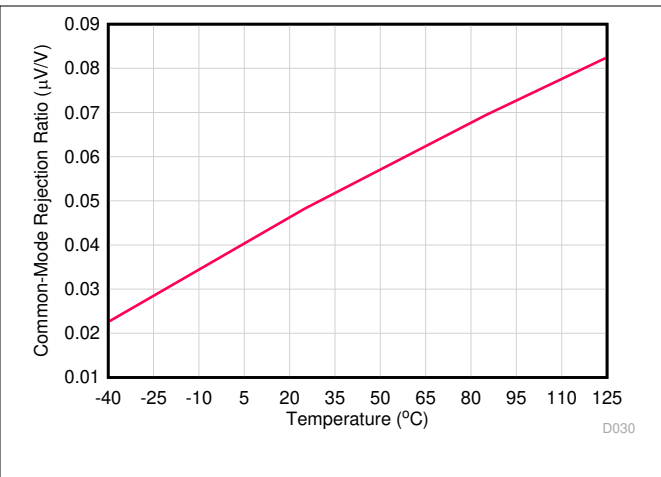
图 6-8. Common Mode Rejection Ratio vs Temperature
