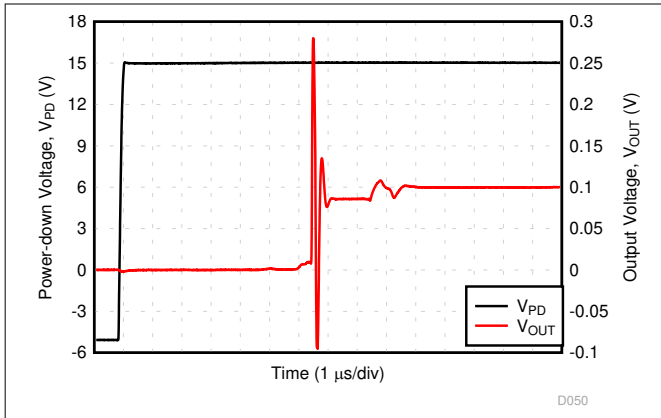
图 6-37. Power-Down Time (PD Low to High)
