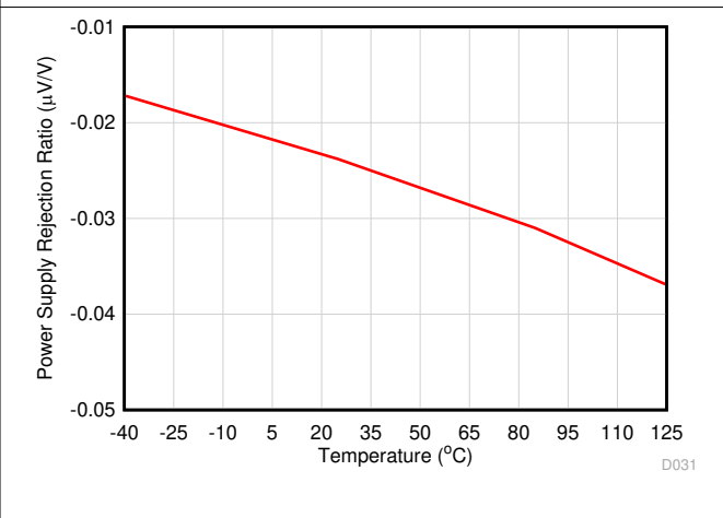
图 6-10. Power Supply Rejection Ratio vs Temperature
