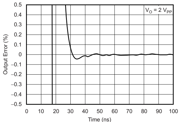
Figure 17. OUTPUT SETTLING TIME TO 0.1%
