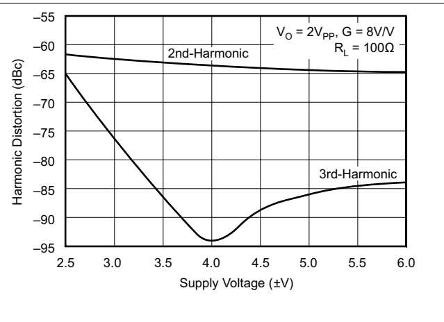
Figure 5-46. 10-MHz Harmonic Distortion vs Supply Voltage
