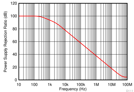
图 6-51. Power Supply Rejection Ratio vs Frequency
