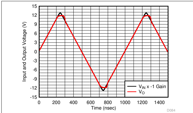
图 6-30. Output Overdrive Recovery
