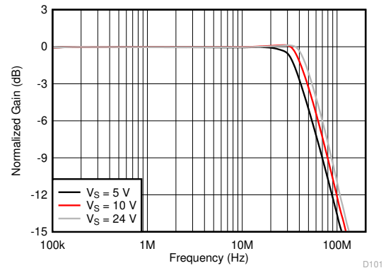
图 6-43. Large-Signal Response vs Supply Voltage
