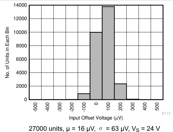
图 6-58. Input Offset Voltage Distribution
