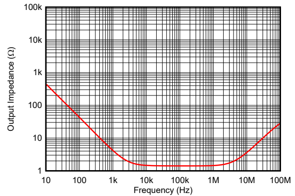
图 6-49. Open-Loop Output Impedance vs Frequency
