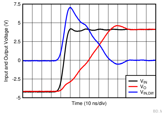
图 8-18. Large-Signal Transient Response Using the OPA810
