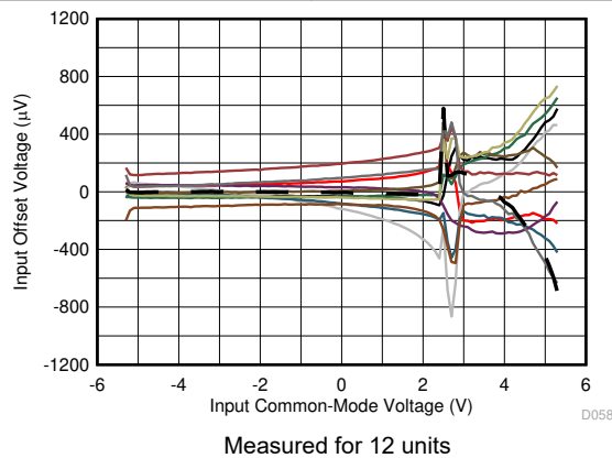
图 6-17. Input Offset Voltage vs Input Common-Mode Voltage
