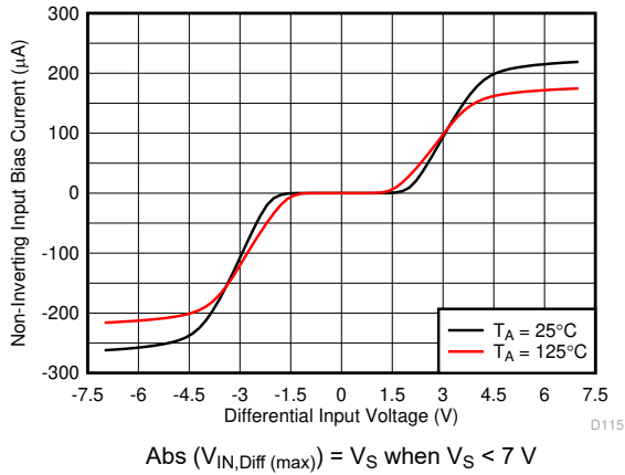
图 6-54. Input Bias Current vs Differential Input Voltage
