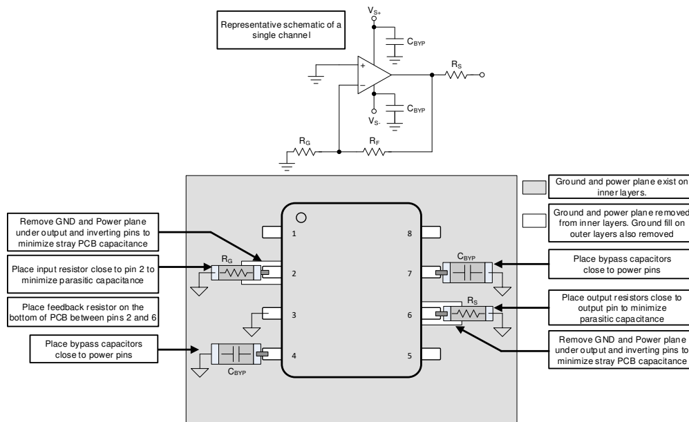
图 8-19. Layout Recommendation
