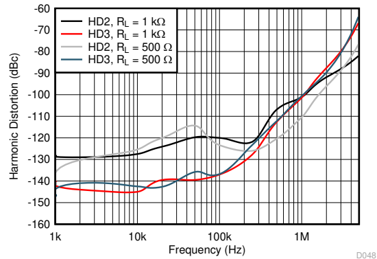
See 图 8-1, gain = 2 V/V
