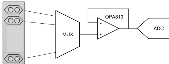
图 8-17. Multichannel Sensor Interface Using a Single Higher GBWP Amplifier
