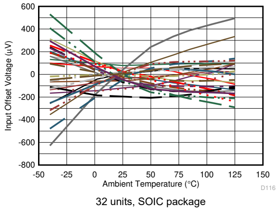
图 6-56. Input Offset Voltage vs Ambient Temperature
