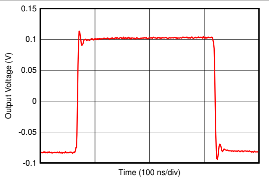
See 图 8-1, gain = 1 V/V, R_F = 0\ \Omega , C_L = 10\text{ pF}
