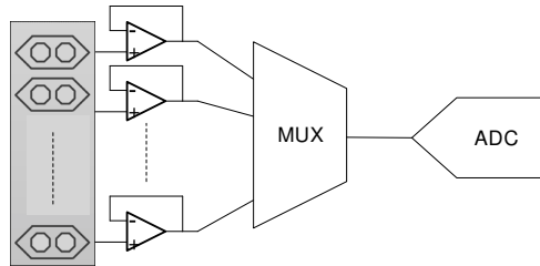
图 8-16. Multichannel Sensor Interface Using Multiple Amplifiers
