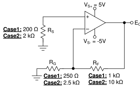
图 8-11. Comparing Noise Contributors for Two Cases with the Amplifier in a Noninverting Gain of 5 V/V
