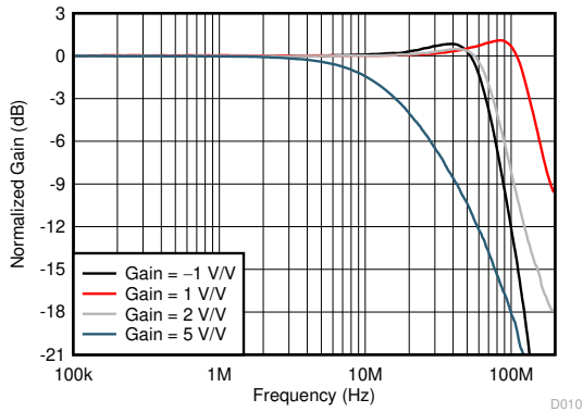
图 6-34. Small-Signal Response vs Gain
