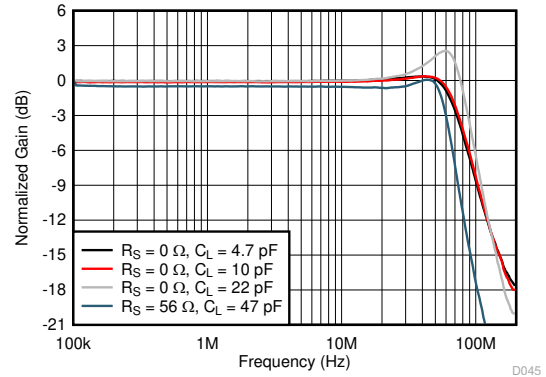
图 6-2. Small-Signal Frequency Response vs Output Load
