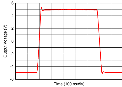
图 6-25. Large-Signal Transient Response
