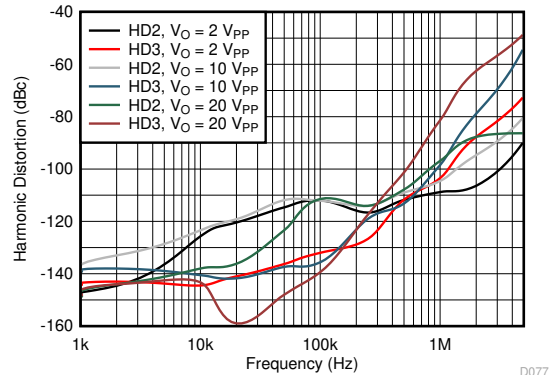
See 图 8-2, gain = -1 V/V
