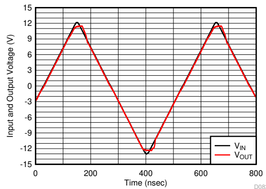
图 6-27. Large-Signal Transient Response
