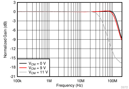
See 图 8-1, V_O = 20\text{ mV}_{PP} , gain = 1 V/V, C_L = 4.7\text{ pF} , R_F = 0\ \Omega
