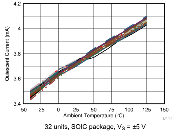
图 6-55. Quiescent Current vs Ambient Temperature
