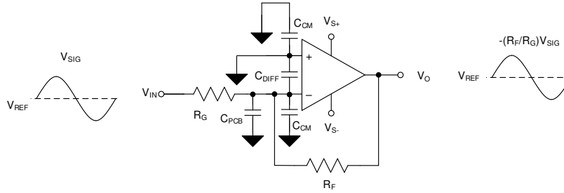
图 8-5. Inverting Amplifier With Input Capacitors
