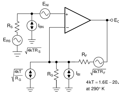
图 8-10. Operational Amplifier Noise Analysis Model
