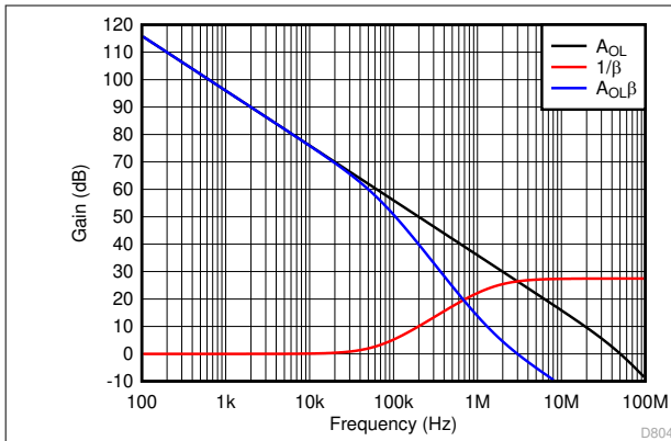
图 8-13. Loop-Gain Magnitude vs Frequency for the Transimpedance Amplifier Circuit of 图 8-12
