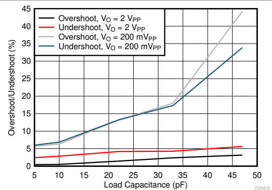
See 图 8-1, gain = 1 V/V, R_F = 0\ \Omega
