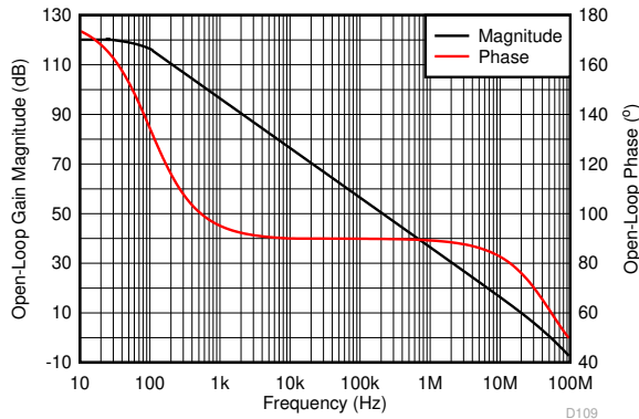
图 6-42. Open-Loop Gain and Phase vs Frequency
