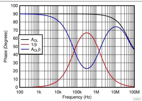
图 8-14. Loop-Gain Phase vs Frequency for the Transimpedance Amplifier Circuit of 图 8-12
