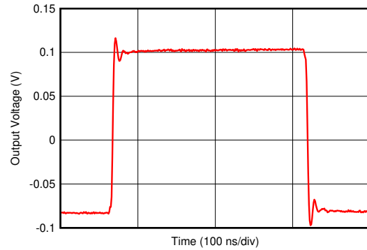
图 6-35. Small-Signal Transient Response
