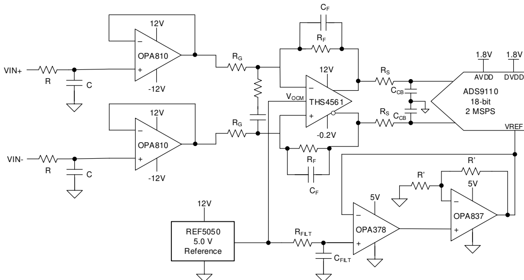
图 8-15. High-Z Input Data Acquisition Front-End
