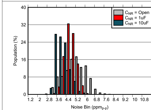
图 6-15. 0.1Hz to 10Hz Noise Distribution ( V_{REF} = 2.5\text{V} , C_L = 1\mu\text{F} , I_L = 0\text{mA} )
