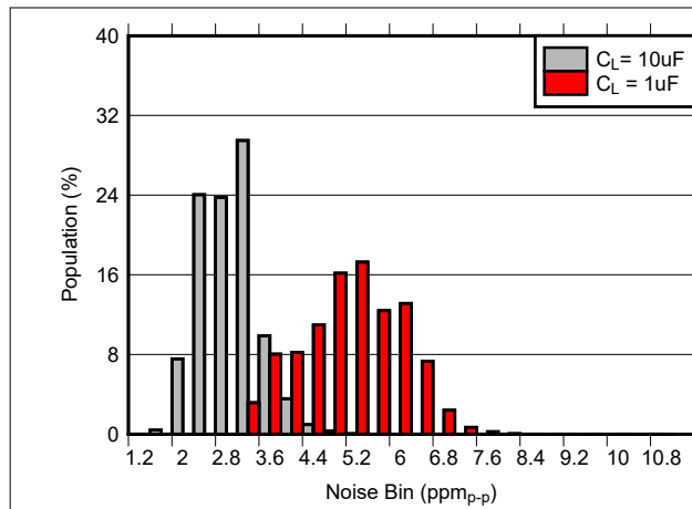
图 6-13. 0.1Hz to 10Hz Noise Distribution ( V_{REF} = 2.5\text{V} , C_{NR} = \text{Open} , I_L = 0\text{mA} )
