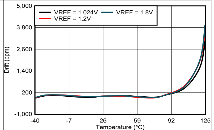
图 6-6. Output Voltage Drift vs Free-Air Temperature
