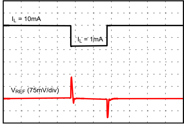
图 8-4. Load Transient Response 1\text{mA} to 10\text{mA} , C_L = 1\mu\text{F}
