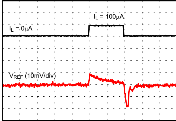
图 8-3. Load Transient Response 0\mu\text{A} to 100\mu\text{A} , C_L = 1\mu\text{F}
