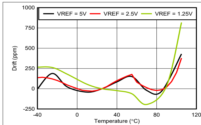
图 6-1. Output Voltage Drift vs Free-Air Temperature
