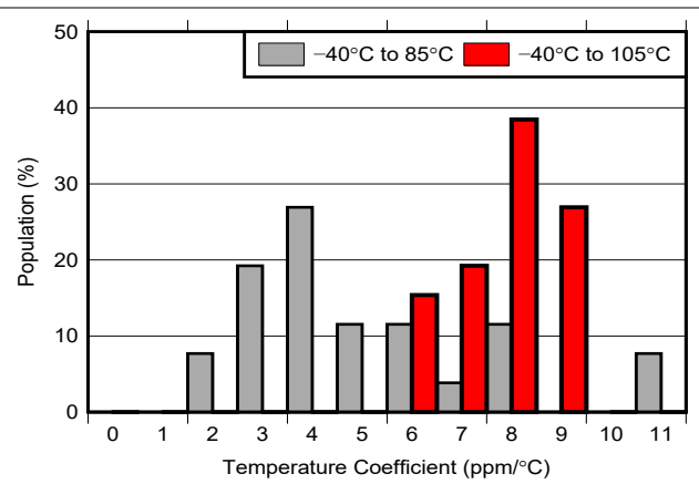
图 6-2. Temperature Coefficient Distribution ( V_{REF} = 1.25\text{V} )
