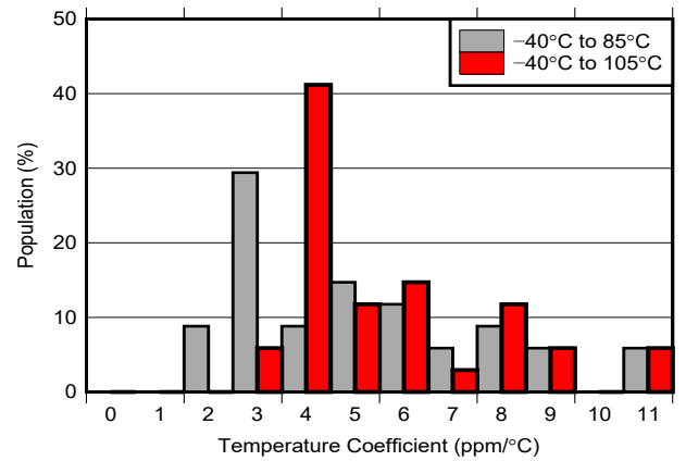
图 6-4. Temperature Coefficient Distribution ( V_{REF} = 5.0\text{V} )
