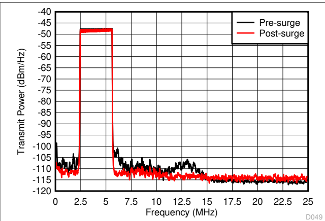
图 7-9. China SGCC HPLC Band1 Pre-Surge and Post-Surge
