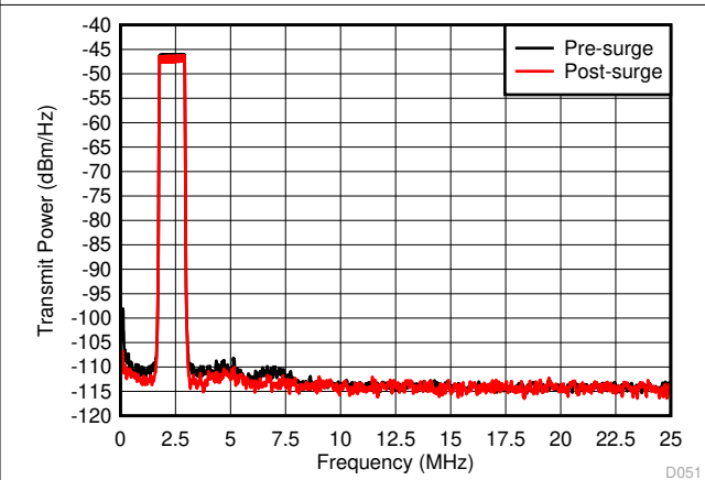
图 7-11. China SGCC HPLC Band3 Pre-Surge and Post-Surge
