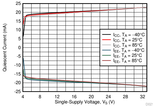
图 6-31. Quiescent Current vs Single-Supply Voltage
