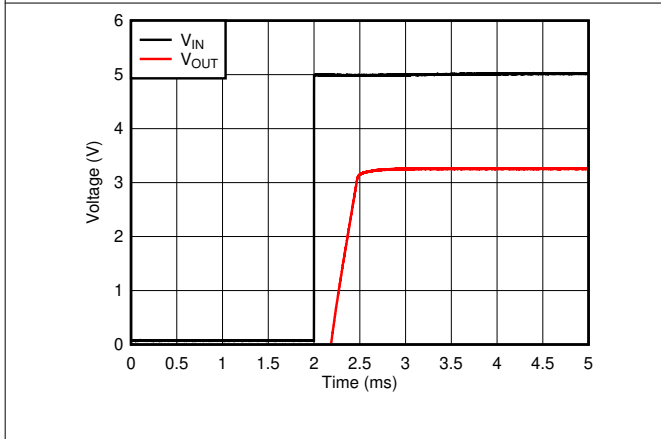
图 5-9. V_{IN} = V_{EN} Power-Up
