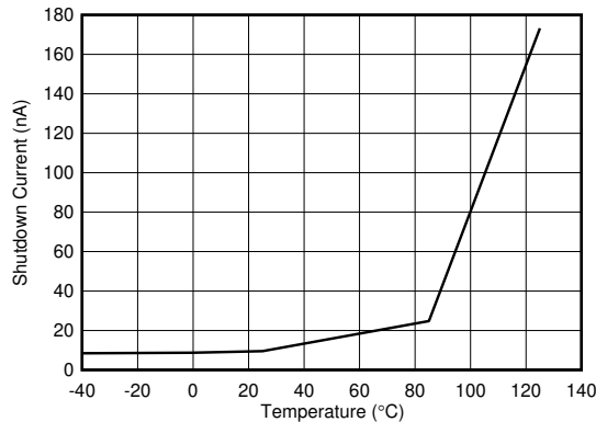
V_{EN} = 0\text{V}
