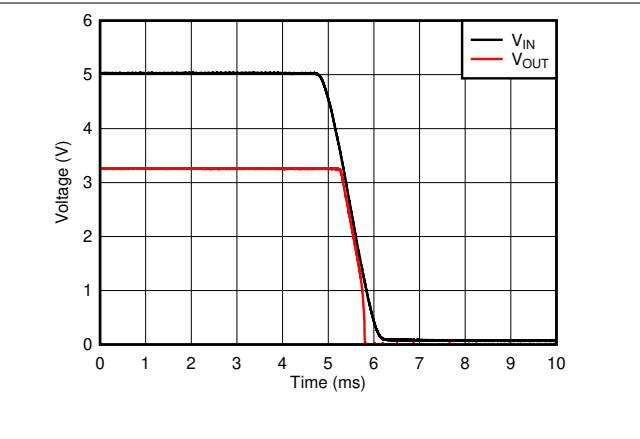
图 5-10. V_{IN} = V_{EN} Shutdown
