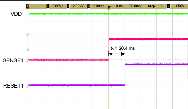
V_{\text{SENSE1}} start up 0 V to 3.3 V, V_{\text{DD}} = 3.3 V, V_{\text{RESET1}} = 3.3 V, TPS37044A7OHDDFRQ1
