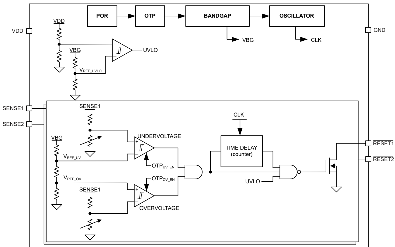
图 7-2. TPS37042-Q1 Dual-Channel Functional Block Diagram
