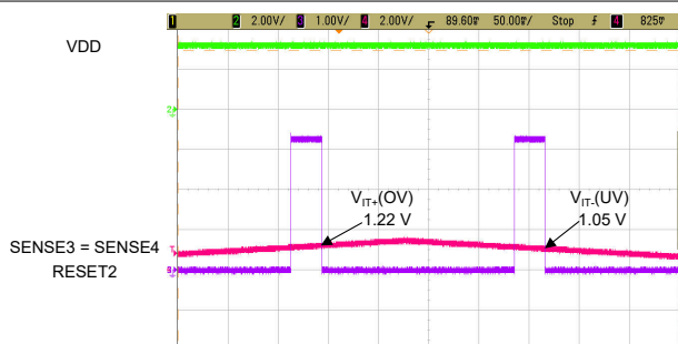
V_{\text{SENSE3\_4}} ramp 0 V to 1.5 V, OV/UV Threshold = 1.15 V (+7.5%, -5.5%), V_{\text{DD}} = 3.3 V, V_{\text{RESET2}} = 3.3 V, TPS37044A7OHDDFRQ1
