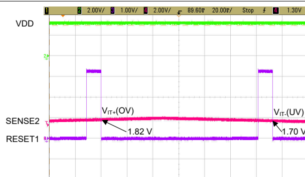
V_{\text{SENSE2}} ramp 0 V to 2 V, OV/UV Threshold = 1.8 V (+4%, -3.5%), V_{\text{SENSE1}} = 3.3 V, V_{\text{DD}} = 3.3 V, V_{\text{RESET1}} = 3.3 V, TPS37044A7OHDDFRQ1
