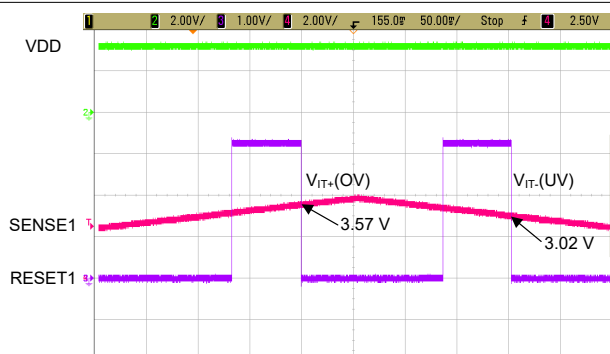
V_{\text{SENSE1}} ramp 0 V to 3.75 V, OV/UV Threshold = 3.3 V ( \pm 8\% ), V_{\text{SENSE2}} = 1.8 V, V_{\text{DD}} = 3.3 V, V_{\text{RESET1}} = 3.3 V, TPS37044A7OHDDFRQ1
