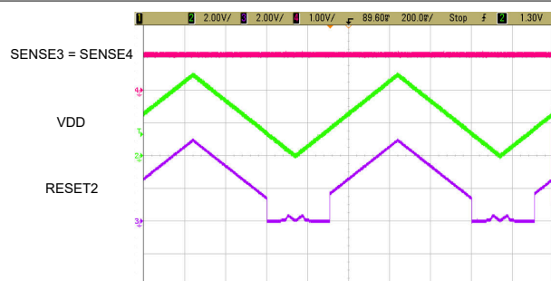
V_{\text{DD}} ramp 0 V to 5 V, V_{\text{SENSE3\_4}} = 1.2 V, V_{\text{RESET2}} = 3.3 V, TPS37044A7OHDDFRQ1
