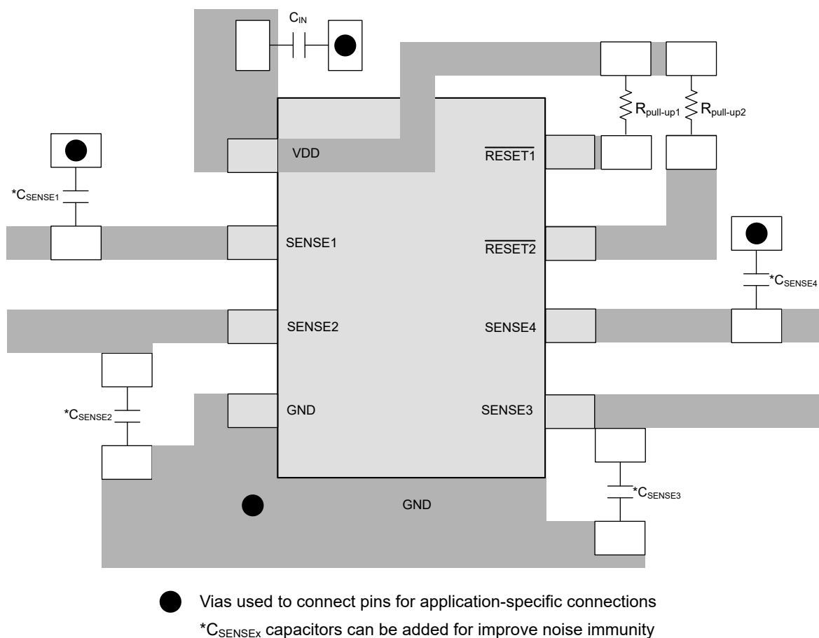
图 8-15. Recommended Layout
