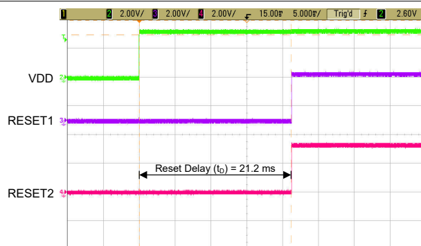
V_{\text{DD}} start up 0 V to 3.3 V, V_{\text{SENSE1}} = 3.3 V, V_{\text{SENSE2}} = 1.8 V, V_{\text{SENSE3\_4}} = 1.15 V, V_{\text{RESET1\_2}} = 3.3 V, TPS37044A7OHDDFRQ1
