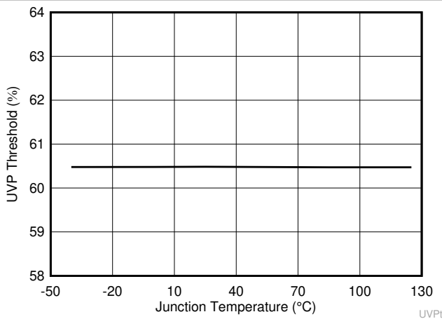
图 6-9. UVP Threshold vs Junction Temperature UVPT
