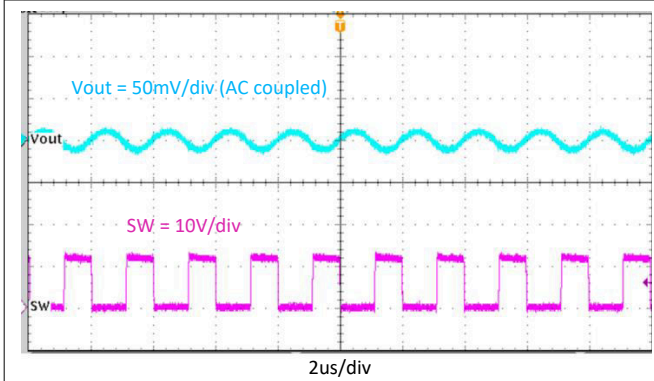
图 8-14. Output Voltage Ripple, I_{OUT} = 10\text{ A}
