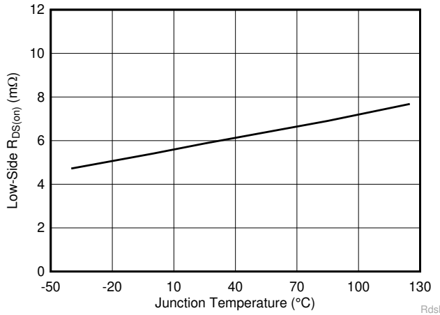
图 6-7. Low-Side R_{DS(on)} vs Junction Temperature RdSl
