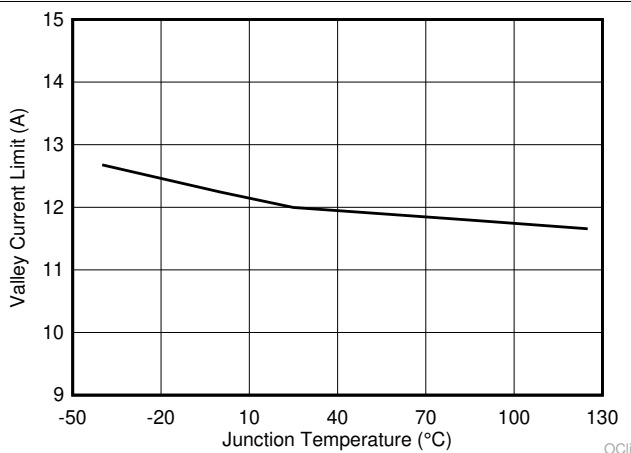
图 6-11. Valley Current Limit vs Junction Temperature OCi
