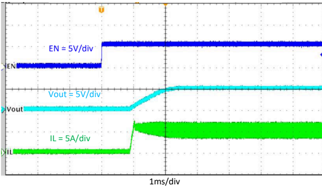
图 8-8. Start-Up Through EN, I_{OUT} = 5\text{ A}
