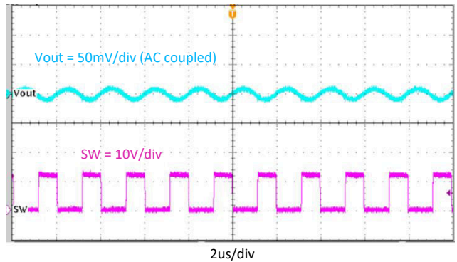
图 8-13. Output Voltage Ripple, I_{OUT} = 5\text{ A}
