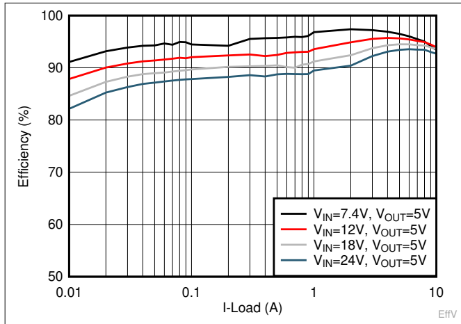
图 8-2. Efficiency Curve
