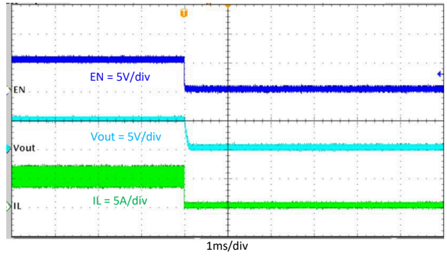
图 8-9. Shut-down Through EN, I_{OUT} = 5\text{ A}
