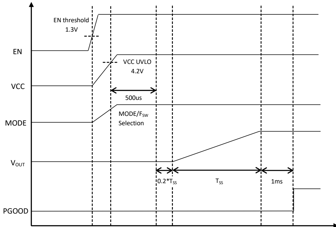
图 7-1. Power-Up Sequence
