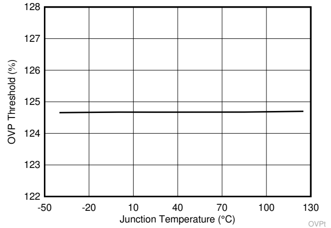
图 6-8. OVP Threshold vs Junction Temperature OVPT
