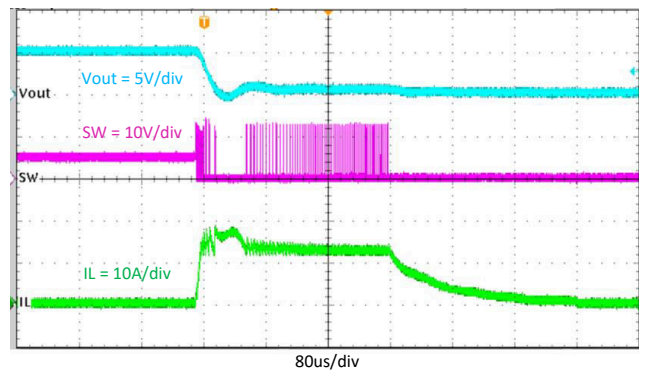
图 8-17. Normal Operation to Output Hard Short
