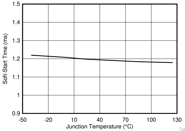
图 6-13. Soft-Start Time vs Junction Temperature
