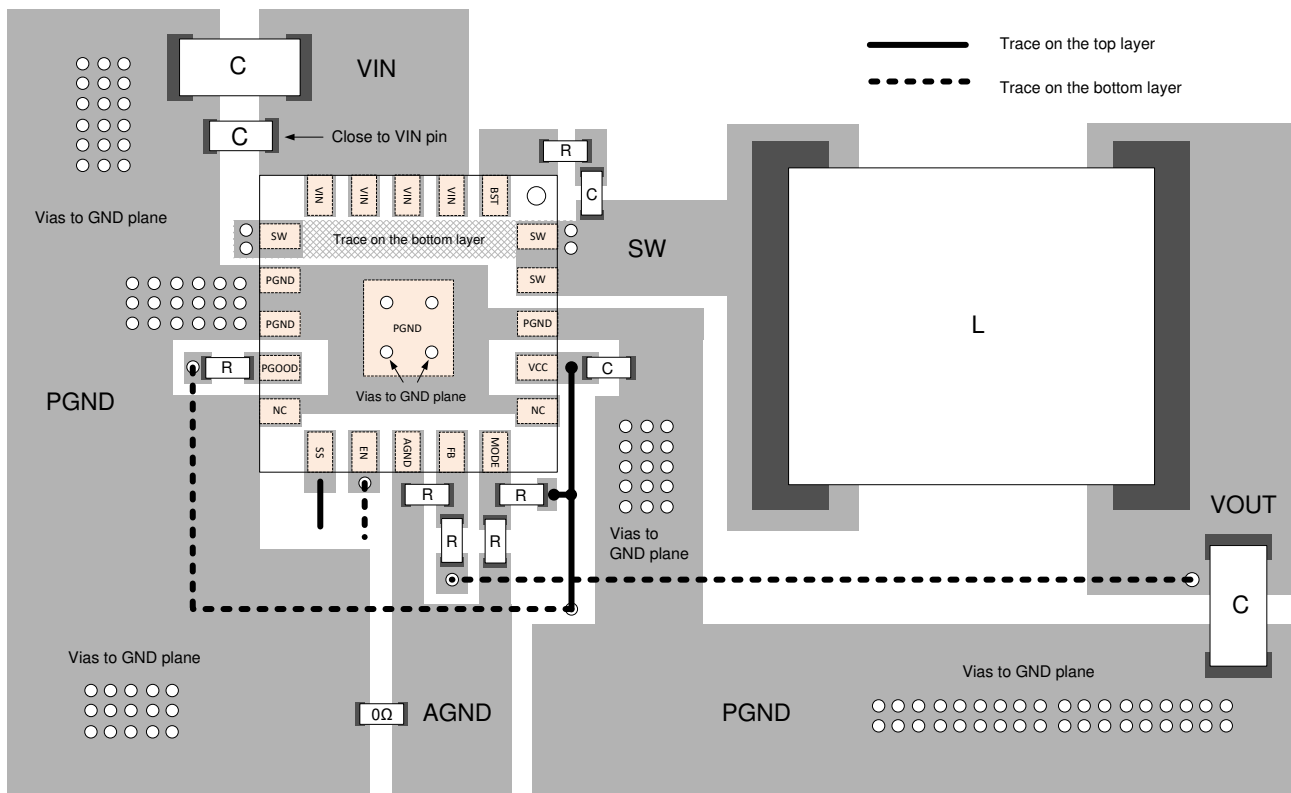
图 10-1. Top-Side Layout
