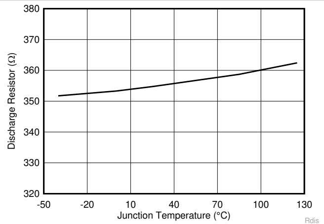
图 6-10. Discharge Resistor vs Junction Temperature Rdis
