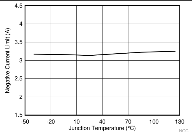
图 6-12. Negative Current Limit vs Junction Temperature NOC
