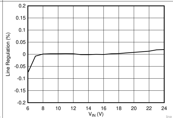
图 8-7. Line Regulation, I_{OUT} = 5\text{ A}
