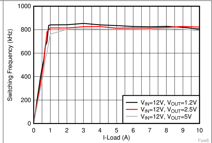
图 6-20. Switching Frequency vs Load Current, F_{sw} = 800 \text{ kHz} , Eco-mode
