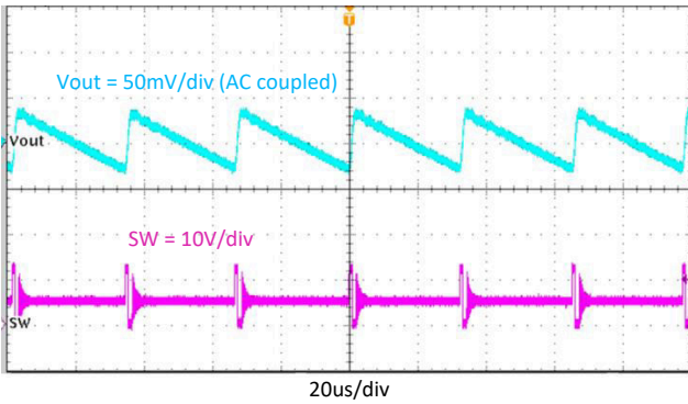
图 8-12. Output Voltage Ripple, I_{OUT} = 0.1\text{ A}
