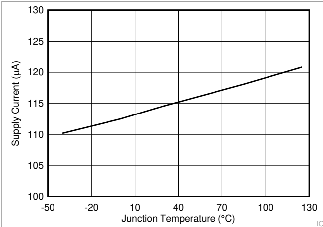
图 6-1. Supply Current vs Junction Temperature
