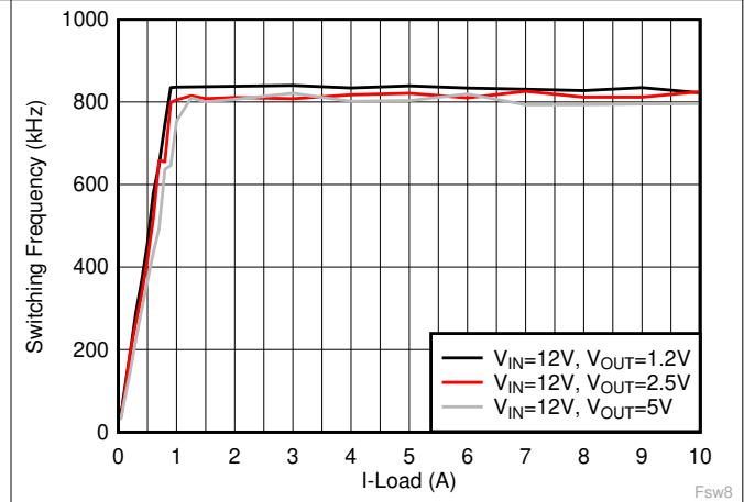
图 6-22. Switching Frequency vs Load Current, F_{sw} = 800 \text{ kHz} , OOA
