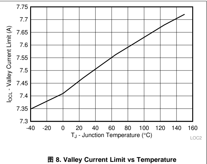
图 8. Valley Current Limit vs Temperature
