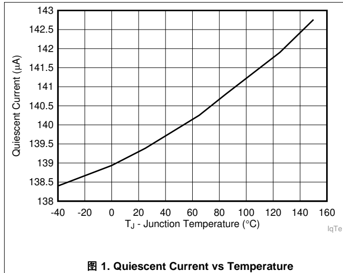
图 1. Quiescent Current vs Temperature
