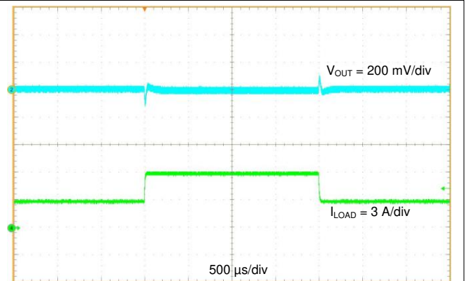
图 27. Transient Response 0 to 6 A
