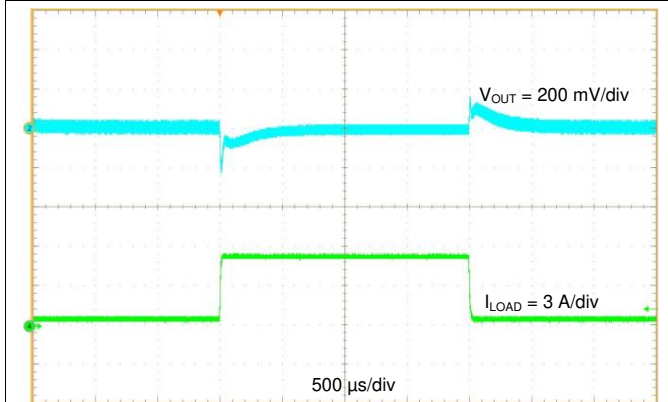
图 26. Transient Response 0 to 3 A
