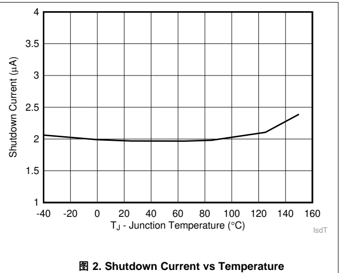
图 2. Shutdown Current vs Temperature
