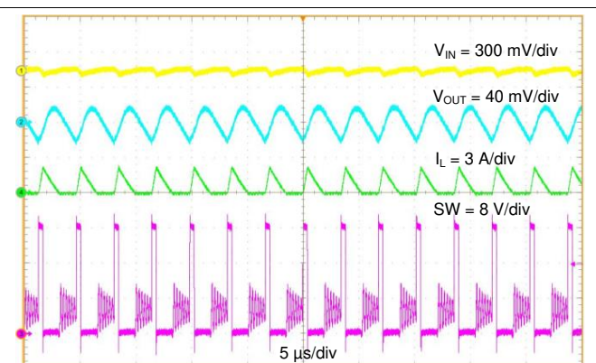
图 23. Steady State Waveforms, I_{OUT} = 0.6 A
