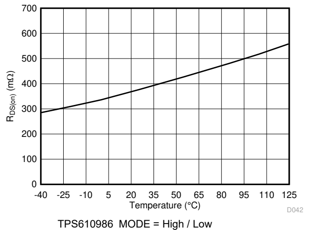
图 7-16. Low Side Switch on Resistance vs Temperature
