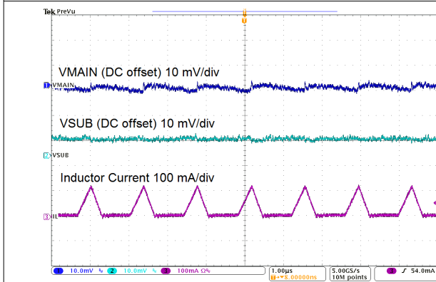
图 9-5. Switching Waveforms
