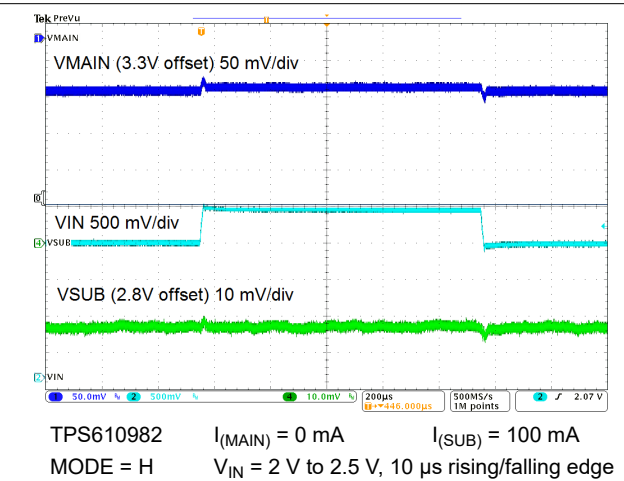
图 9-33. Line Transient Response
