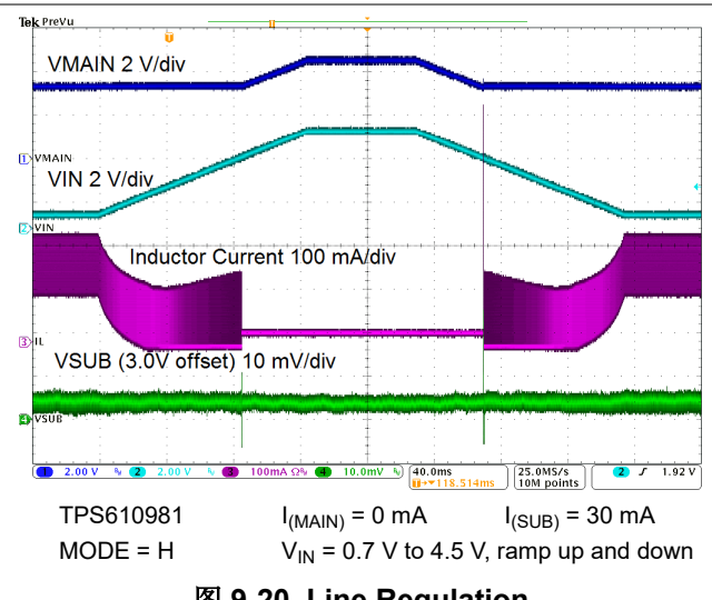
图 9-20. Line Regulation
