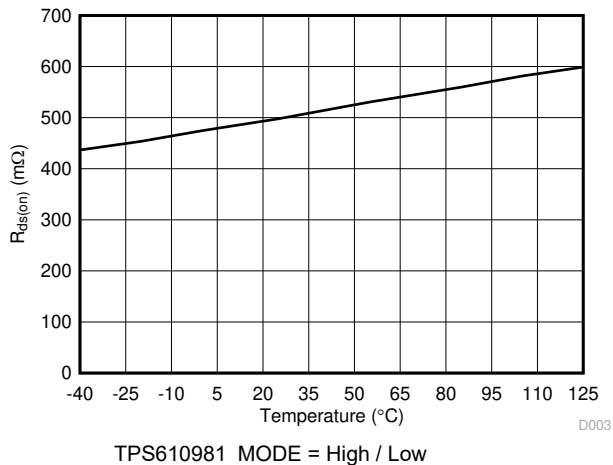
图 7-9. Rectifier On Resistance vs Temperature
