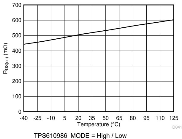
图 7-15. Rectifier on Resistance vs Temperature
