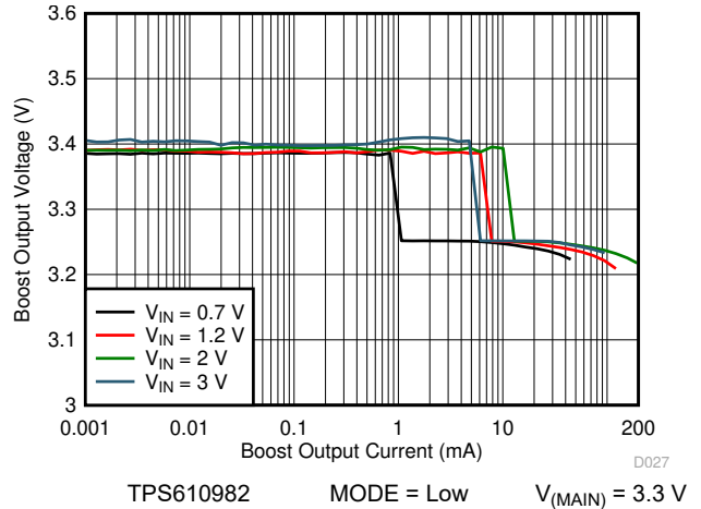
图 7-32. Boost Load Regulation (Low Power Mode)
