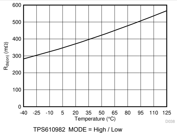
图 7-12. Low Side Switch On Resistance vs Temperature
