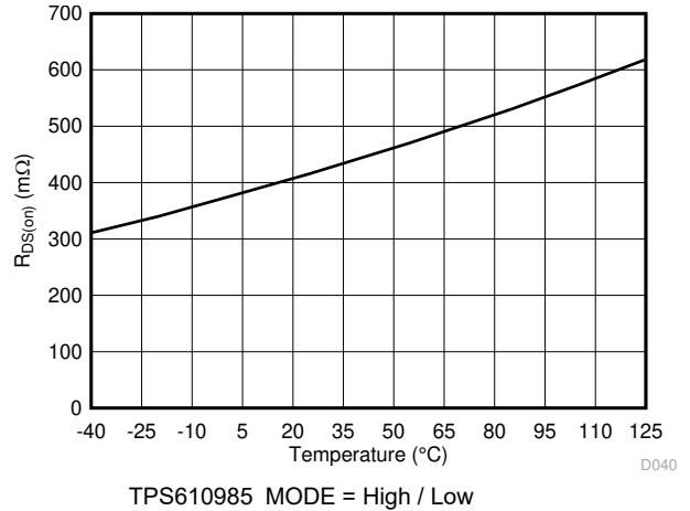
图 7-14. Low Side Switch On Resistance vs Temperature
