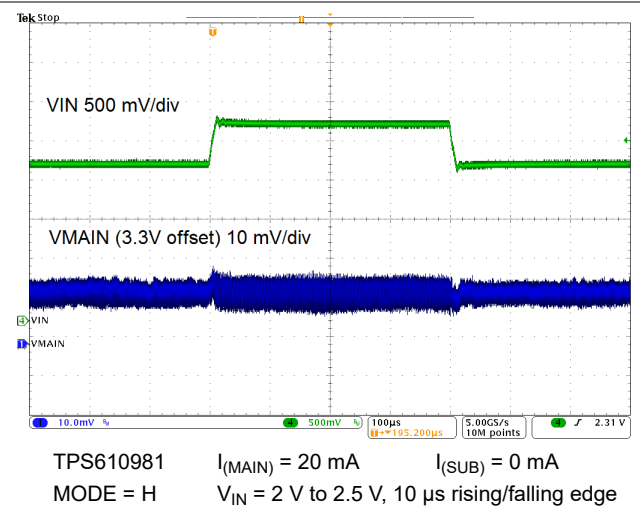
图 9-16. Line Transient Response
