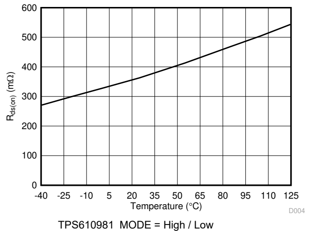
图 7-10. Low Side Switch On Resistance vs Temperature
