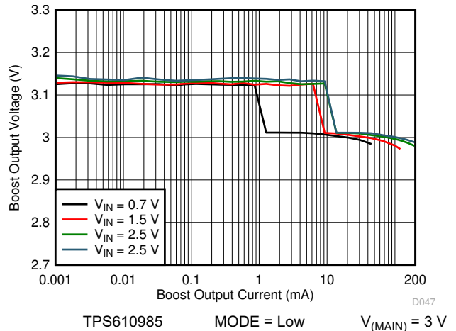
图 7-34. Boost Load Regulation (Low Power Mode)
