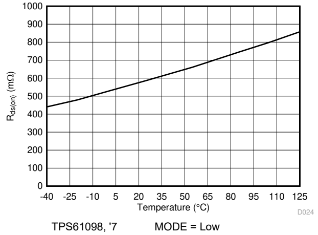
图 7-8. Low Side Switch On Resistance vs Temperature
