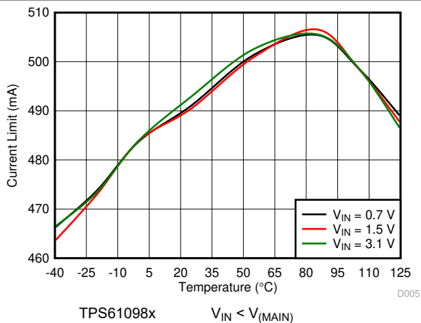
图 7-17. Current Limit vs Temperature
