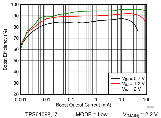
图 7-18. Boost Efficiency vs Output Current (Low Power Mode)
