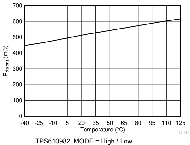
图 7-11. Rectifier On Resistance vs Temperature
