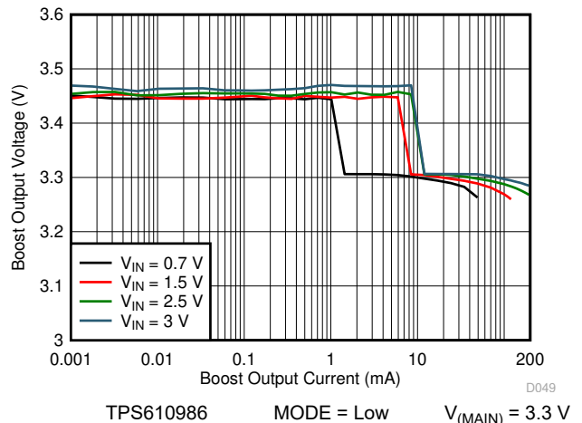
图 7-36. Boost Load Regulation (Low Power Mode)
