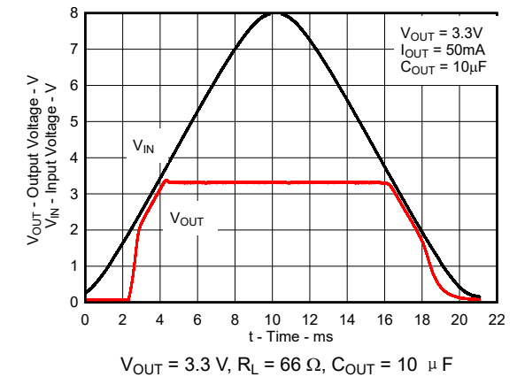
图 6-18. Power-Up and Power-Down for New Chip
