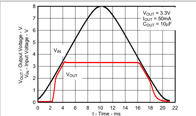
图 8-6. TPS71533-Q1 Power-Up and Power-Down Waveform for New Chip
