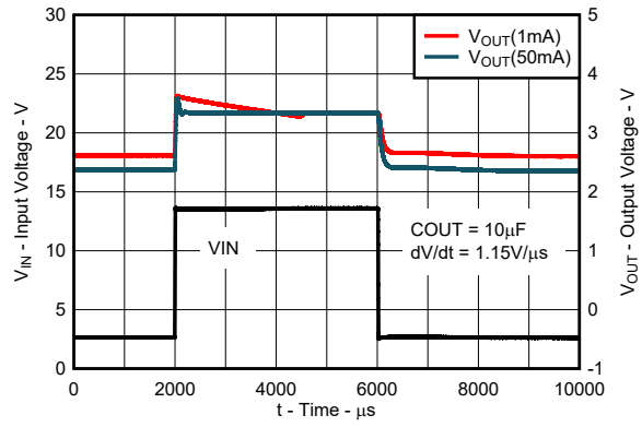
8-10. TPS71533-Q1 Dropout Exit Transient Response for New Chip
