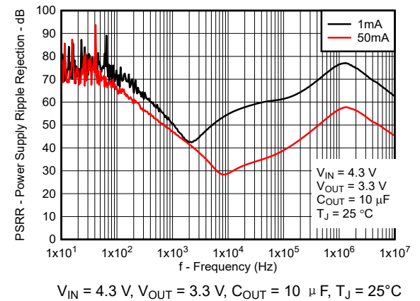
图 6-16. Power-Supply Ripple Rejection vs Frequency for New Chip
