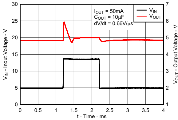
8-9. TPS71533-Q1 Fast Line Transient Waveform for New Chip
