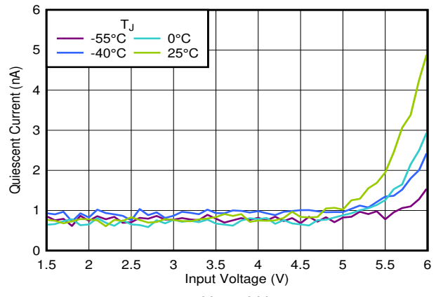
图 6-10. I_{SHDN} vs V_{IN} and Temperature
