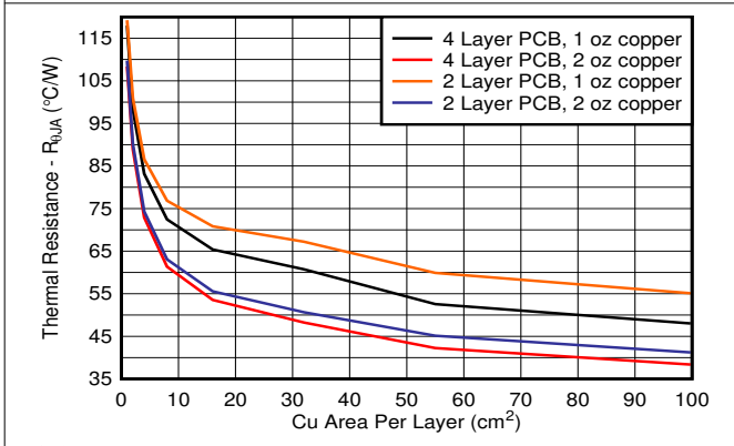
8-4. R_{\theta JA} vs Copper Area 2s2p DCY Package
