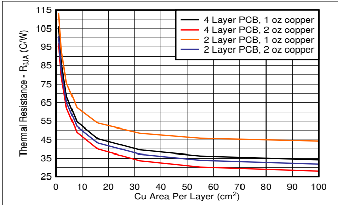
8-2. R_{\theta JA} vs Copper Area 2s2p DRB Package
