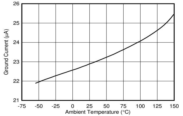
I_{OUT} = 500\ \mu\text{A} 图 6-26. Ground Current
