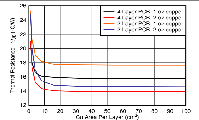
8-3. \Psi_{JB} vs Copper Area 2s2p DRB Package
