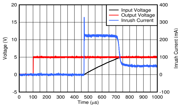
V_{IN} = 13.5\ \text{V} , C_{OUT} = 10\ \mu\text{F} 图 6-29. Startup Plot With EN
