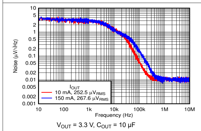
图 6-11. Noise vs Frequency at 3.3 V
