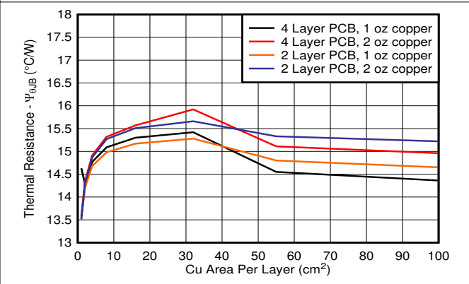
8-5. \Psi_{JB} vs Copper Area 2s2p DCY Package
