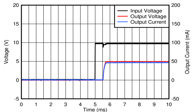
C_{OUT} = 10\ \mu\text{F} 图 6-30. Startup Plot
