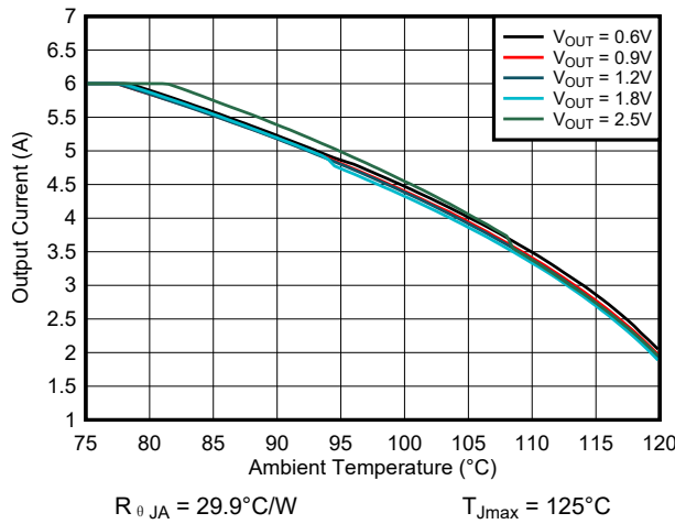
图 8-38. Safe Operating Area V_{IN} = 3.3\text{-V} TPSM82866AA0PRCFR
