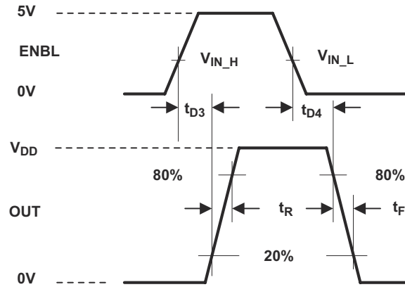
图 7-2. Switching Waveform for Enable to Output
