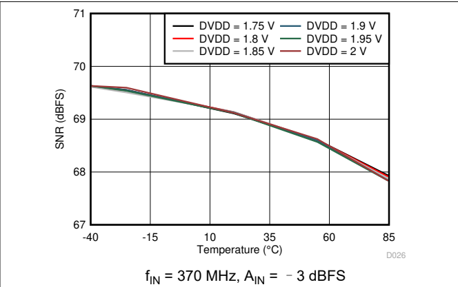
图 6-28. Signal-to-Noise Ratio vs DVDD Supply and Temperature
