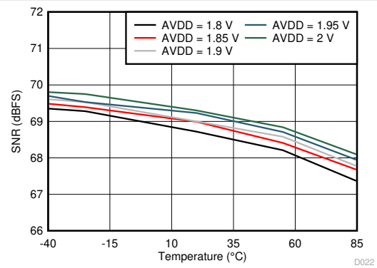
图 6-22. Signal-to-Noise Ratio vs AVDD Supply and Temperature
