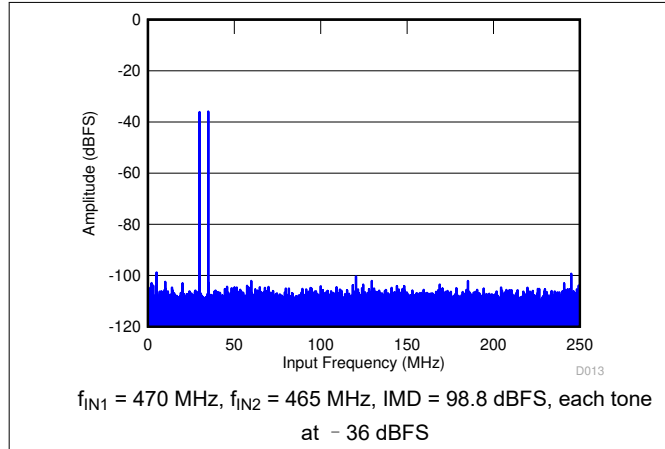
图 6-15. FFT for Two-Tone Input Signal
