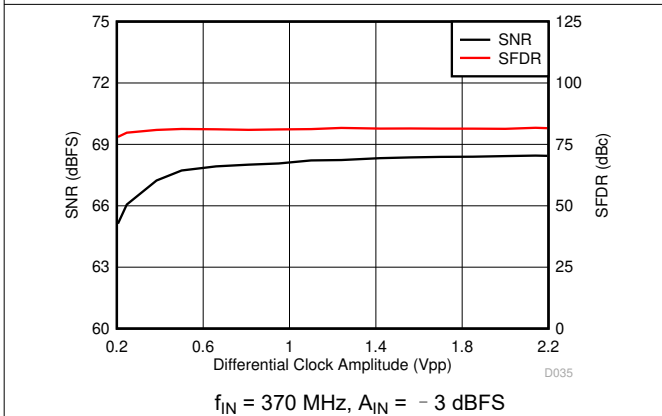
图 6-37. Performance vs Clock Amplitude
