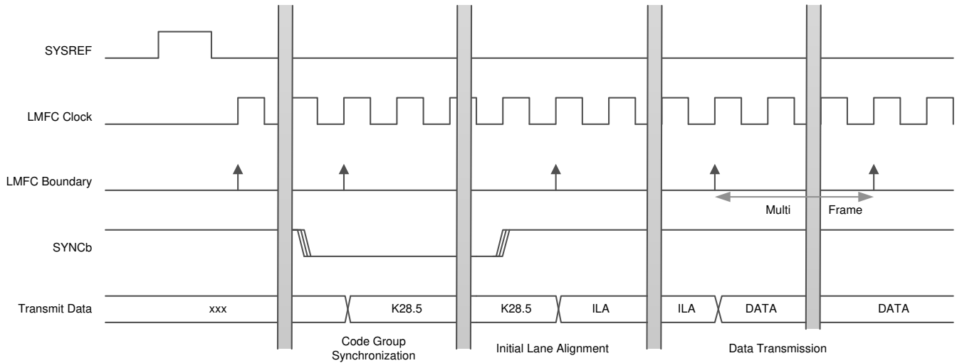
图 7-27. ILA Sequence
