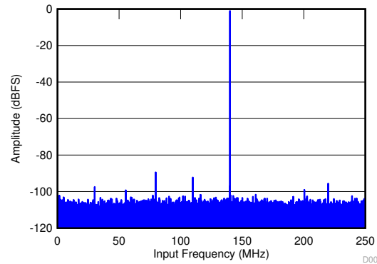
f_{\text{IN}} = 140\text{ MHz} , A_{\text{IN}} = -1\text{ dBFS} , \text{SNR} = 70\text{ dBFS} , \text{SFDR} = 88\text{ dBc} , \text{SFDR} = 91\text{ dBc} (non 23)
