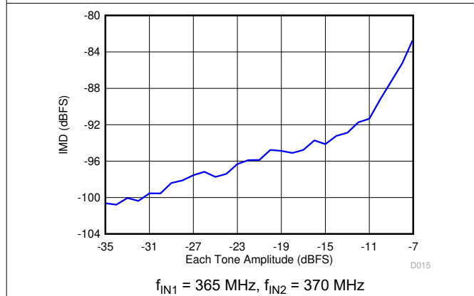
图 6-17. Intermodulation Distortion vs Input Amplitude
