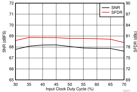
图 6-39. Performance vs Clock Duty Cycle
