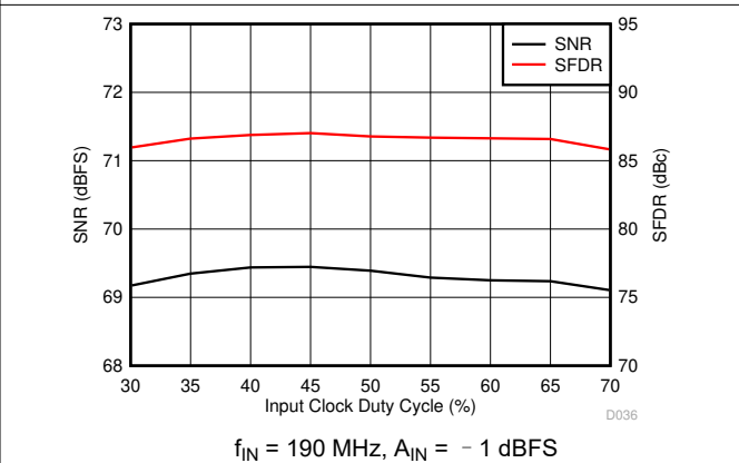
图 6-38. Performance vs Clock Duty Cycle
