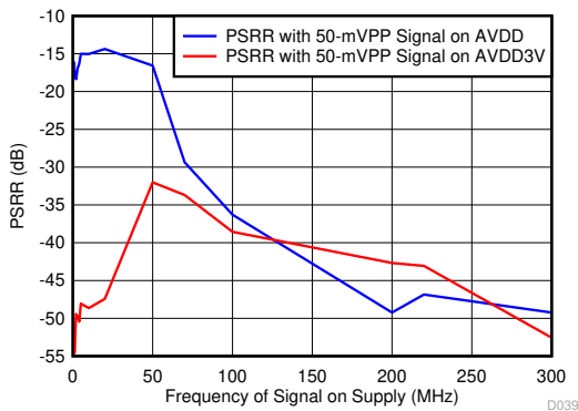
图 6-41. Power-Supply Rejection Ratio vs Supplies
