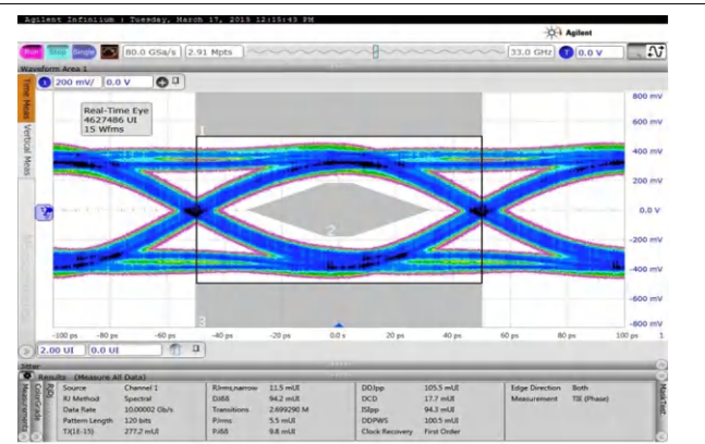
图 7-33. Eye at 10-Gbps Bit Rate with Increased Output Swing
