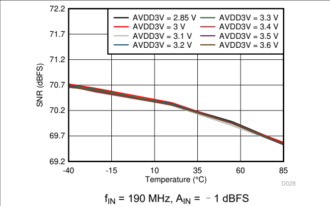
图 6-30. Signal-to-Noise Ratio vs AVDD3V Supply and Temperature
