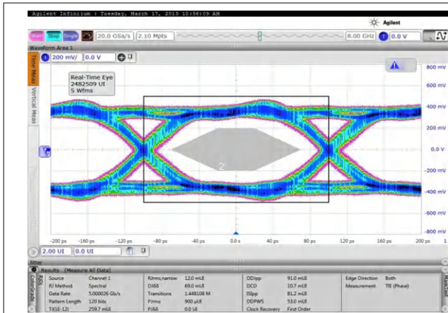
图 7-30. Eye at 5-Gbps Bit Rate with Default Output Swing
