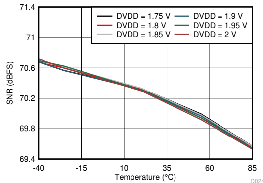
图 6-26. Signal-to-Noise Ratio vs DVDD Supply and Temperature
