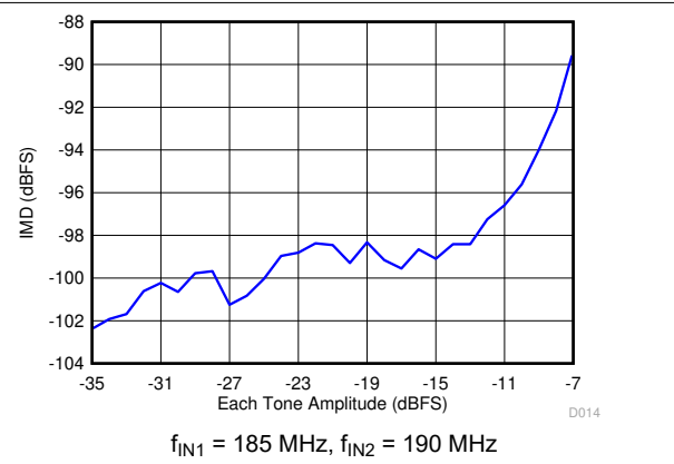
图 6-16. Intermodulation Distortion vs Input Amplitude
