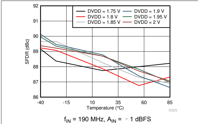
图 6-27. Spurious-Free Dynamic Range vs DVDD Supply and Temperature
