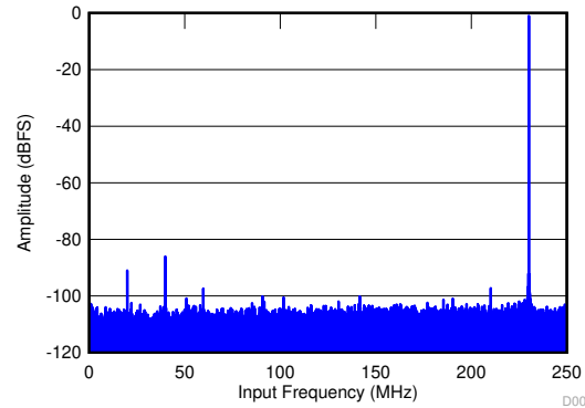
f_{\text{IN}} = 230\text{ MHz} , A_{\text{IN}} = -1\text{ dBFS} , \text{SNR} = 69.4\text{ dBFS} , \text{SFDR} = 85\text{ dBc} , \text{SFDR} = 96\text{ dBc} (non 23)
