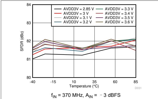
图 6-33. Spurious-Free Dynamic Range vs AVDD3V Supply and Temperature
