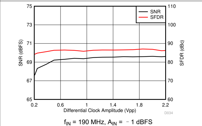
图 6-36. Performance vs Clock Amplitude
