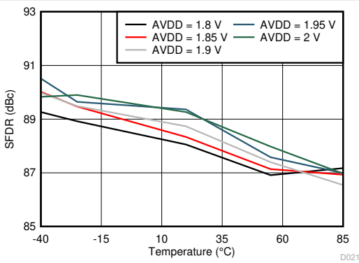
图 6-23. Spurious-Free Dynamic Range vs AVDD Supply and Temperature
