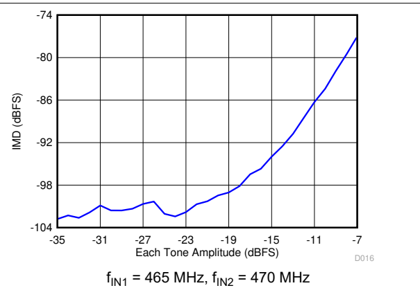
图 6-18. Intermodulation Distortion vs Input Amplitude
