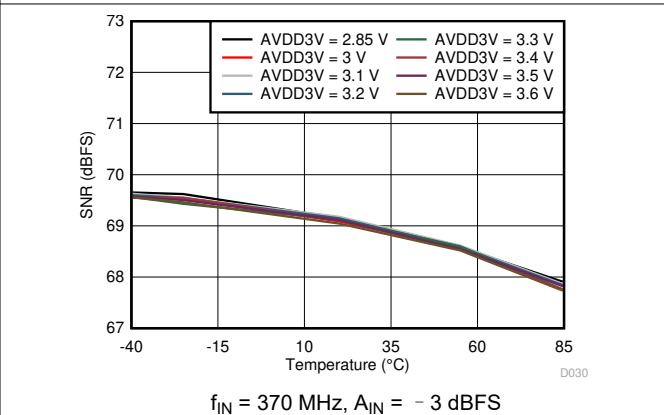
图 6-32. Signal-to-Noise Ratio vs AVDD3V Supply and Temperature
