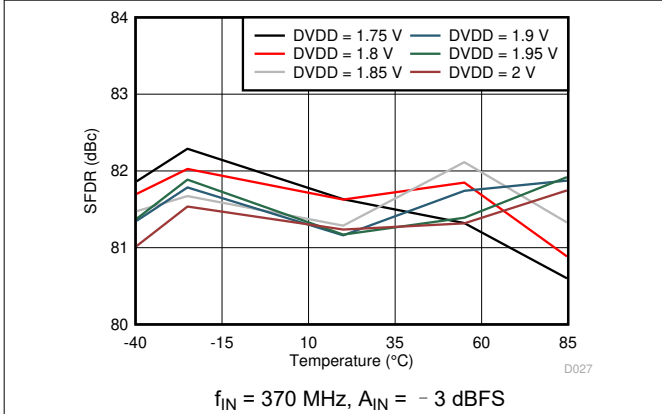
图 6-29. Spurious-Free Dynamic Range vs DVDD Supply and Temperature
