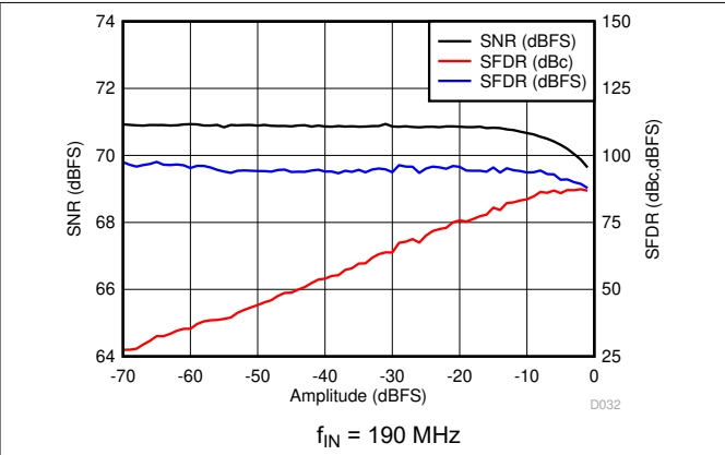
图 6-34. Performance vs Amplitude
