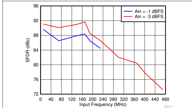
图 6-19. Spurious-Free Dynamic Range vs Input Frequency
