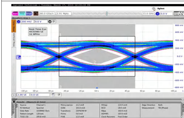
图 7-32. Eye at 10-Gbps Bit Rate with Default Output Swing
