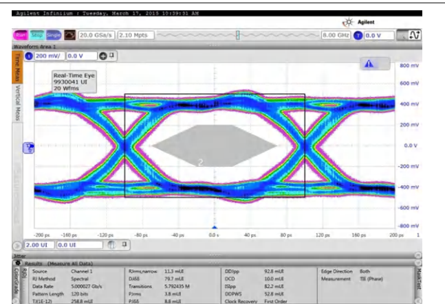
图 7-31. Eye at 5-Gbps Bit Rate with Increased Output Swing
