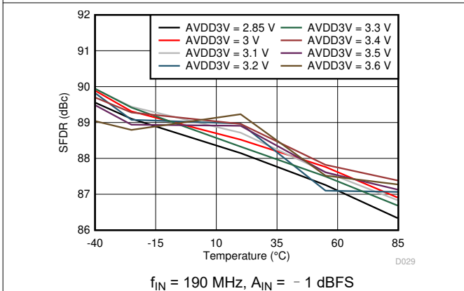
图 6-31. Spurious-Free Dynamic Range vs AVDD3V Supply and Temperature
