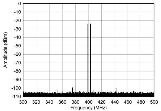
图 5-263. Dual Tone Spectrum at 400 MHz and -30 dBFS ( \pm 100 MHz)
