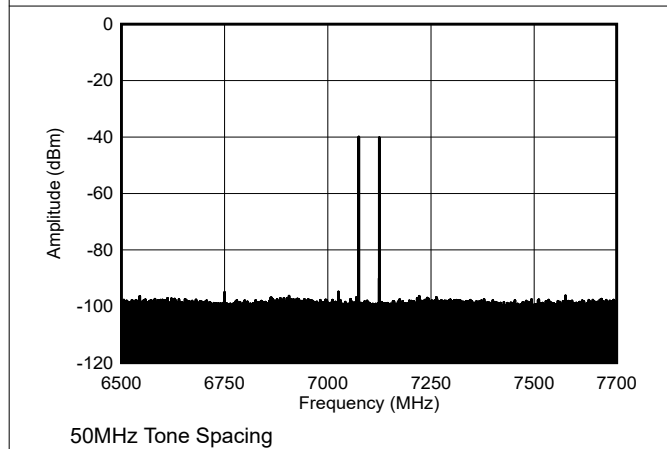
图 5-566. Two Tone Output Spectrum at 7.1GHz, -30dBFS each (Inband)
