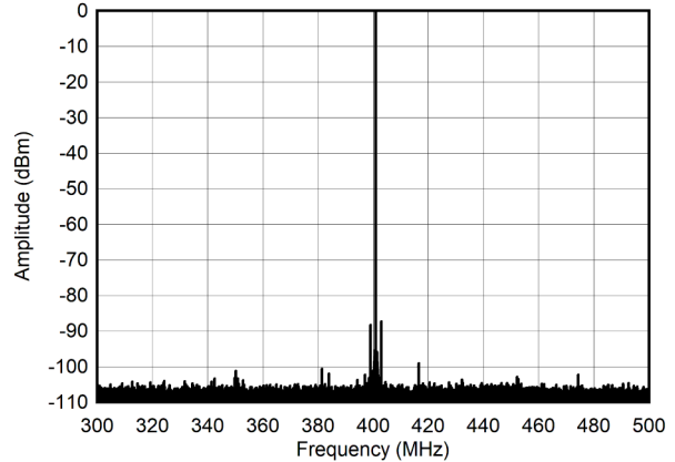
图 5-251. Single Tone Spectrum at 400 MHz and -6 dBFS ( \pm 100\text{MHz} )
