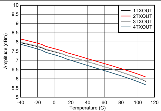
图 5-203. TX Output Fullscale vs Temperature at 30 MHz
