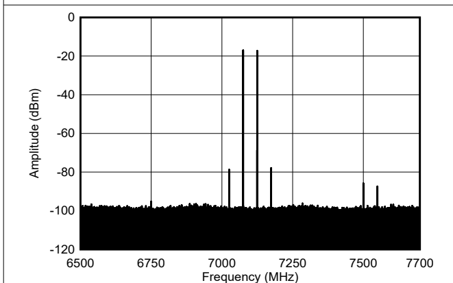
图 5-562. Two Tone Output Spectrum at 7.1GHz, -7dBFS each (Inband)
