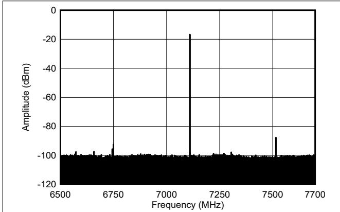
图 5-558. Single Tone Output Spectrum at 7.1GHz, -6dBFS (Inband)
