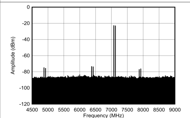
图 5-561. Two Tone Output Spectrum at 7.1GHz, -7dBFS each (Nyquist)
