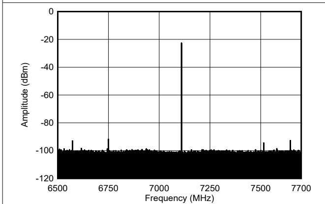
图 5-560. Single Tone Output Spectrum at 7.1GHz, -12dBFS (Inband)
