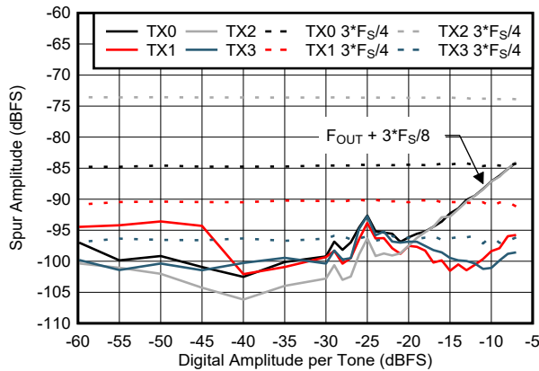
Inband = 7100MHz ± 600MHz, excluding IMD3 components, 3*Fs/4 spur not included and shown separately
