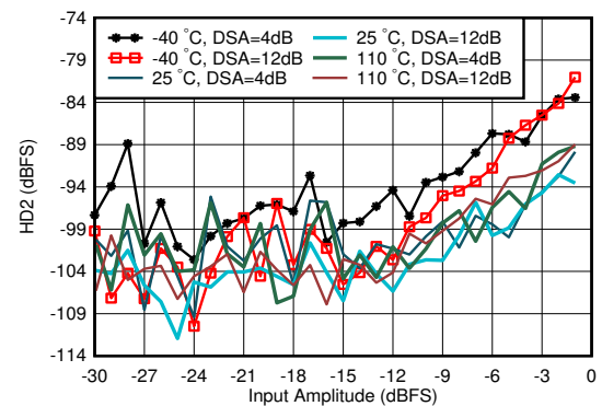
With 1.8 GHz matching, f_{\text{in}} = 1900\text{MHz} , measured after HD2 trim, DDC bypass mode (TI only mode for characterization)
