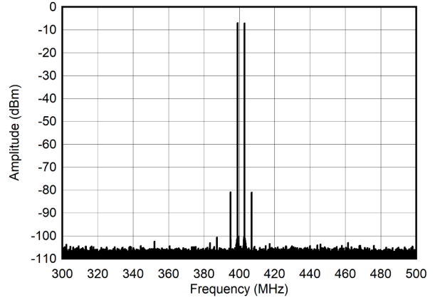
图 5-261. Dual Tone Spectrum at 400 MHz and -13 dBFS ( \pm 100 MHz)
